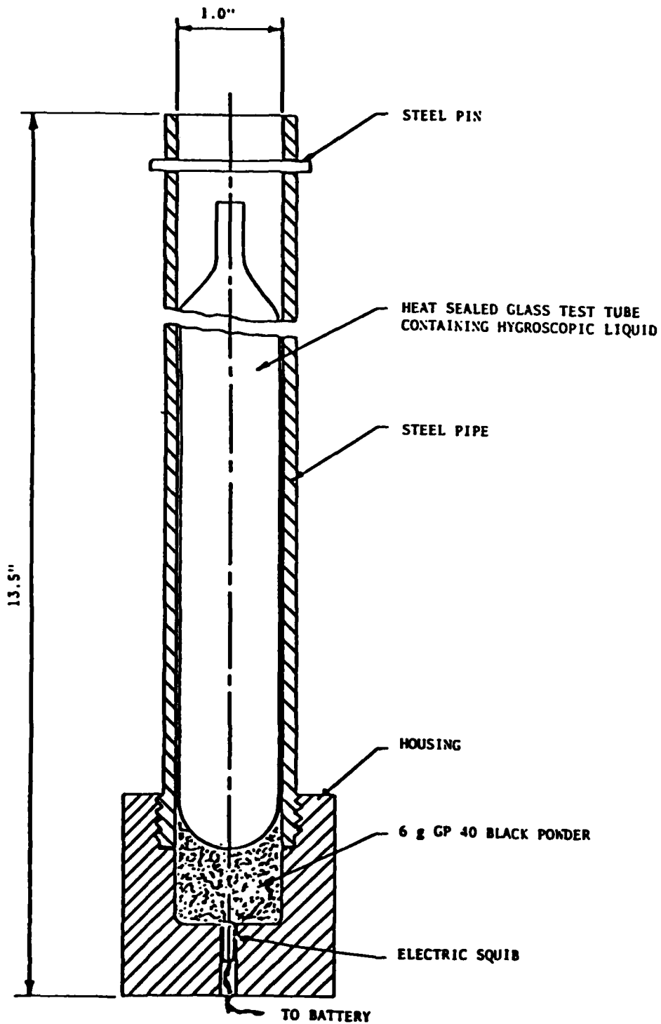
FIGURE C1 - Apparatus used to expel hygroscopic charges into the atmosphere
