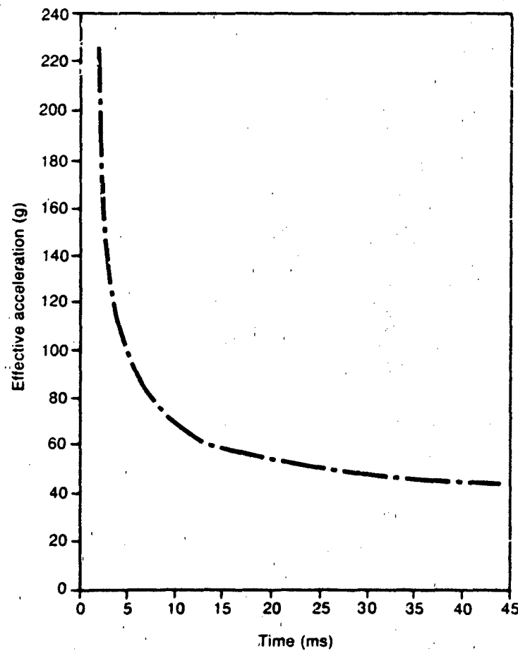
Figure 5.6-Wayne State University Cerebral Concussion Tolerance Curve
