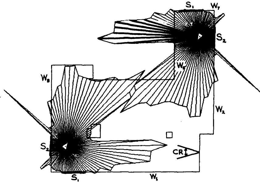
Figure 11: These are two feasible localizations based on the interpretations (S_1 W_1)(S_2 W_3) (lower left) and [(S_1 W_7)(S_2 W_2)] (upper right). Given the cone of reflection as shown, the upper right localization would fail the sonar barrier test because the heavy black segments apparently penetrate wall W_5 from inside the cone of reflection.
