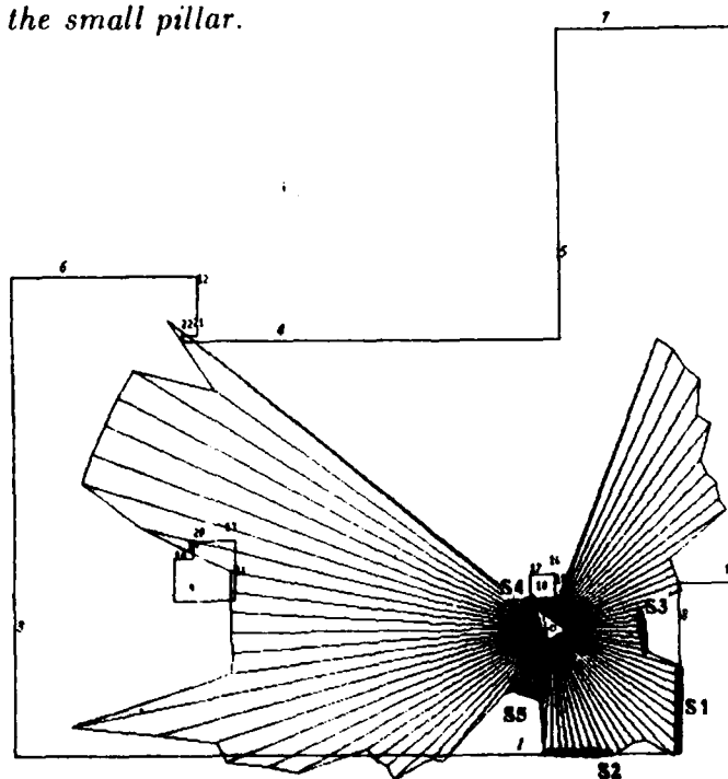
Figure 20: This sonar contour is similar to the contour in Figure 19, except for some deliberately introduced clutter ( S_3 and S_5 ). The clutter segments were successfully ignored.
