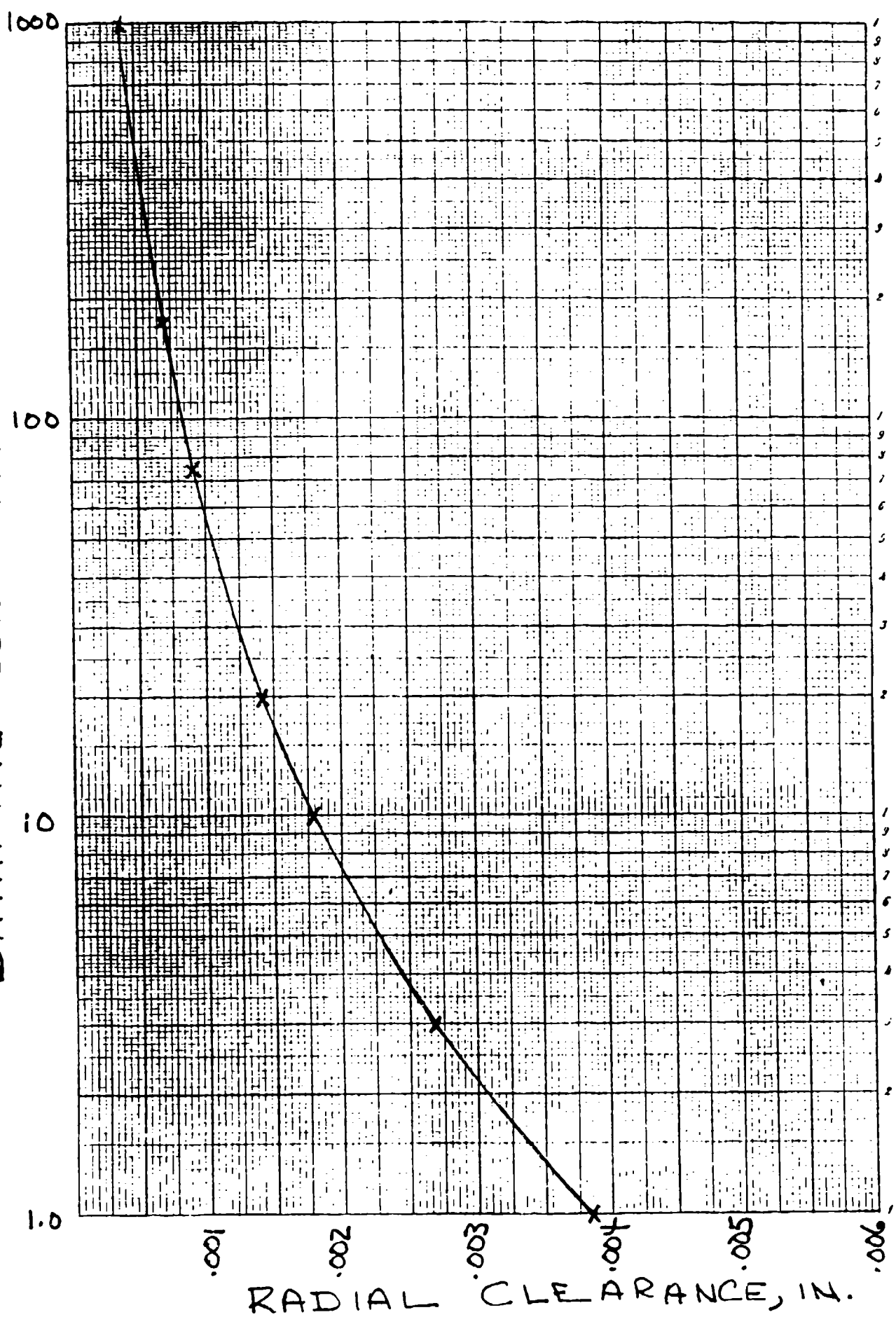
Figure 2.2.3-4 Damping Constant as a Function of Clearance
