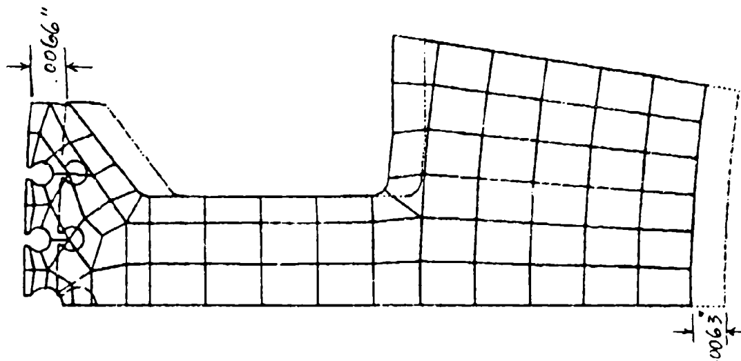
OF CONDITIONED SYSTEM ROTOR ASSEMBLY 2 SUPERB POST PLOT NO. 5 DISTORTED GEOMETRY 03/03/11
