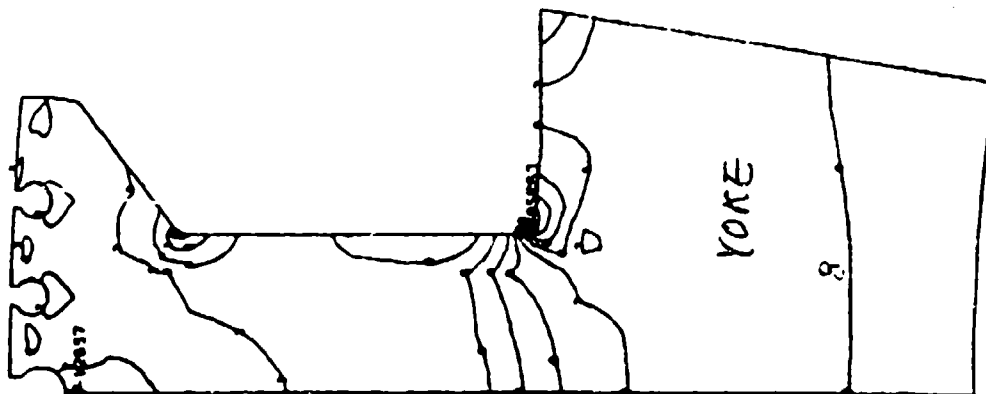
OF CONDITIONED SYSTEM ROTOR ASSEMBLY 2 SUPERB POST PLOT NO. 7 MAX PRINCIPAL STRESS 03/03/11
