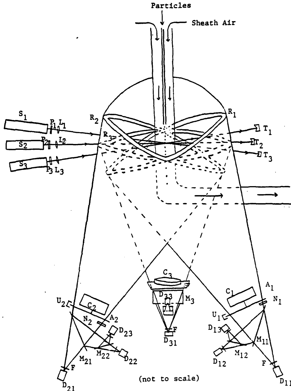
Figure 6 Optical System
