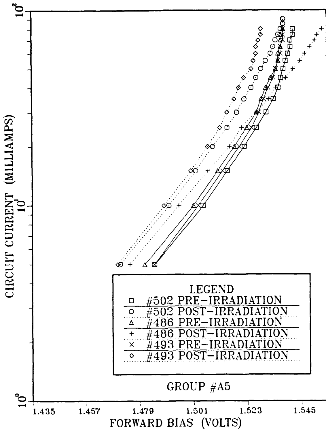
Figure 16. I-V Characteristics for 3 LEDs in Group A5 (expanded scale)
