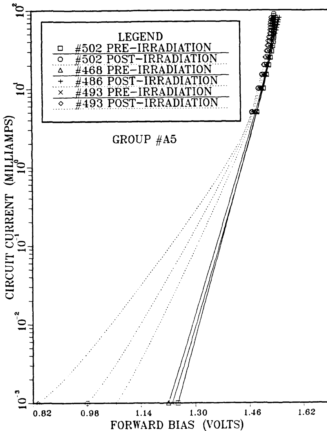
Figure 15. I-V Characteristics for 3 LEDs in Group A5 (— before irradiation, ... after)
