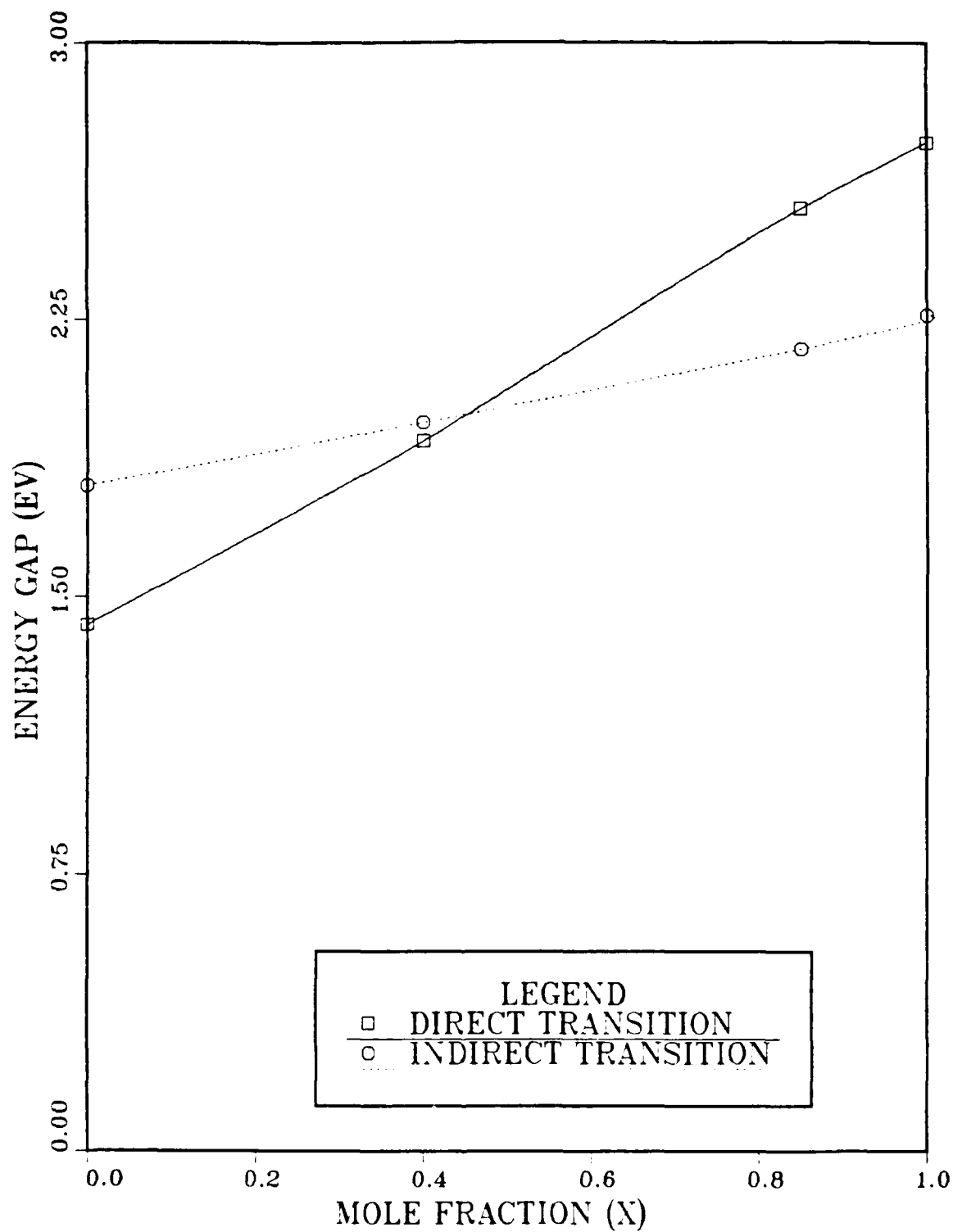
Figure 3. Compositional Dependencies for Direct and Indirect Band Gap Energies in GaAs 1-x P x
