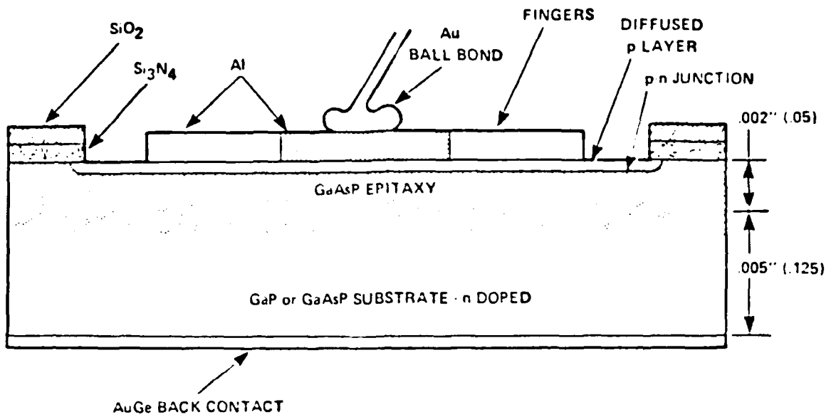
CROSS SECTION OF AN LED
