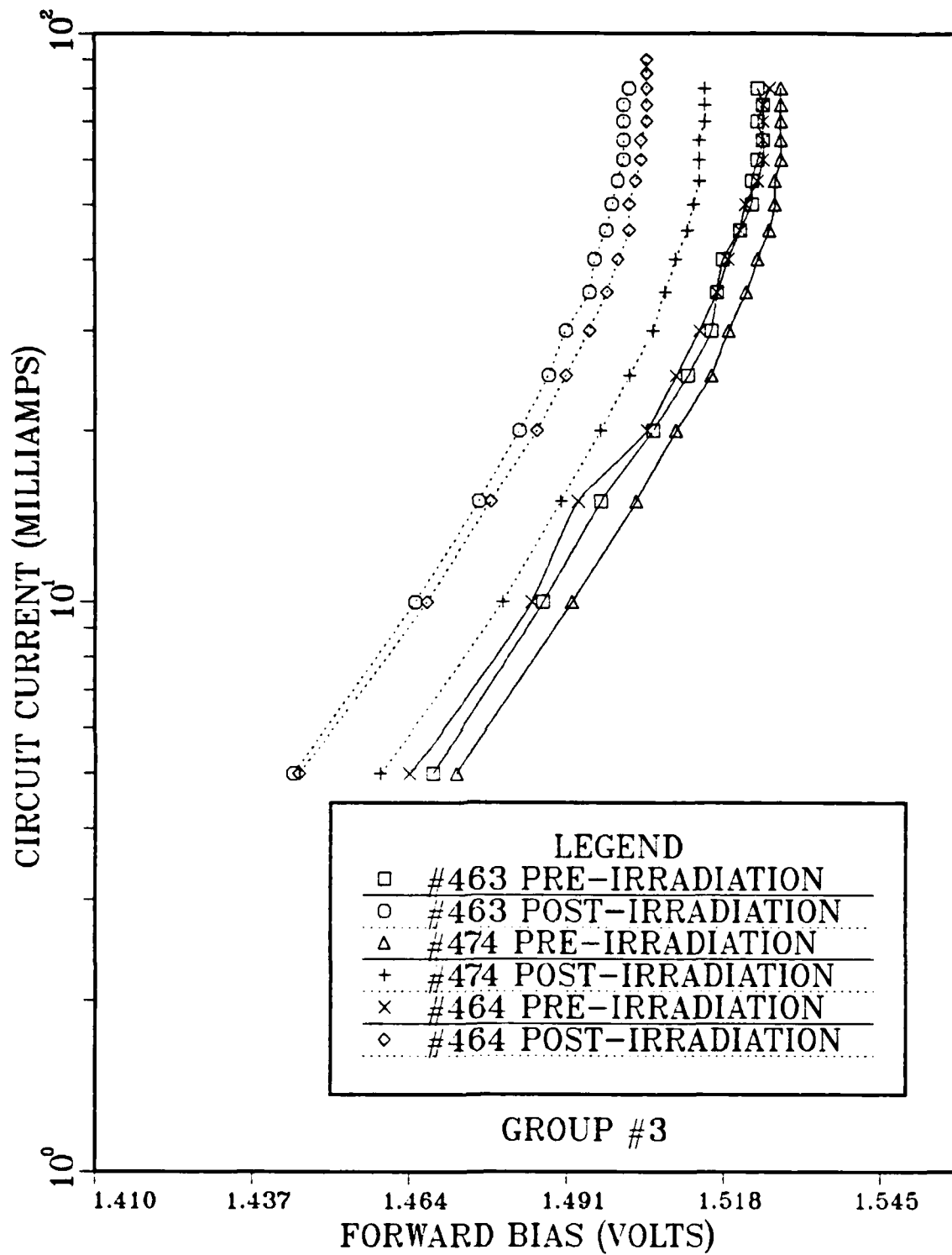
Figure 14. I-V Characteristics for 3 LEDs in Group 3 (expanded scale)
