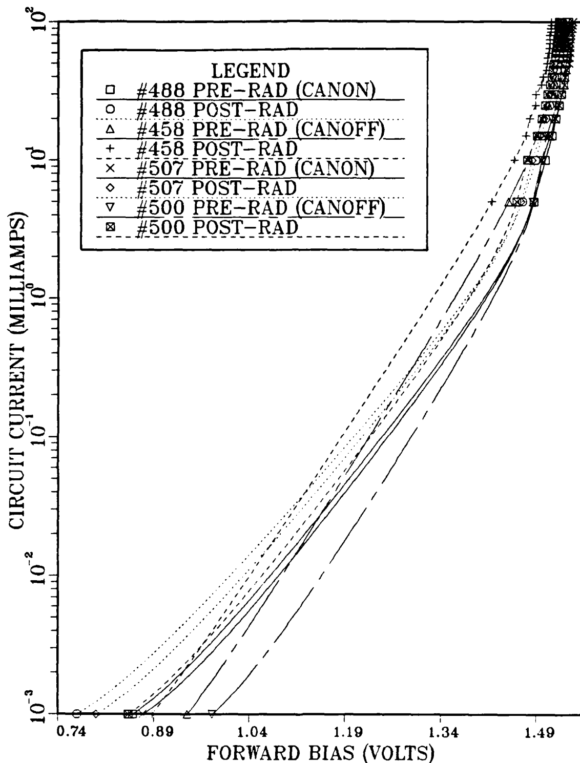
Figure 25. I-V Characteristics at 45° Offset (— before irradiation can-on, ... after can-on, --- before can-off, - - - after can-off)
