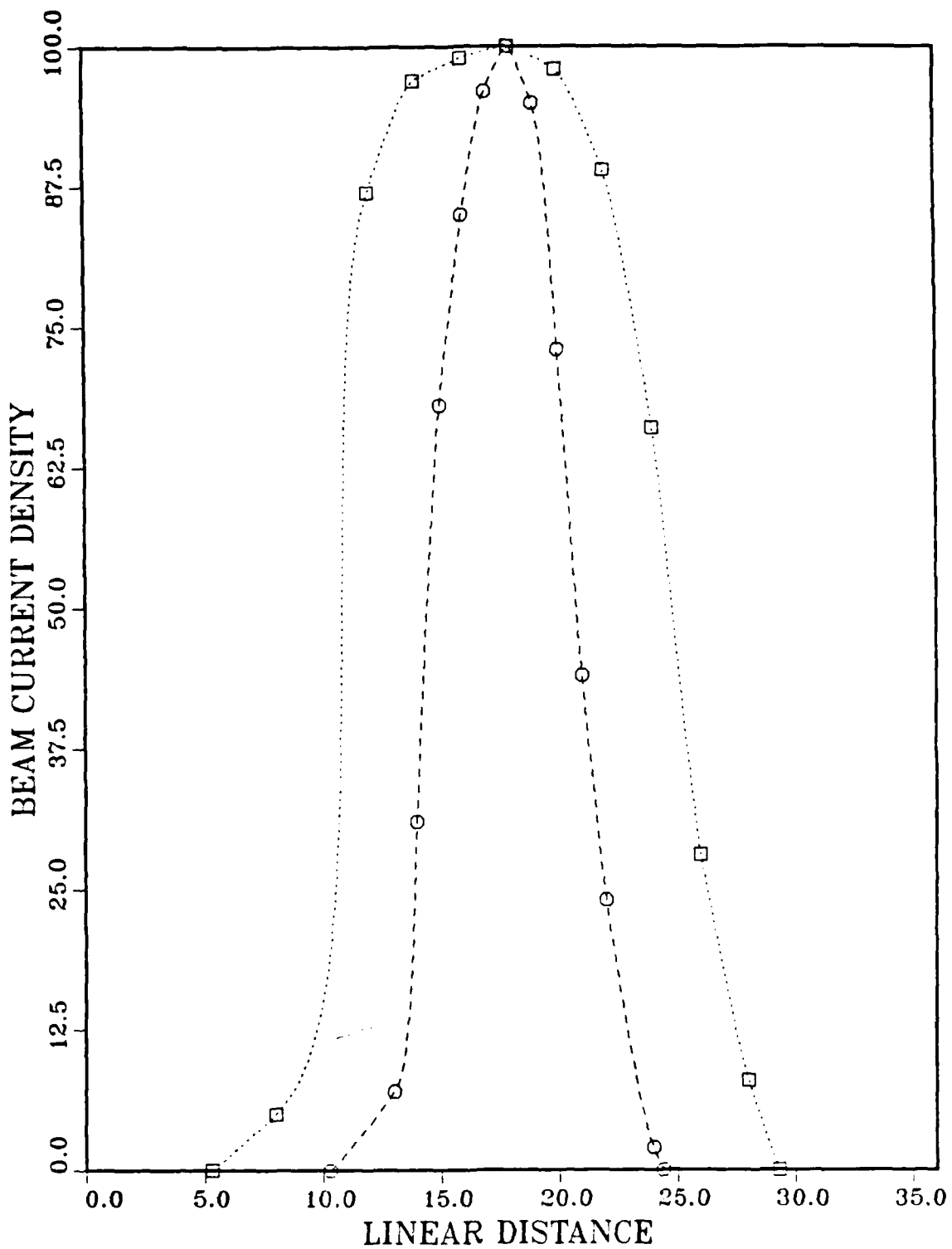
Figure 10. Apparent Beam Current Density versus Linear Distance as Determined From Wire Target Experiment. (Square plot symbols indicate horizontal axis, round symbols indicate vertical axis.)
