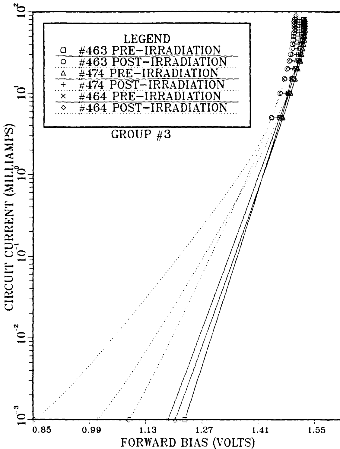
Figure 13. I-V Characteristics for 3 LEDs in Group 3 (— before irradiation, ... after)
