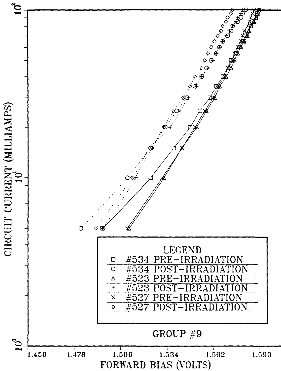
Figure 12. I-V Characteristics for 3 LEDs in Group 9 (expanded scale)
