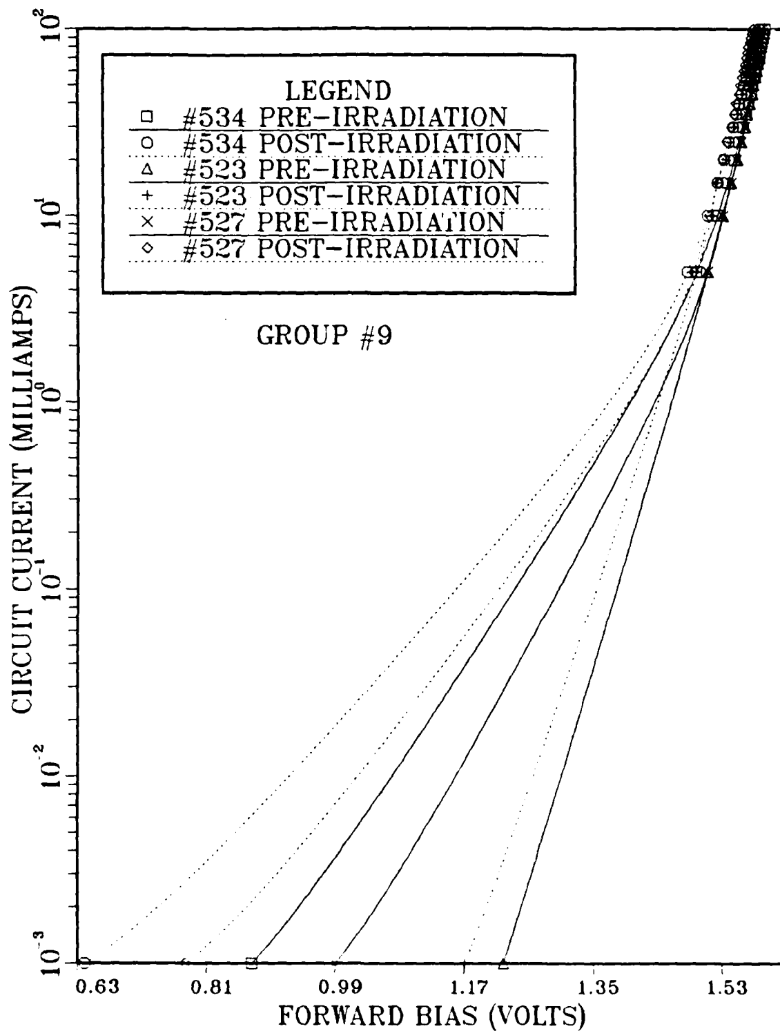
Figure 11. I-V Characteristics for 3 LEDs in Group 9 (- before irradiation, ... after)
