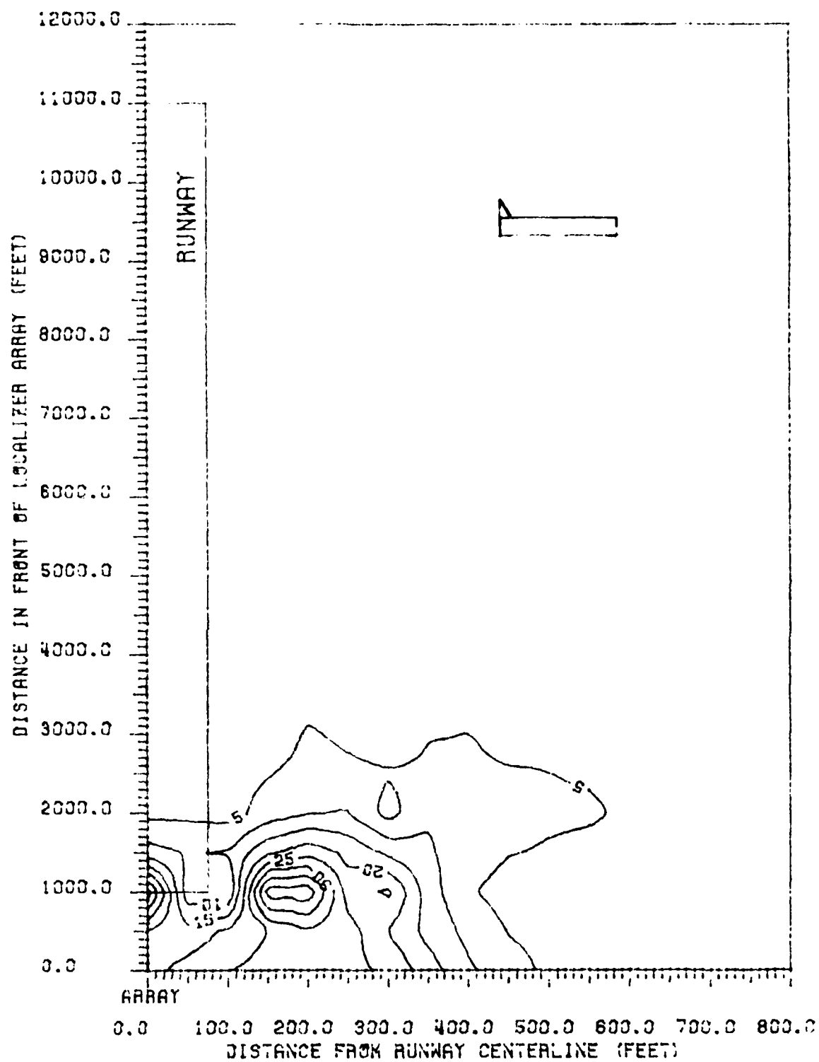
Figure 58 Contours of peak CDI values produced in ILS Zone 2 for a L-1011. L-1011 fuselage is perpendicular to runway centerline, with tail towards the runway. 8-element single-frequency array, LPD antennas.
