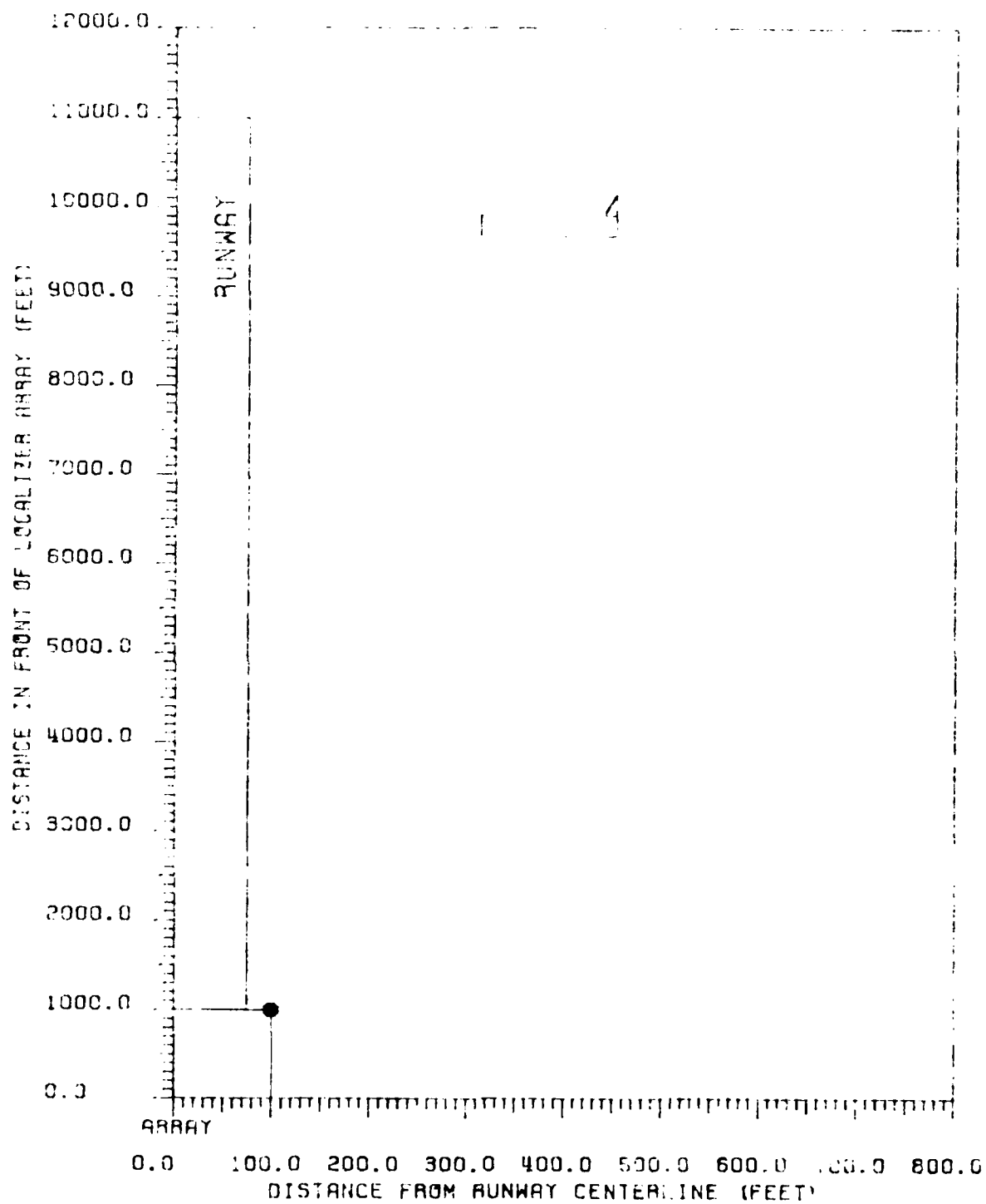
Figure 1. Critical area map for CAT II tolances relative to 0C-9 aircraft. 0C-9 fuselage is perpendicular to runway centerline with tail away from runway. 0C-9 element single-frequency array, LPD antennas.
