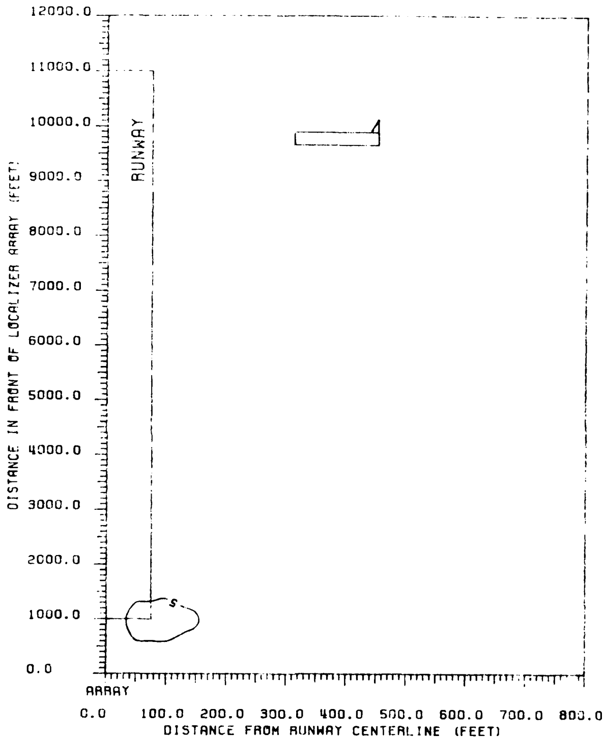
Figure 5. Contours of peak CD values produced in ILS zone 5 for a DC-9. DC-9 baseline is perpendicular to runway centerline, with tail away from the runway. See legend single-frequency array, LPD antennas.
