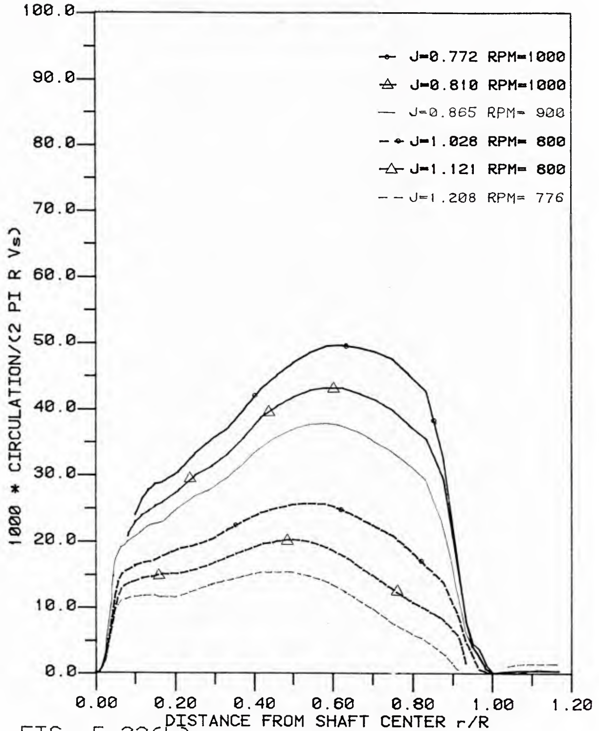
FIG. 5.32(b) CIRCULATION DISTRIBUTION OF PR4498 AT DIFERENT J 'S; X = .84R (HUB APEX)
