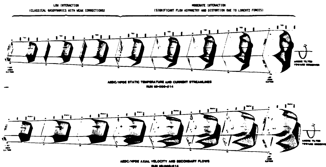
Fig. 6. Development of velocity, temperatures and current under conditions of AEDC/HPDE Run MI-006-014.
