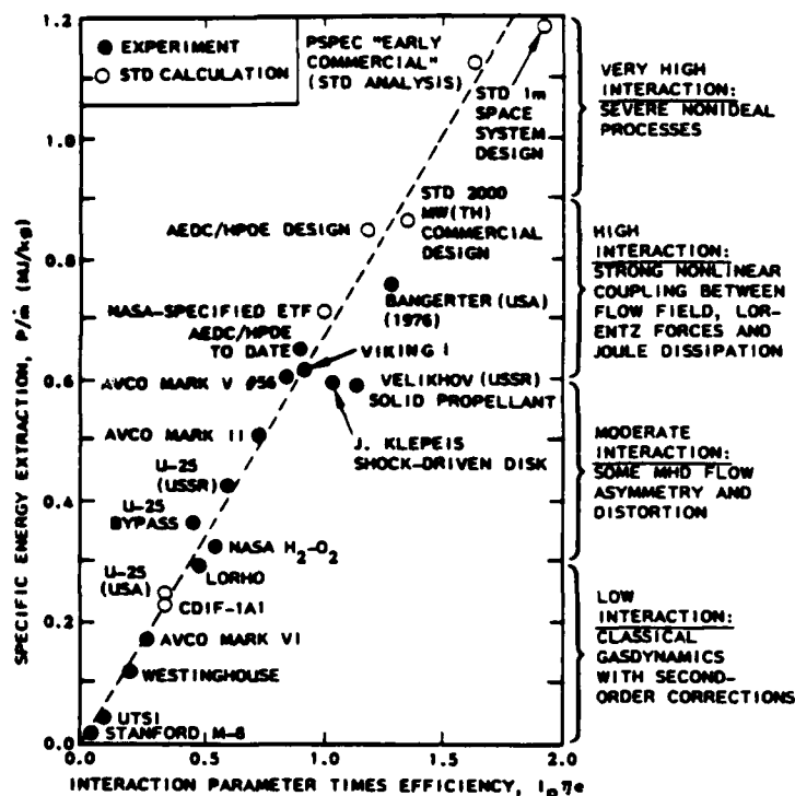
Fig. 5. Interaction levels and specific energy extraction of major MHD power generation experiments and designs in the U.S.A. and the U.S.S.R. Solid points indicate experimental test data. Interaction regimes are arbitrarily divided on the basis of the degree of MHD flow distortion in the STD calculations.
