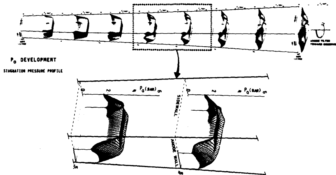
Fig. 9. Development of the stagnation pressure profiles in the 5 tesla AEDC/HPDE simulations of Figs. 7(c) and 8(c).
