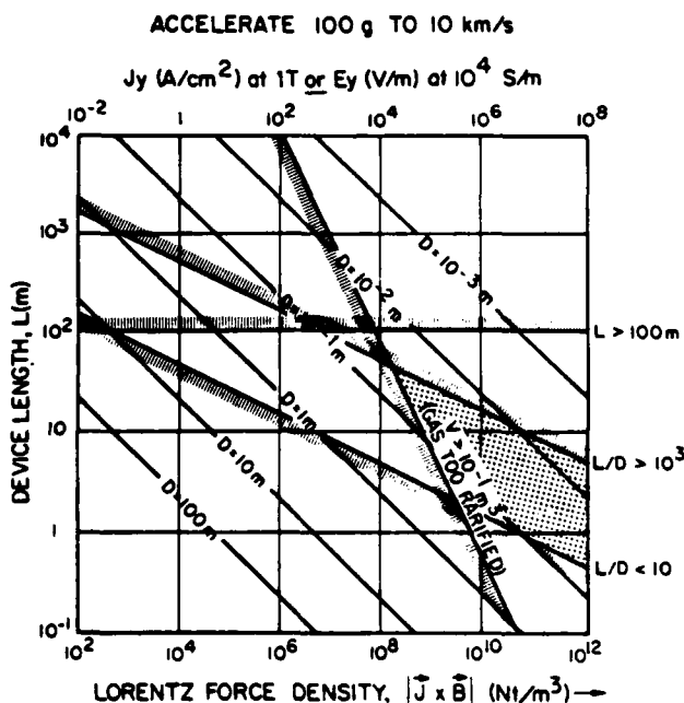
Fig. 2. Feasible domain to accelerate 100 g mass to 10 km/s by application of the Lorentz force in an imposed magnetic field of 1 T in a linear MHD device.
