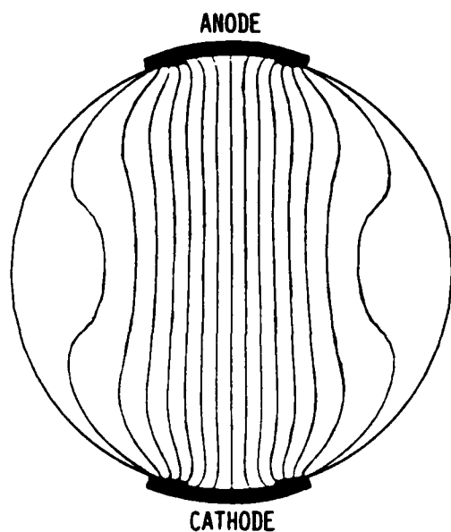
Fig. 13. Current Streamlines in the cross section at the 5 m station in Fig. 11 for an electrode subtended angle of 40^\circ . Peak transverse current density 0.5 \text{ A/cm}^2 .
