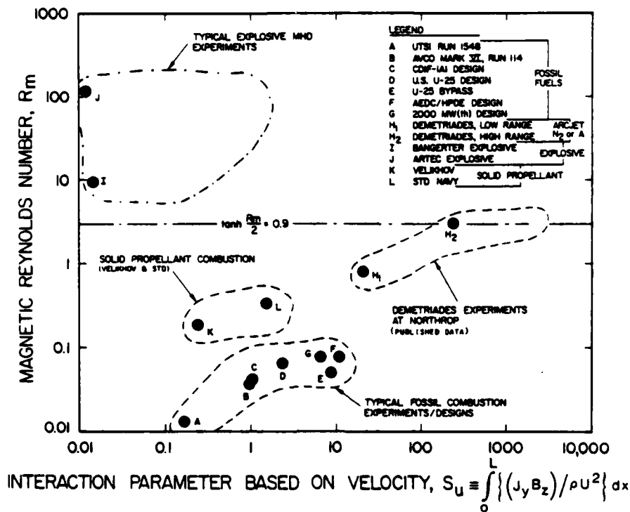
Fig. 3. Map of the magnetic Reynolds number and interaction parameter based on velocity for some significant MHD generator experiments and designs using as working fluids (a) fossil fuel combustion products, (b) solid propellant combustion products, (c) explosion products and noble-gas driver gas, and (d) nitrogen or argon arc-jet plasma.
