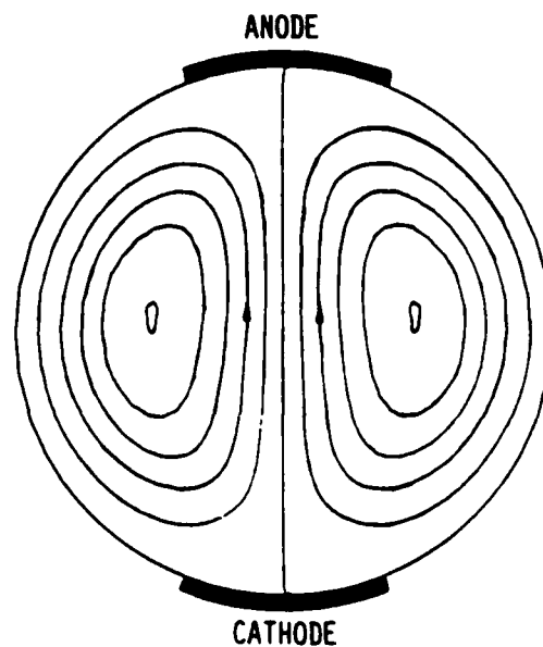
Fig. 14. Streamlines of the secondary flow velocity corresponding to Fig. 13. Peak transverse velocity components are 9% of the mean axial velocity.
