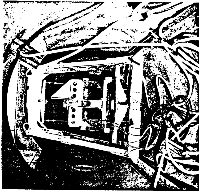
Fig. 4. Rear view of MGD driver in vacuum tank
