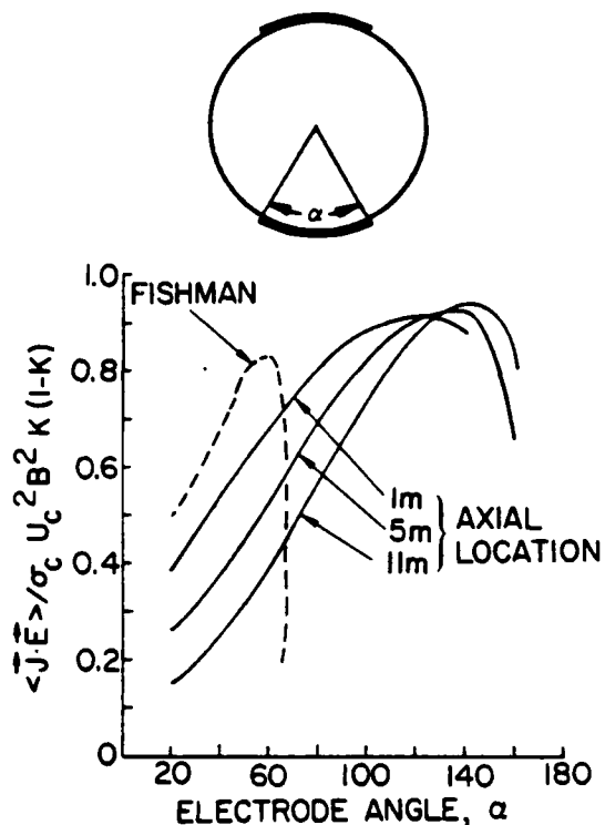
Fig. 11. Total power density relative to the core power density at three stations in a 1000 MW (thermal input) coal-fired MHD generator with circular cross section, as a function of the angle subtended by the electrodes. Also shown (dashed) are the idealized, constant property results of F.J. Fishman, J. Advan. Energy Conv., 4:223-236 (1964).
