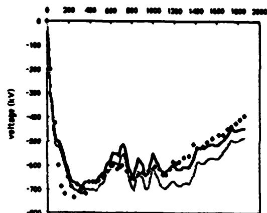
Fig. 10. MELBA experimental voltage (points) for type A shot compared to SPICE code using experimental impedance profile with: Actual charging voltages (dark line) V_1 = +56 kV, V_2 = +56 kV, and, increased charging voltage on the reversed stage, V_1 = +56 kV, V_2 = +90 kV
