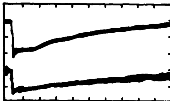
Fig. 3. Voltage (upper, 400 kV/div) and current (lower) into 127 ohm resistive load without crowbar firing - (1 μs/div). Charging voltages: V_1 = +56\ \text{kV} ; V_2 = +54\ \text{kV} .
