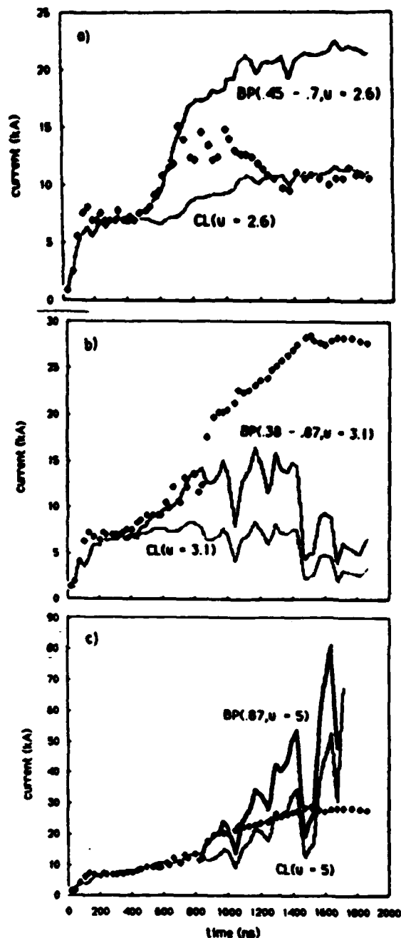
Fig.9 a) Experimental current data (points) from type A shot compared with constant closure velocity model ( u = 2.6 cm/ \mu s ) for Child-Langmuir (CL) current and bipolar flow (BP) turned on linearly from 0.45 \mu s to 0.7 \mu s . b) Experimental current data from type B shot compared to Child-Langmuir (CL) with closure velocity of 3.1 cm/ \mu s and bipolar (BP) flow turned on linearly from 0.38 \mu s to 0.87 \mu s with constant closure velocity. c) Experimental current data from type B shot compared to Child-Langmuir (CL) with a constant closure velocity of 5 cm/ \mu s and bipolar flow (BP) turned on at 0.87 \mu s .
