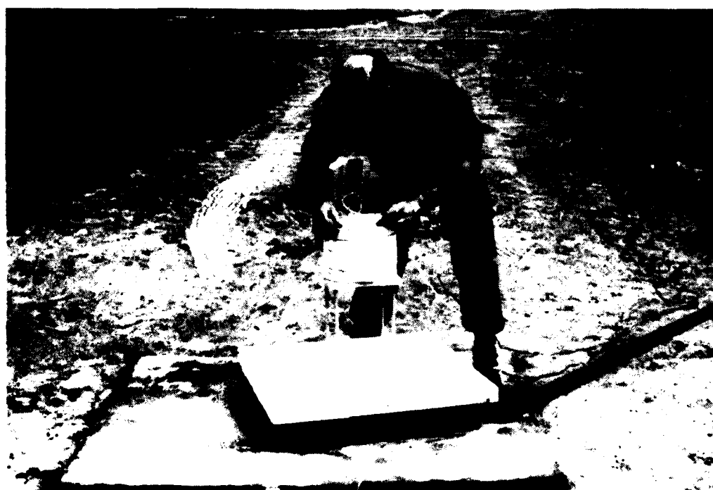
FIGURE 3 Arrangement for pumping liquid nitrogen into the plate cooling box. Truck and equipment is protected from the blast by a wall constructed of concrete "pentane" blocks.
