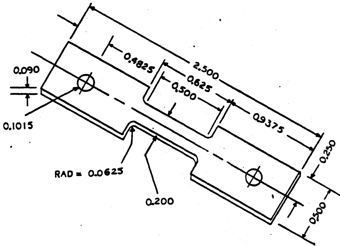
Figure 3.3 Tensile test specimen geometry
