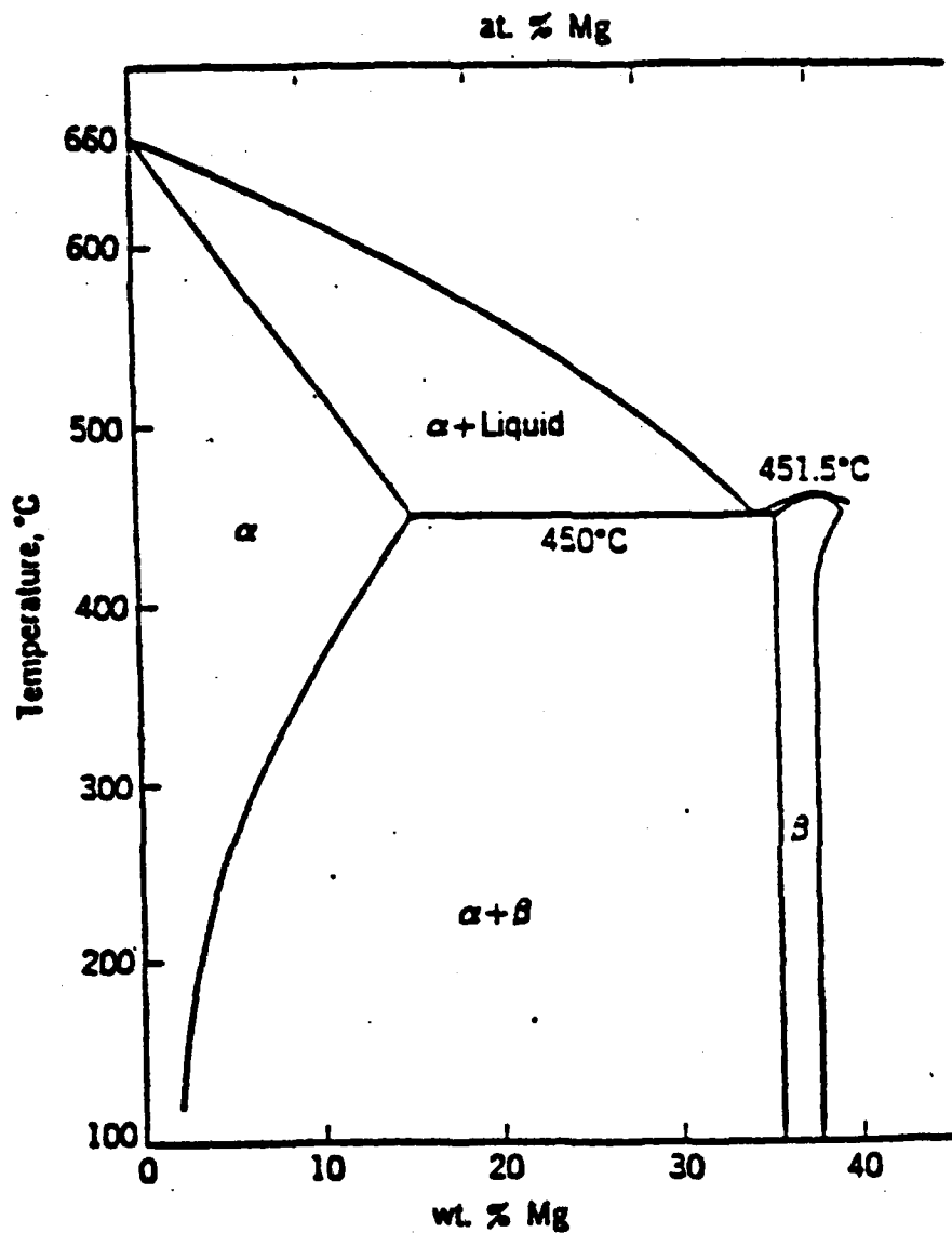
Figure 2.2 Aluminum-magnesium phase diagram
