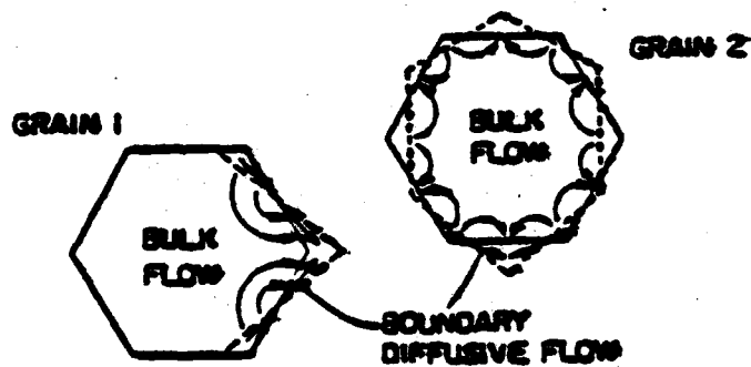
Figure 2.1 Ashby-Verrall grain boundary switching model
