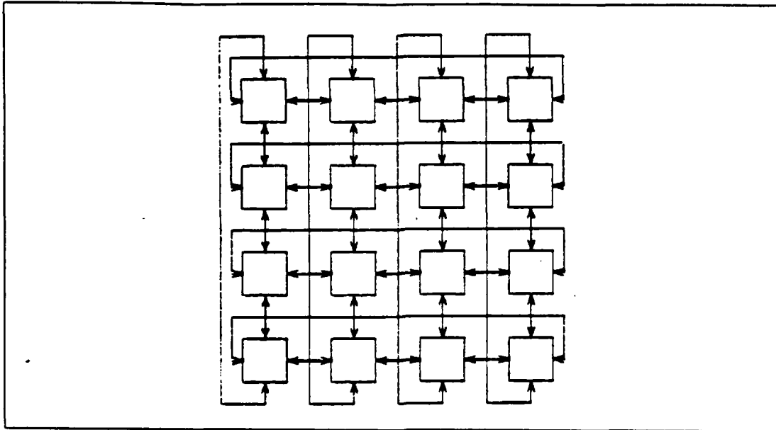
Figure 4.9 A Complete Loop Regular Array
