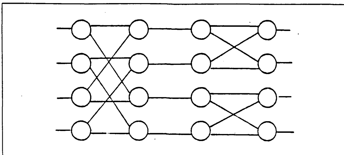
Figure 4.6 Butterfly Structure
