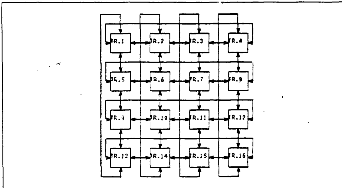
Figure 6.2 16 Transputer Regular Array Complete Loop
