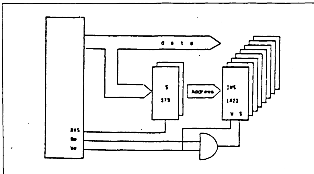
Figure 2.1 Memory Interface Driving Static RAM's
