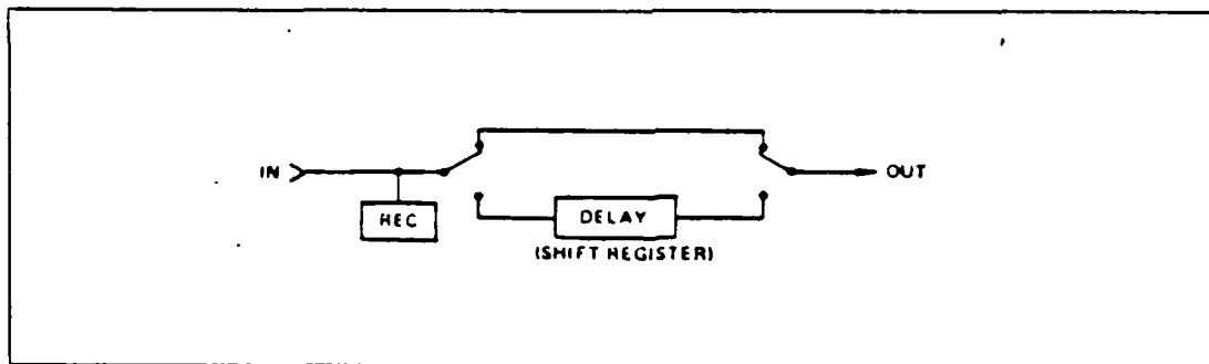
Figure 5.1 Basic Function of Delay Insertion Loop
