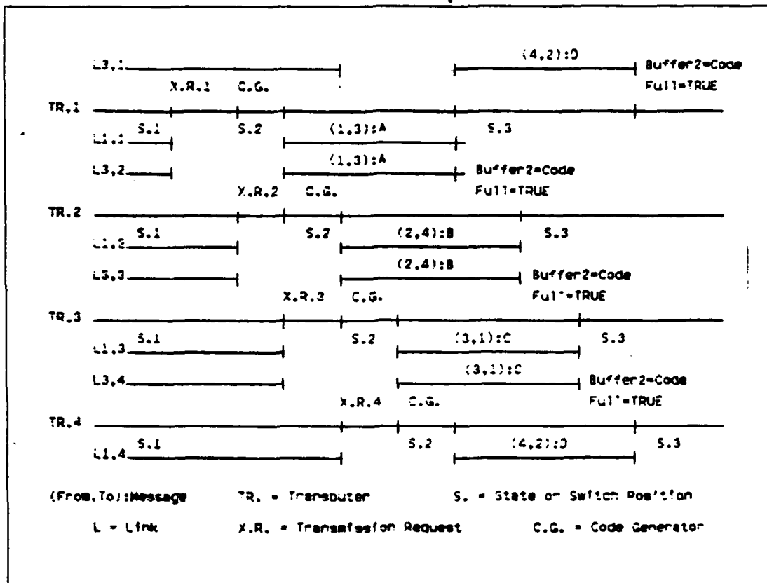
Figure 5.6 Simultaneous Transmission of Four Transputers
