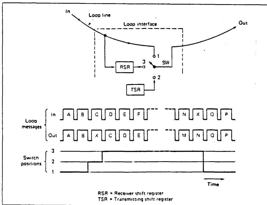
Figure 5.3 Delay Insertion Loop and its Operation
