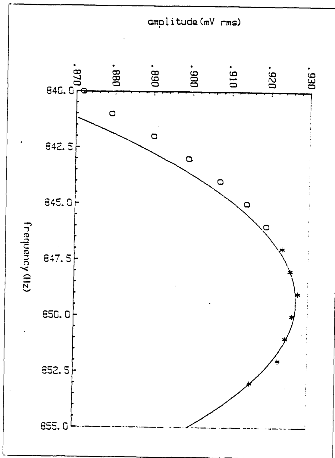
Figure 2.1 Parabolic Curve Fit in Frequency
