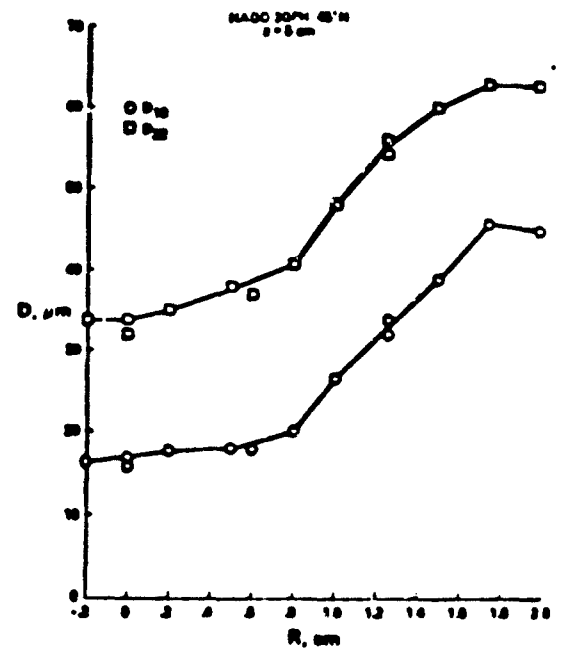
Radial Distribution of Mean Drop Size
