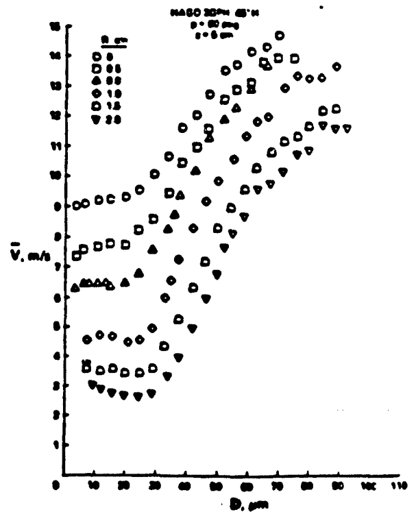
Radial Drop Size - Velocity Correlations
