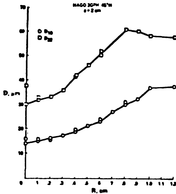
Radial Distribution of Mean Drop Size
