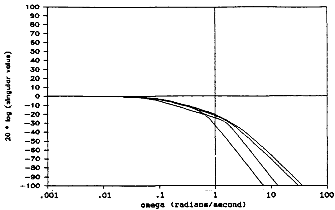
Figure 4.6 Singular Values of the Closed Loop
