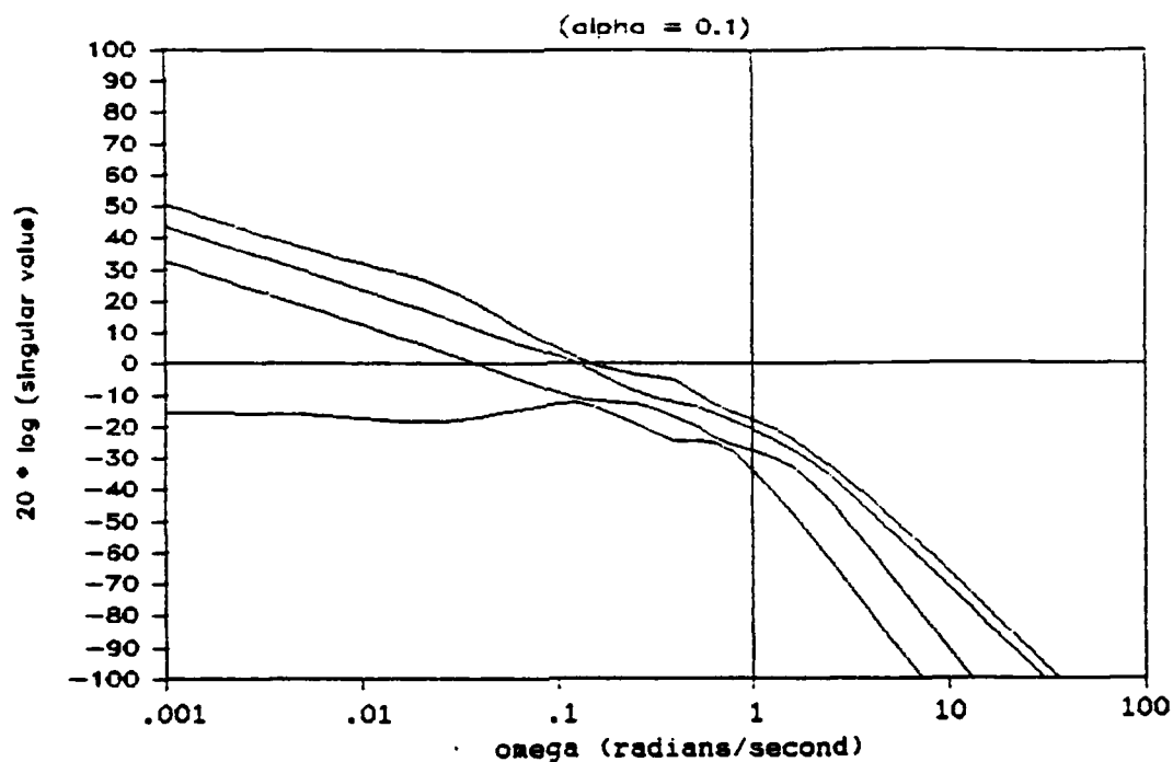
Figure 6.3a Singular Values of G(s)K(s) for \alpha = 0.1
