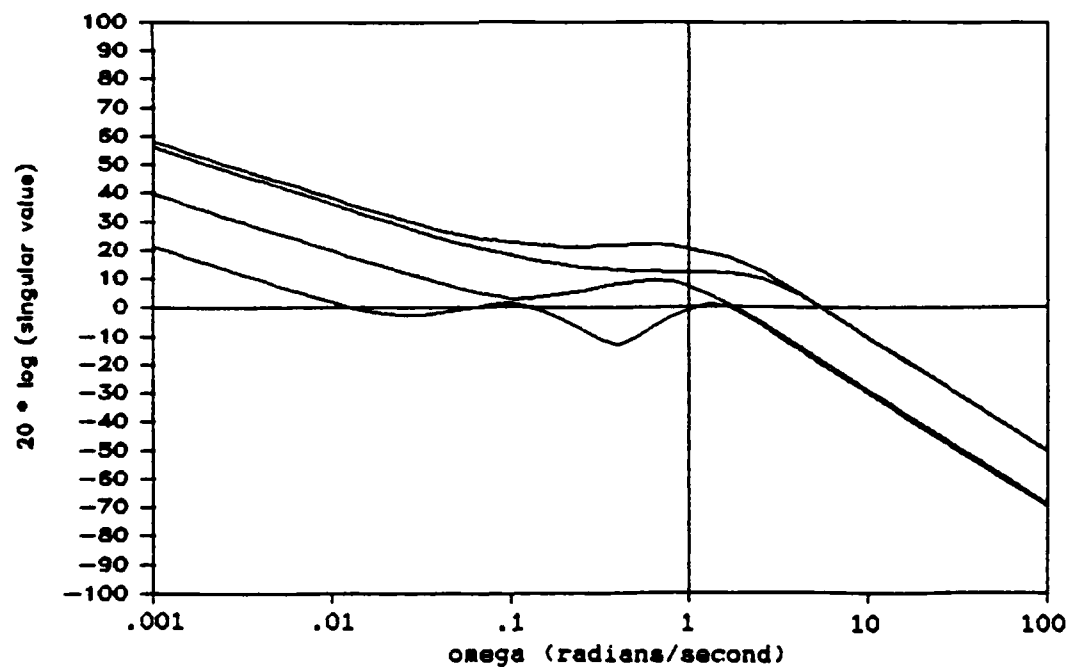
Figure 4.5b Singular Values of K_a(s)
