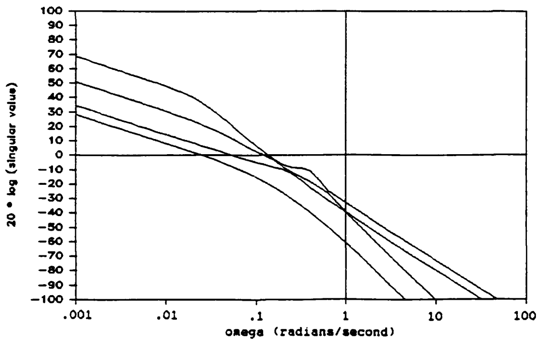
Figure 3.9 Singular Values of Augmented Plant G(s)
