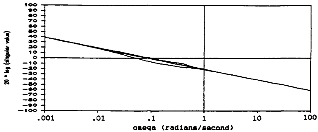
Figure 4.3a Singular Values of G_{f01}(s)
