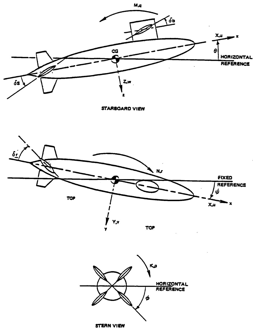
Figure 2.1 Body-Fixed Coordinate System for a Submarine
