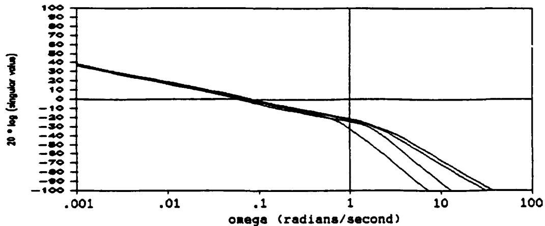
Figure 4.3c Singular Values of G(s)K(s)
