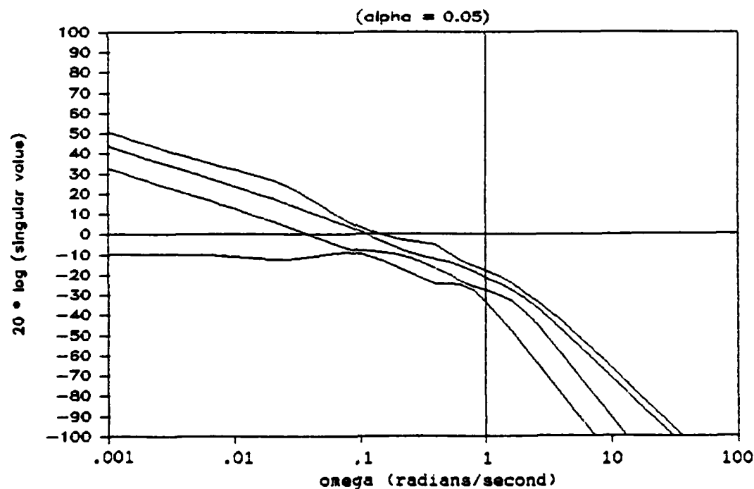
Figure 6.3b Singular Values of G(s)K(s) for \alpha = 0.05
