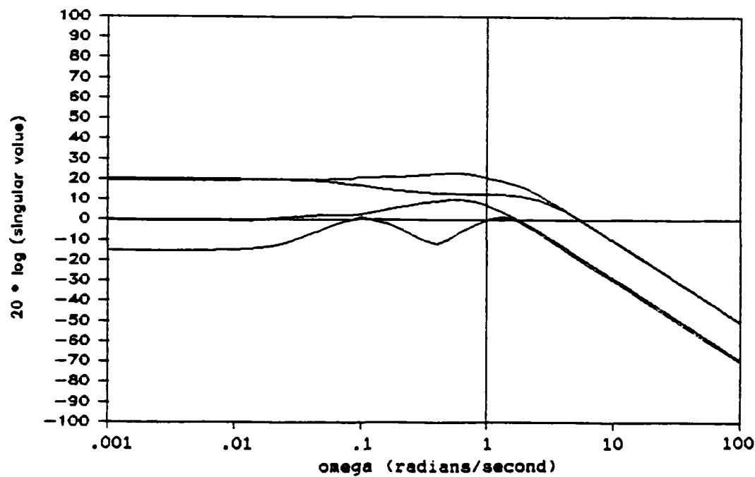
Figure 4.7 Singular Values of K_r(s)
