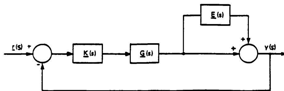
Figure 3.10 MIMO Feedback Loop With Multiplicative Error
