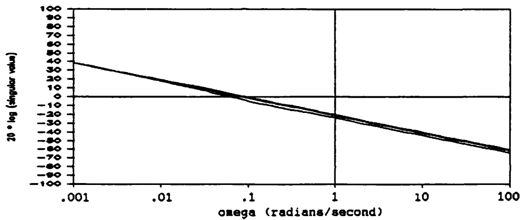
Figure 4.3b Singular Values of G_{kf}(s)
