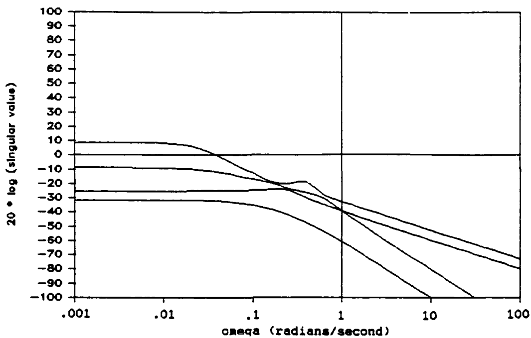
Figure 3.8 Singular Values of Original Plant G_p(s)
