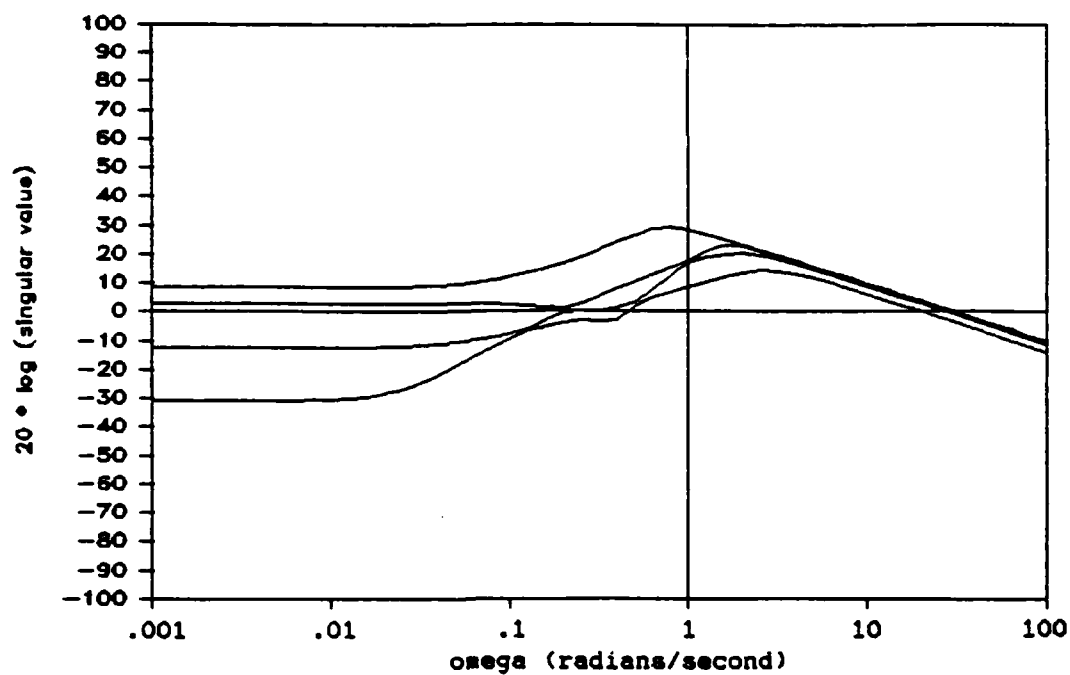
Figure 4.5a Singular Values of K(s)
