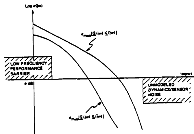
Figure 3.6 Singular Value Requirements for G(s)K(s)
