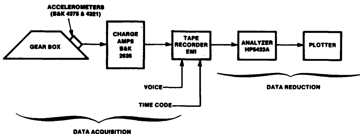
Figure 19. Instrumentation System.
