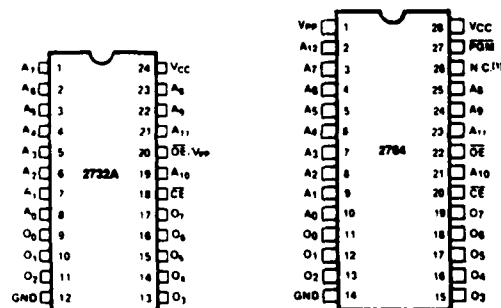
Figure 2. Pin Configurations
