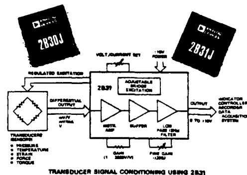
TRANSDUCER SIGNAL CONDITIONING USING 2B31
