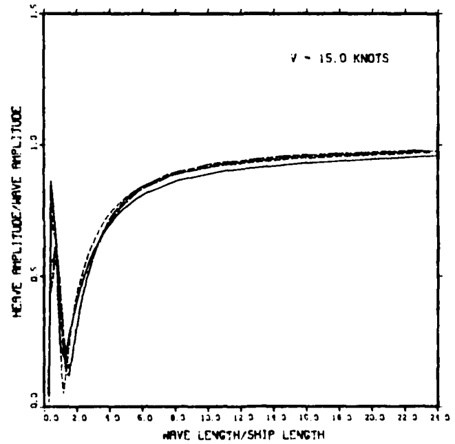
Figure 8 - Heave Transfer Functions in Regular Following Waves for Configurations in the GM L Series
