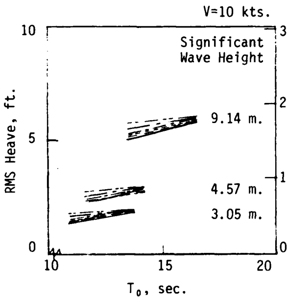
Figure 38 - Heave RMS Responses in Irregular Following Seas for Configurations in the LCF Series
