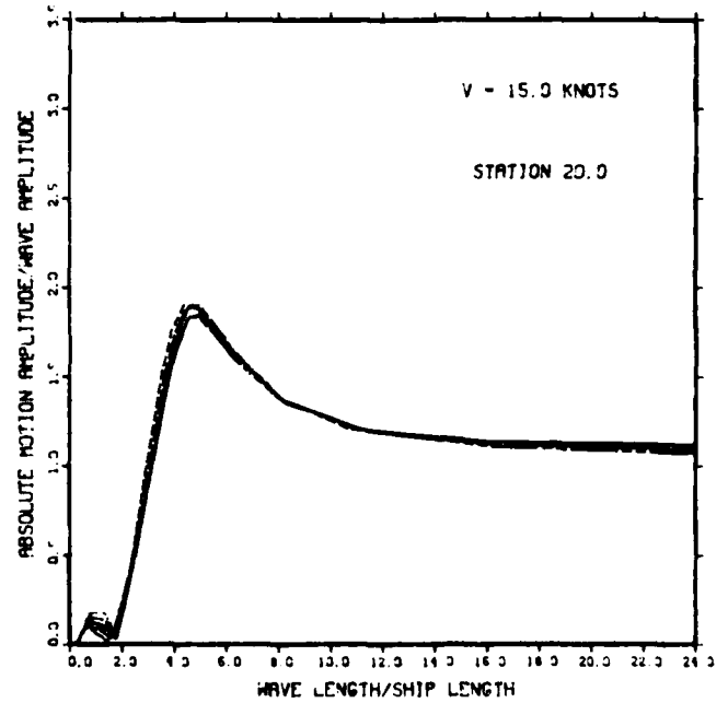
Figure 27 - Absolute Stern Motion Transfer Functions in Regular Head Waves for Configurations in the LCF Series
