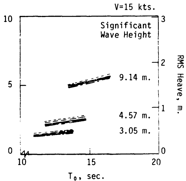
Figure 38 - Heave RMS Responses in Irregular Following Seas for Configurations in the LCF Series
