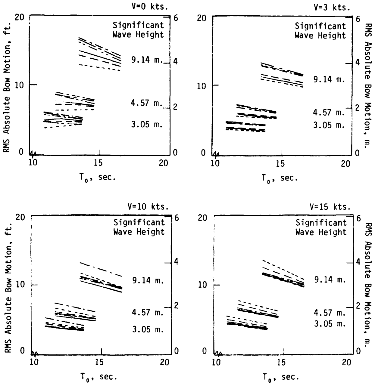
Figure 41 - Absolute Bow Motion in Irregular Following Seas for Configurations in the LCF Series
