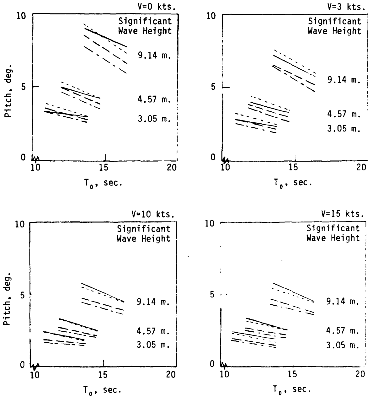
Figure 19 - Pitch RMS Responses in Irregular Following Seas for Configurations in the GM L Series
