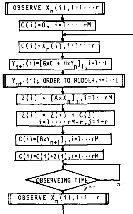
Figure 2. AR Steering Algorithm
