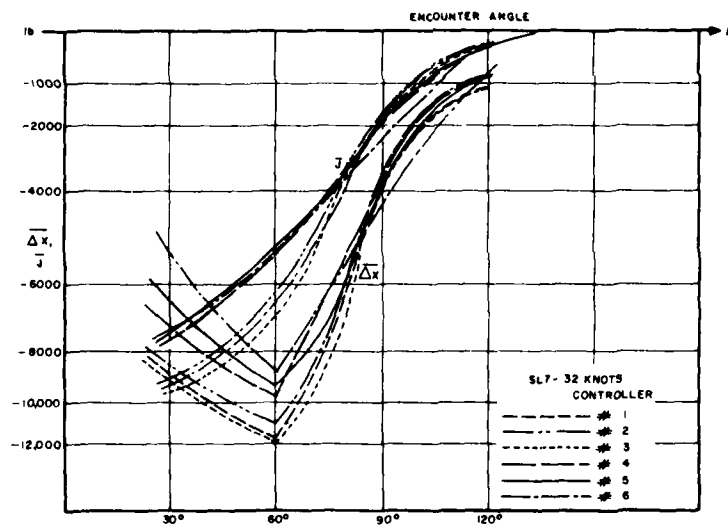
Figure 8. SL-7 - 32 Knots: Effect on Added Resistance Performance of Variation of \lambda in LQG Controller
