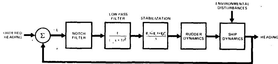
Figure 1. Closed Loop Control System
