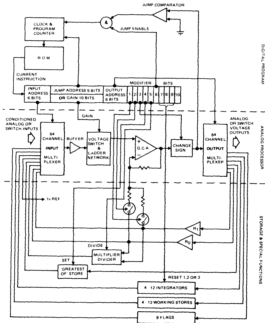
FIGURE 2 BLOCK DIAGRAM OF P.A.C. STRUCTURE
