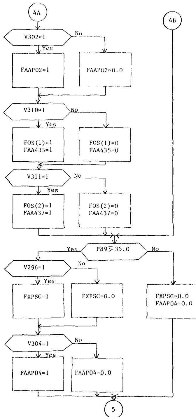
Figure 1A. Fire Room, Control Air (Sheet 6 of 12)
