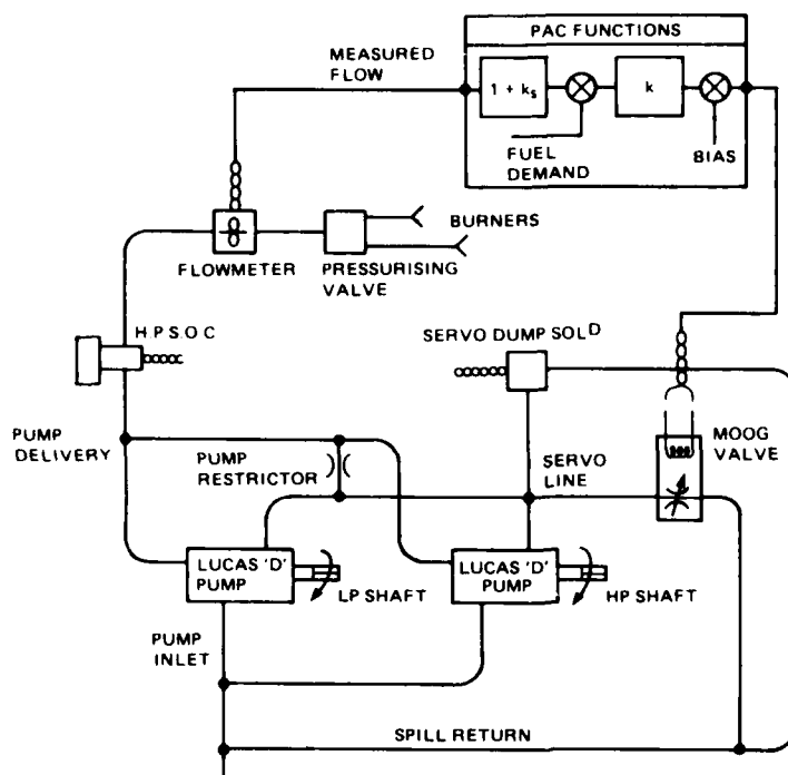
FIGURE 1 HYDRAULIC INTERFACE FUEL SYSTEM
