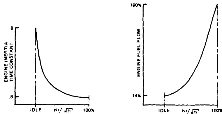
FIGURE 4 ENGINE STEADY STATE AND DYNAMIC CHARACTERISTICS
