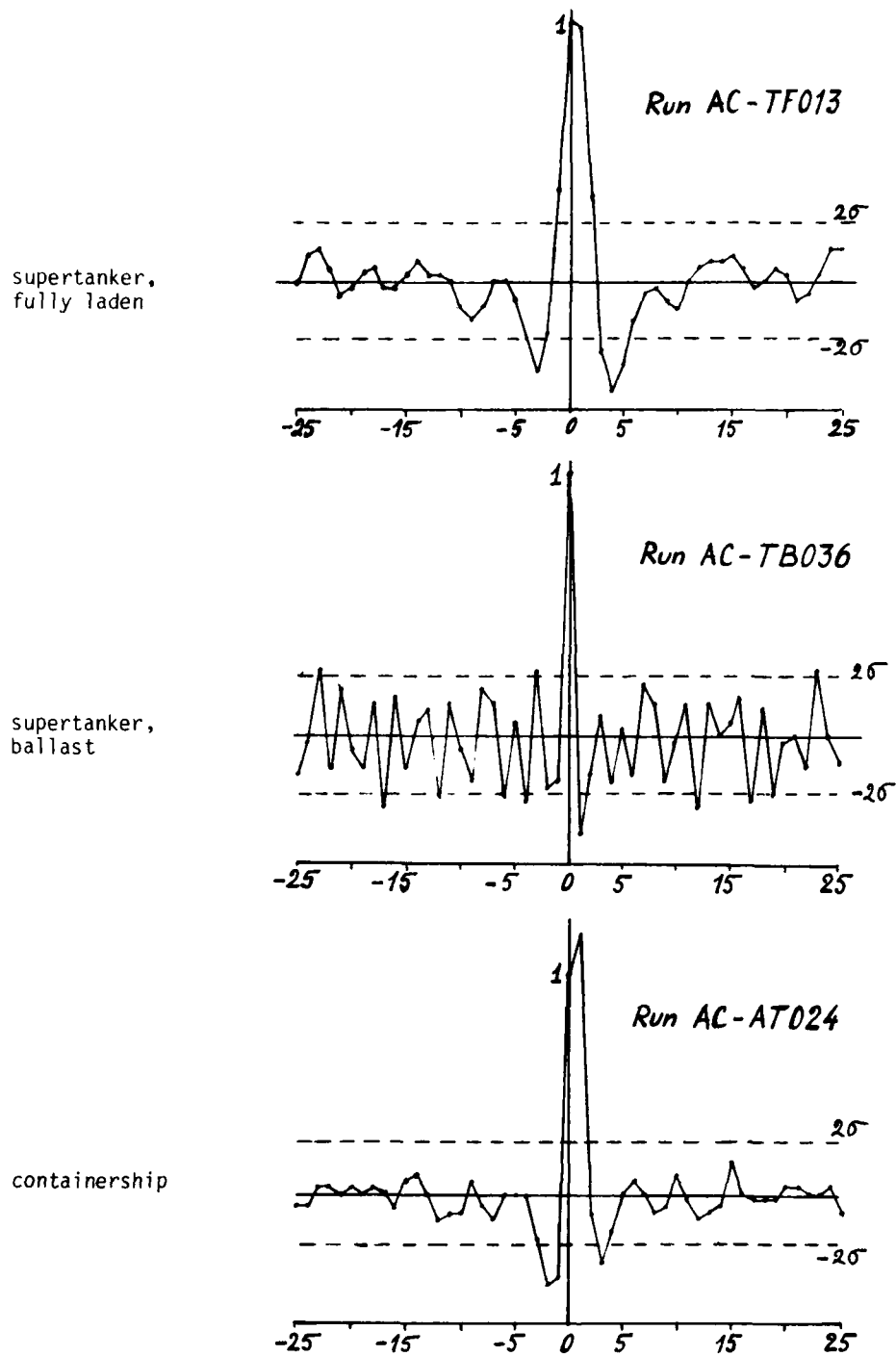
Figure 10: Cross-correlation function of systems input and output signal for the three considered ships.
