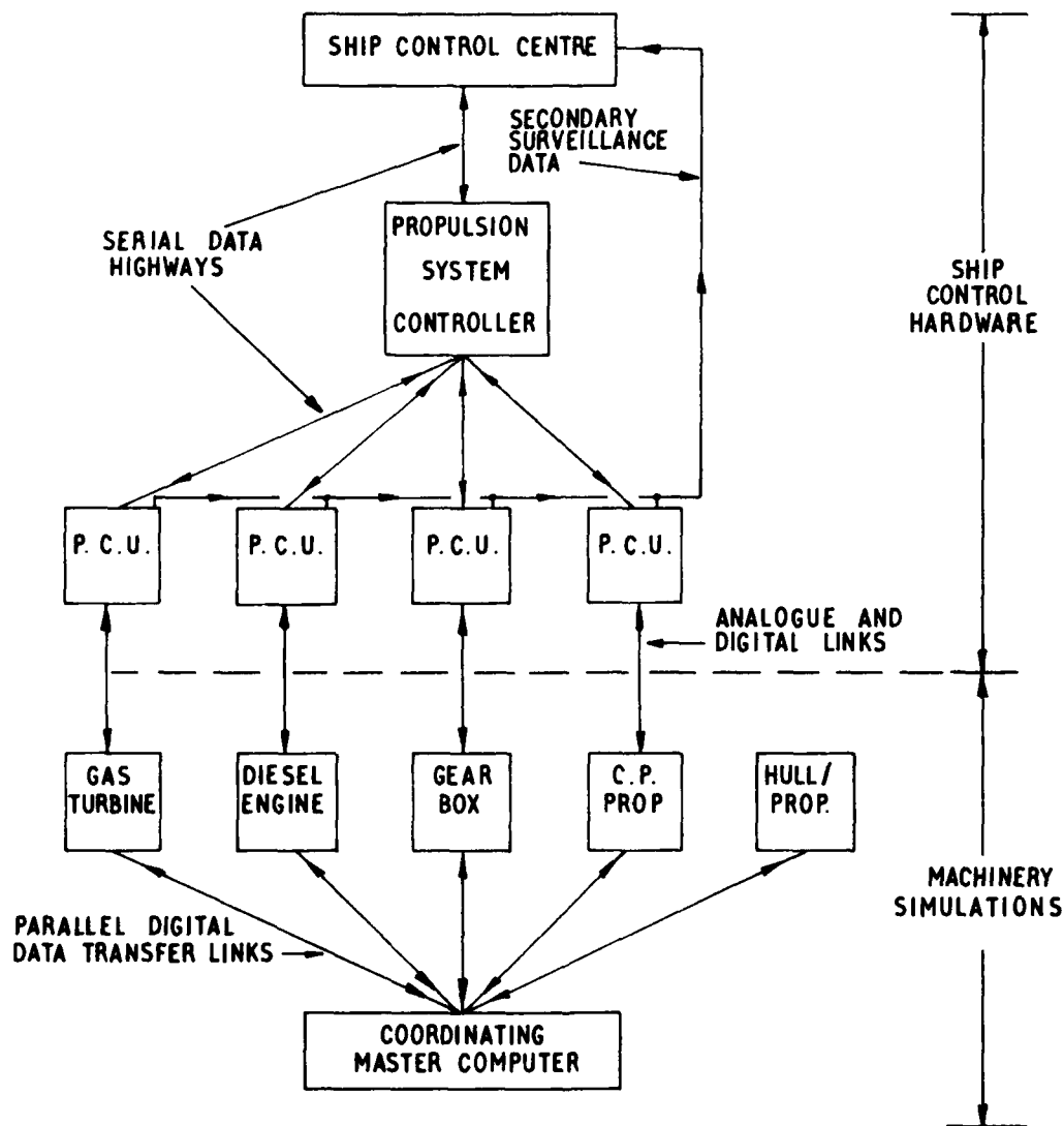
Figure 2. Illustrates communication between simulated propulsion machinery and control system
