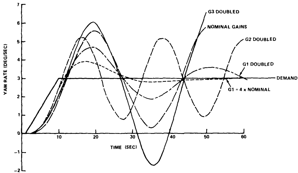
FIGURE 12. CRAFT OVERLAND YAW RATE FOR VARIOUS GAIN SETTINGS FOR A YAW RATE DEMAND OF 3DEG/SEC
