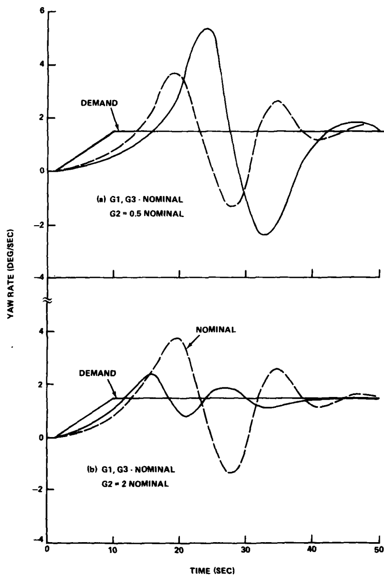
FIGURE 9. SENSITIVITY OF TURN RATE WITH RESPECT TO VARIATIONS IN G2 AT 50 kt
