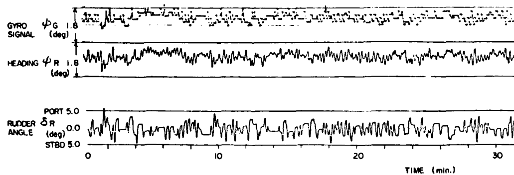
Fig. 7 Conventional APS without Weather Adjust at Heavy Sea
