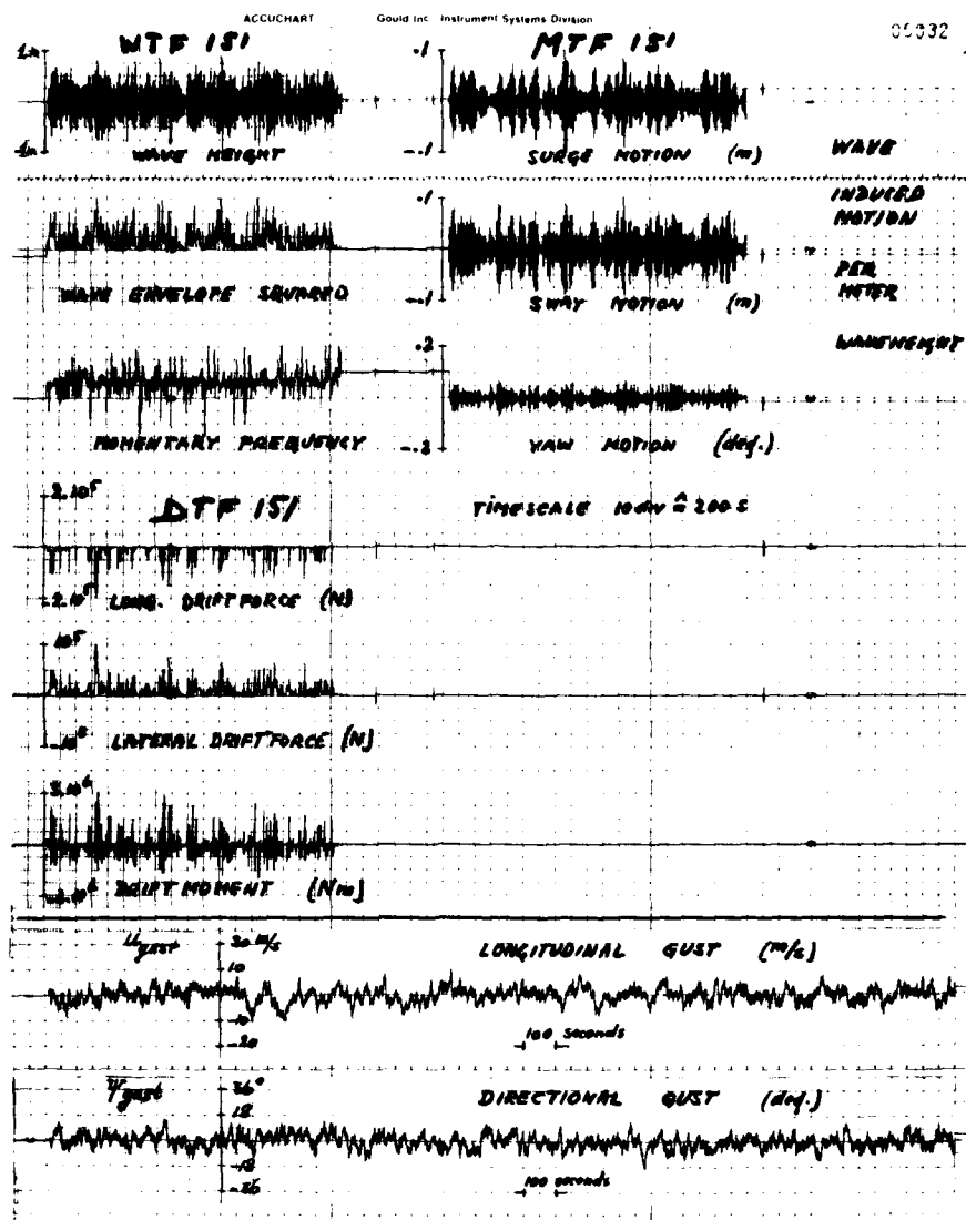
Figure 5: Timeseries of wave induced motions, driftforces and -moment of VLCC, fully laden. Wave direction: 30° off bow. Time series of windgust signals.
