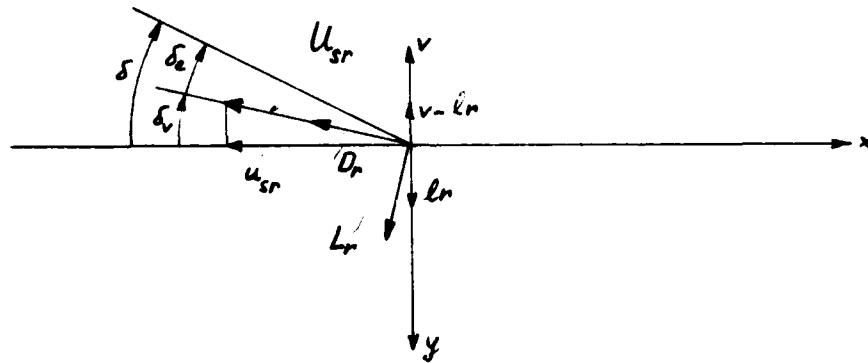
Figure 18: Relative speeds with respect to the rudder and forces on the rudder.
