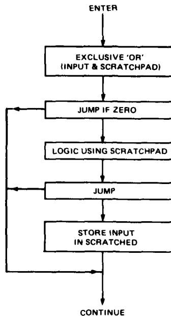
FIGURE 7 SCRATCHPAD FILTER LOGIC
