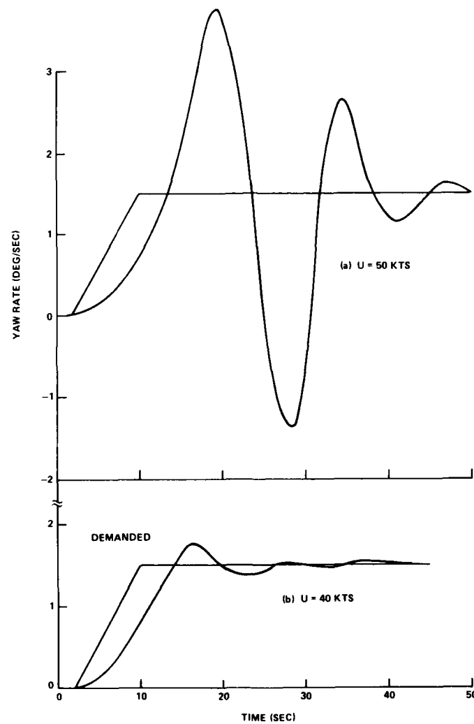
FIGURE 4. SIMULATED TURN RATES FOR JEFF(A) AUTOMATIC CONTROLLER TURNS AT 40 AND 50 kts WITH NOMINAL GAINS
