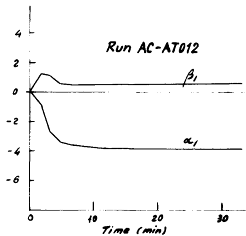
Figure 11: Rate of convergence of model coefficients \alpha_1 and \beta_1 . Runs AC - TF 007 (tanker, full), AC - TB 015 (tanker, ballast), AC - AT 012 (containership).
