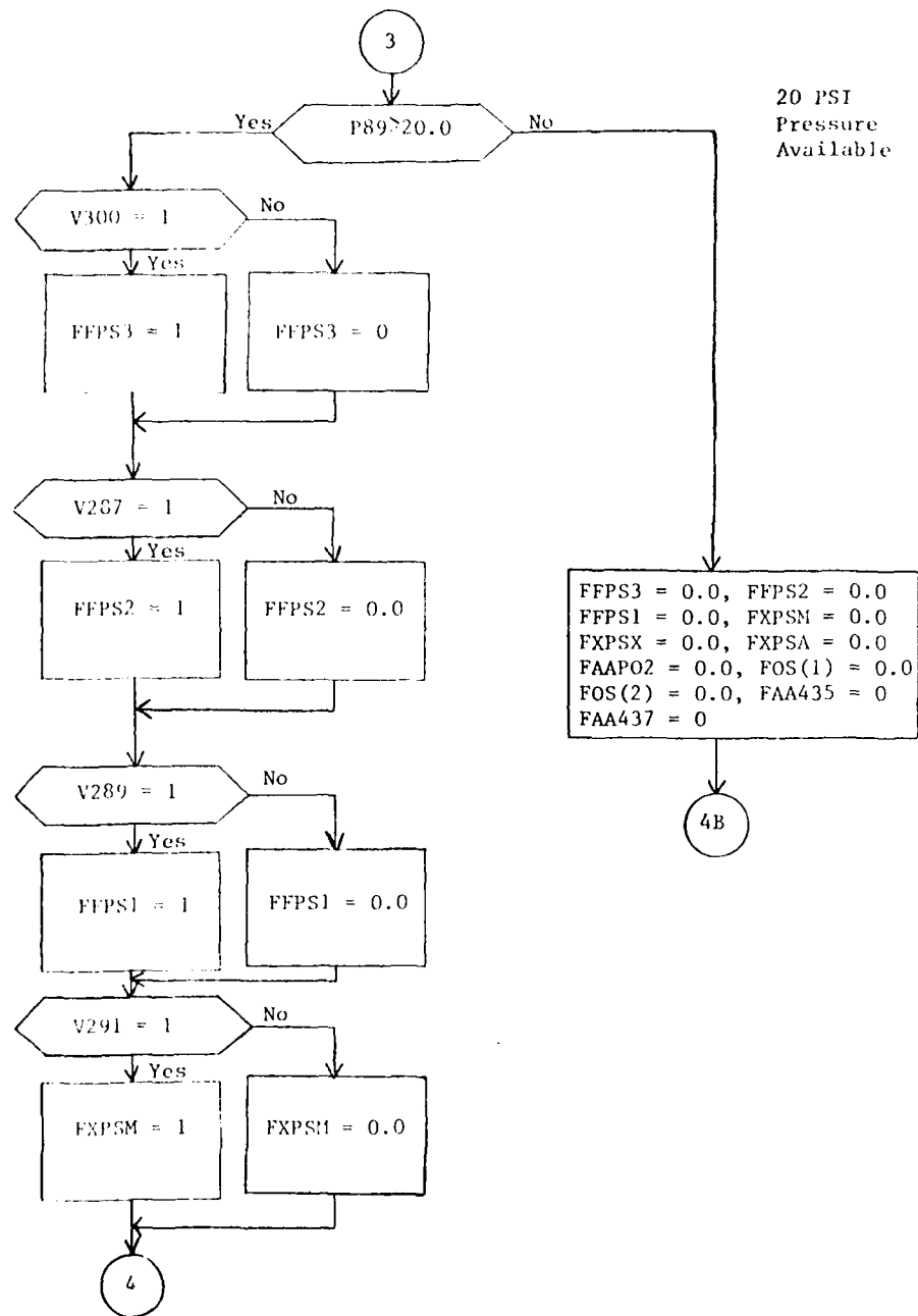
Figure 1A. Fire Room, Control Air (Sheet 4 of 12)
