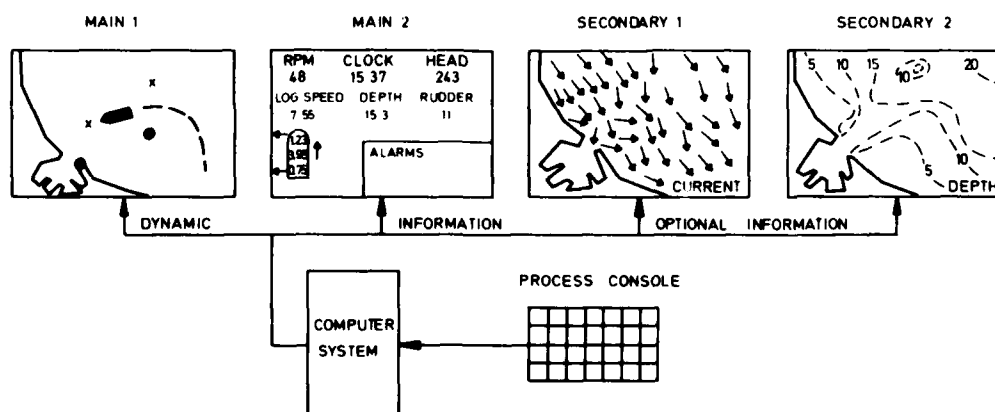
FIG. 6 Example of information available for single ship control
