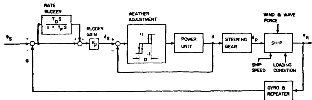
Fig.1 Block Diagram of Conventional APS
