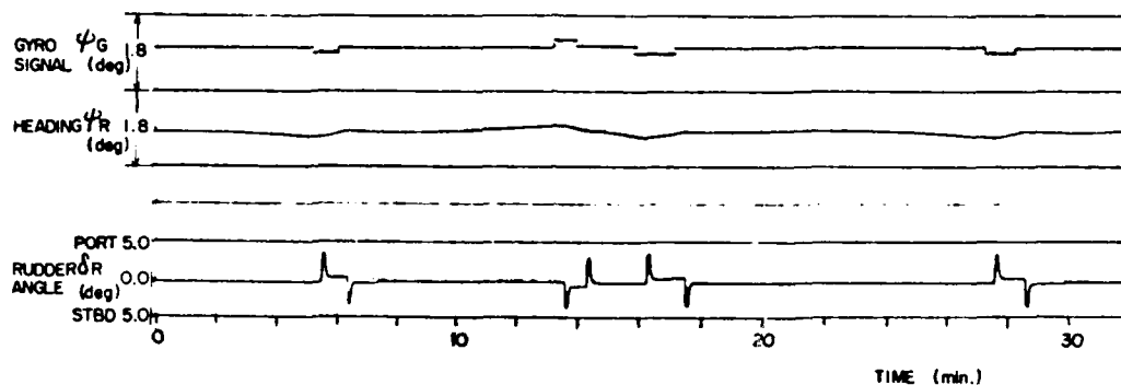
Fig. 6 New Auto PILOT at Calm Sea
