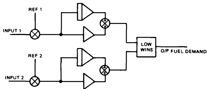
FIGURE 5 TYPICAL 2-LOOP CONTROLLER
