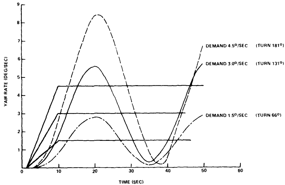
FIGURE 11. CRAFT OVERLAND YAW RATE AT NOMINAL GAIN SETTINGS FOR VARIOUS YAW RATE DEMANDS
