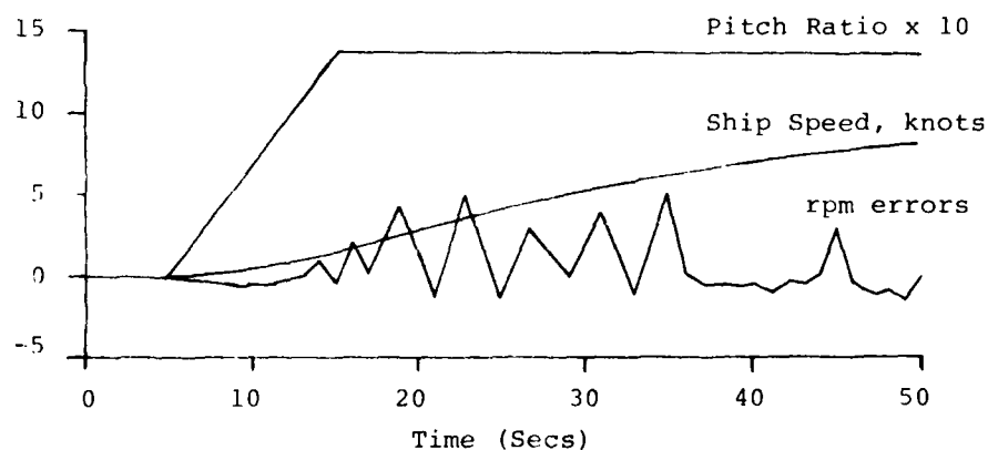
Figure 4. Plant Response, Weights (i).
