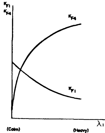
Fig. 3 Filter Gains vs. \lambda_1 (Sea State)
