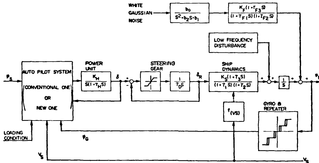
Fig. 4 Block Diagram of Simulation Model
