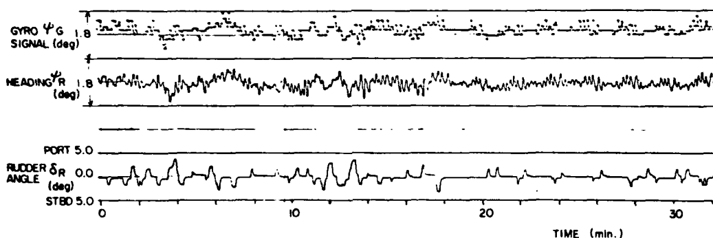
Fig. 8 Conventional APS with Weather Adjust at Heavy Sea
