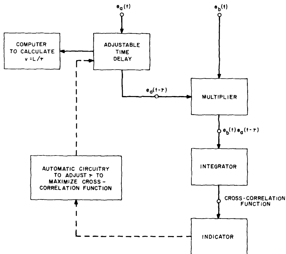
Figure 8. Simple Cross-Correlation Circuitry for Measuring Speed
