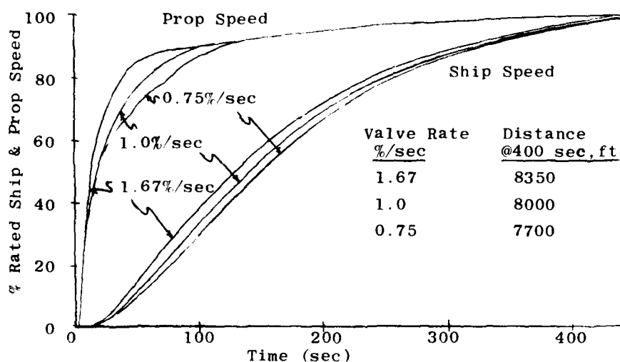
Figure 9. Ahead Reach For Crash-Back And Normal Throttle Valve Maneuvering Rates
