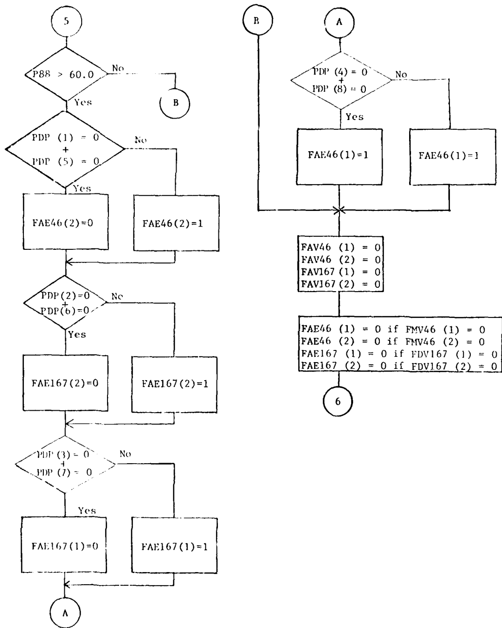
Figure 1A. Fire Room, Control Air (Sheet 7 of 12)
