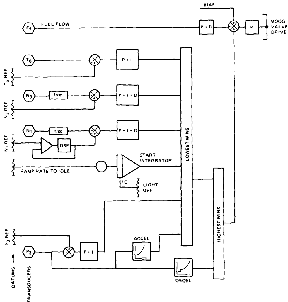
FIGURE 3 PROGRAMMED CONTROL FUNCTIONS
