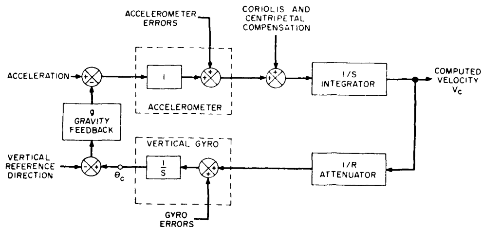
Figure 11. Pure Inertial System for Computing One Horizontal Velocity Component
