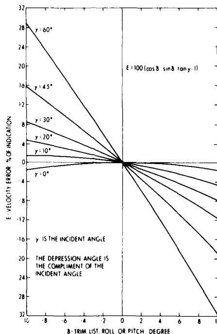
Figure 10. Correlation Speed Sensor Errors Caused by List, Trim, Roll, and Pitch
