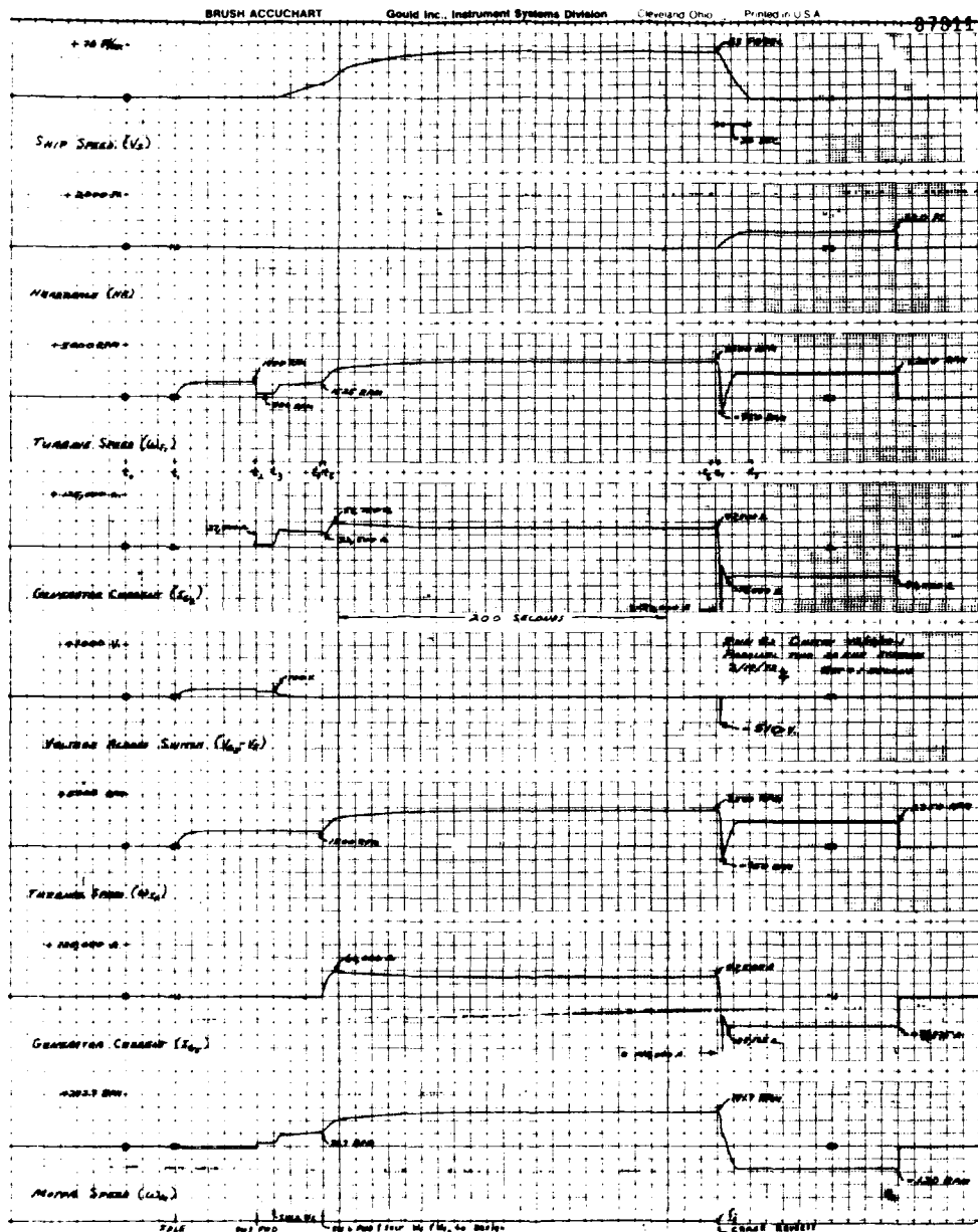
Figure 3. Standard Run: Two 15 MW Turbogenerator Systems
