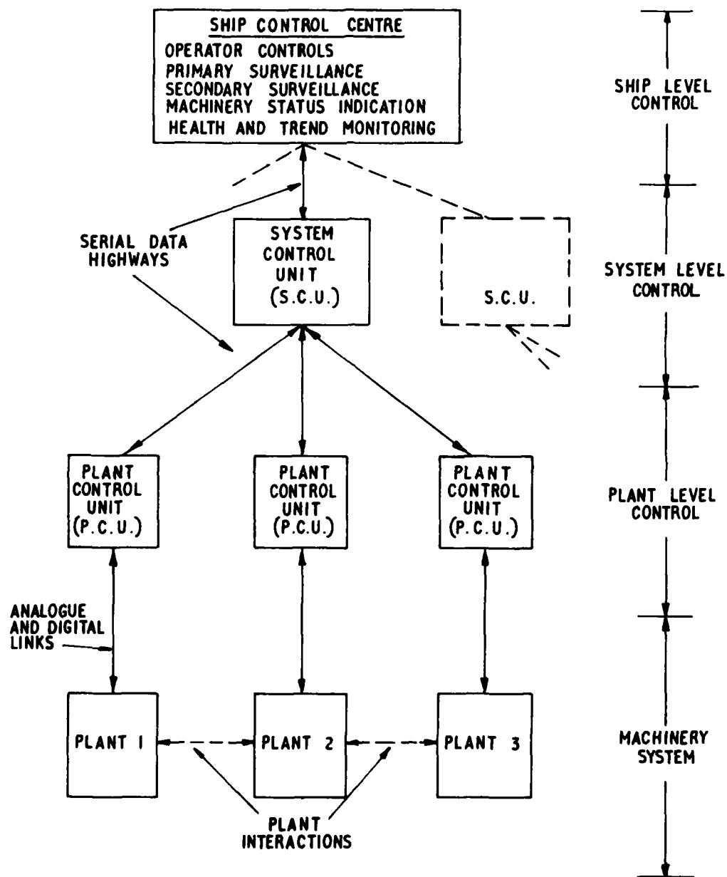
Figure 1. Hierarchical structure of control system
