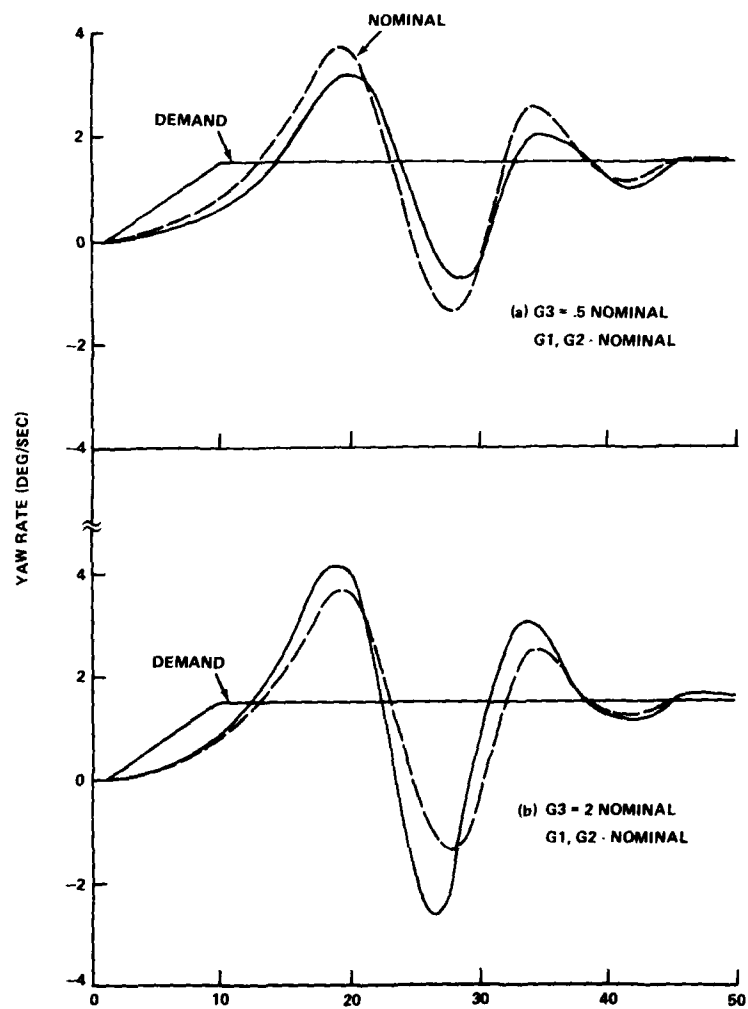
FIGURE 10. SENSITIVITY OF TURN RATE WITH RESPECT TO VARIATIONS IN G3 AT 50 kt
