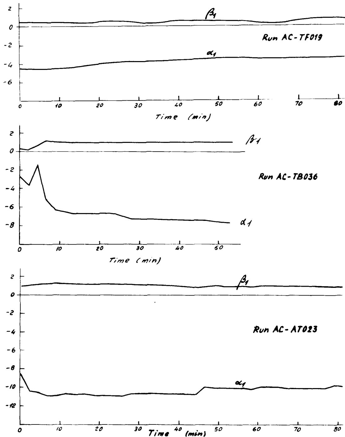
Figure 14: Model coefficients \alpha_1 and \beta_1 to show robustness of algorithm. Runs AC-TF 019 (tanker, full) AC - TB 036 (tanker, ballast) AC - AT 023 (containership).
