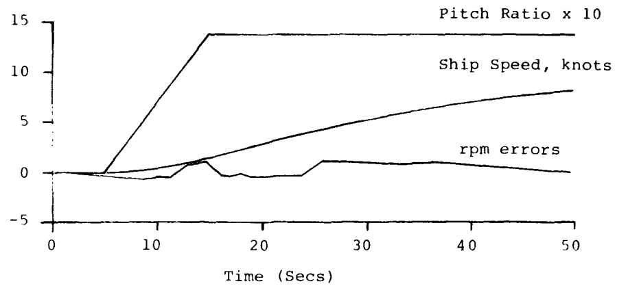
Figure 6. Plant Response, Weights (ii).
