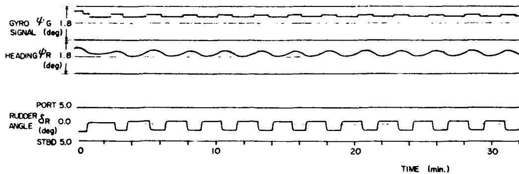
Fig. 5 Conventional APS at Calm Sea
