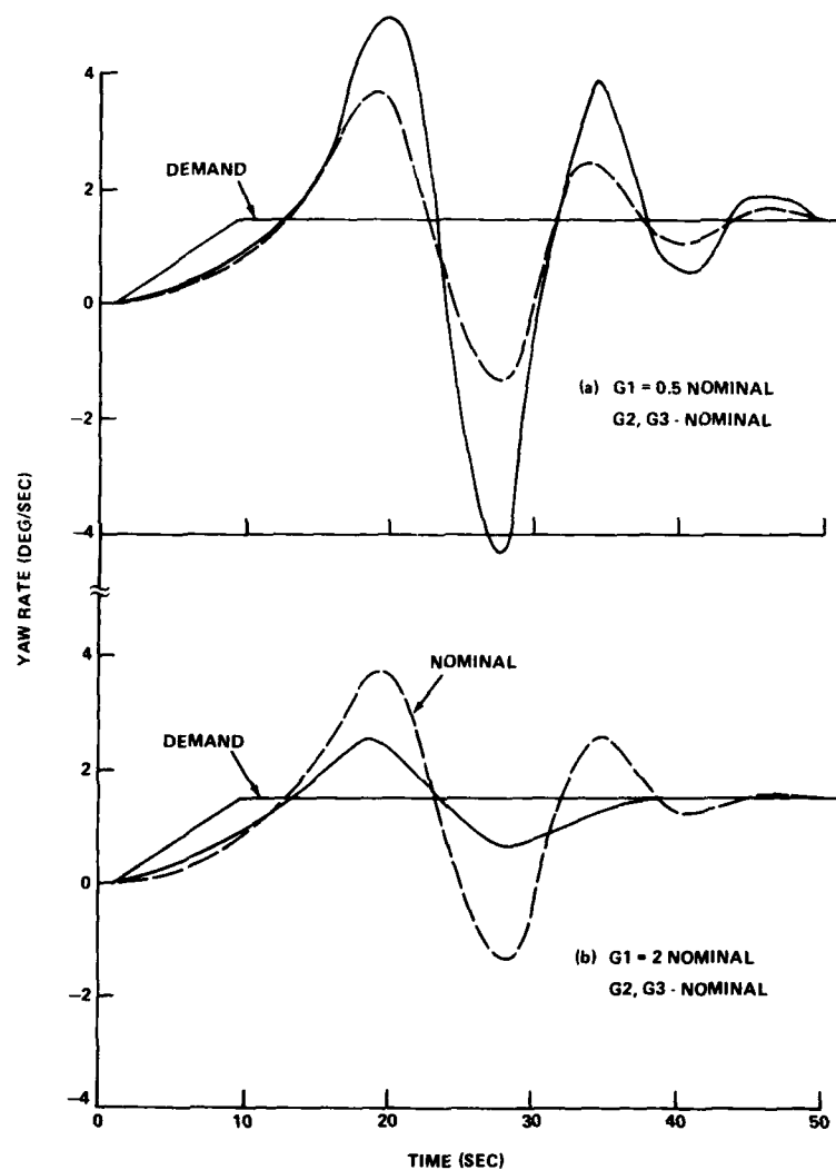
FIGURE 8. SENSITIVITY OF TURN RATE WITH RESPECT TO VARIATIONS IN G1 AT 50 kt
