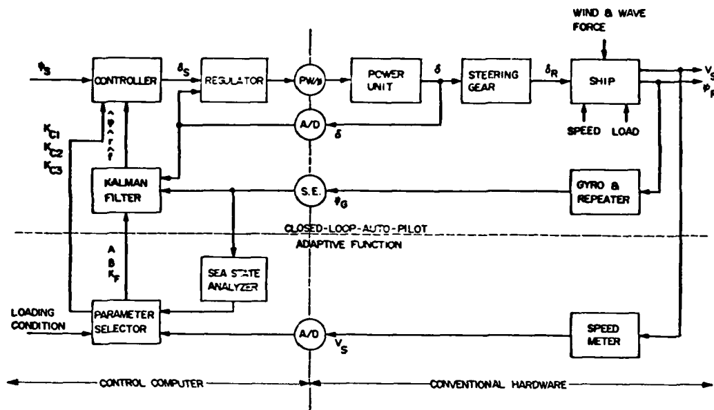
Fig. 2 Block Diagram of New Auto Pilot System
