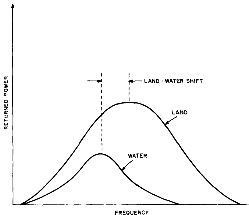
Figure 5. Doppler Frequency Spectrum for Land-Water Surfaces
