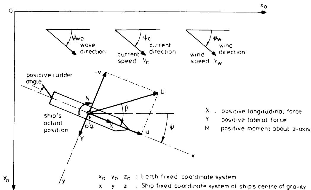
Figure 1: Coordinate systems and sign convention.
