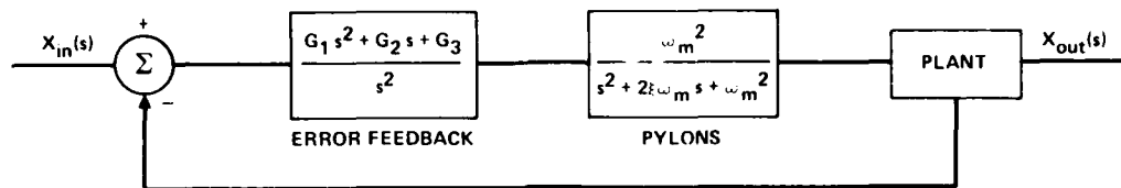
FIGURE 3. SCHEMATIC OF THE JEFF(A) AUTOMATIC CONTROL SYSTEM
