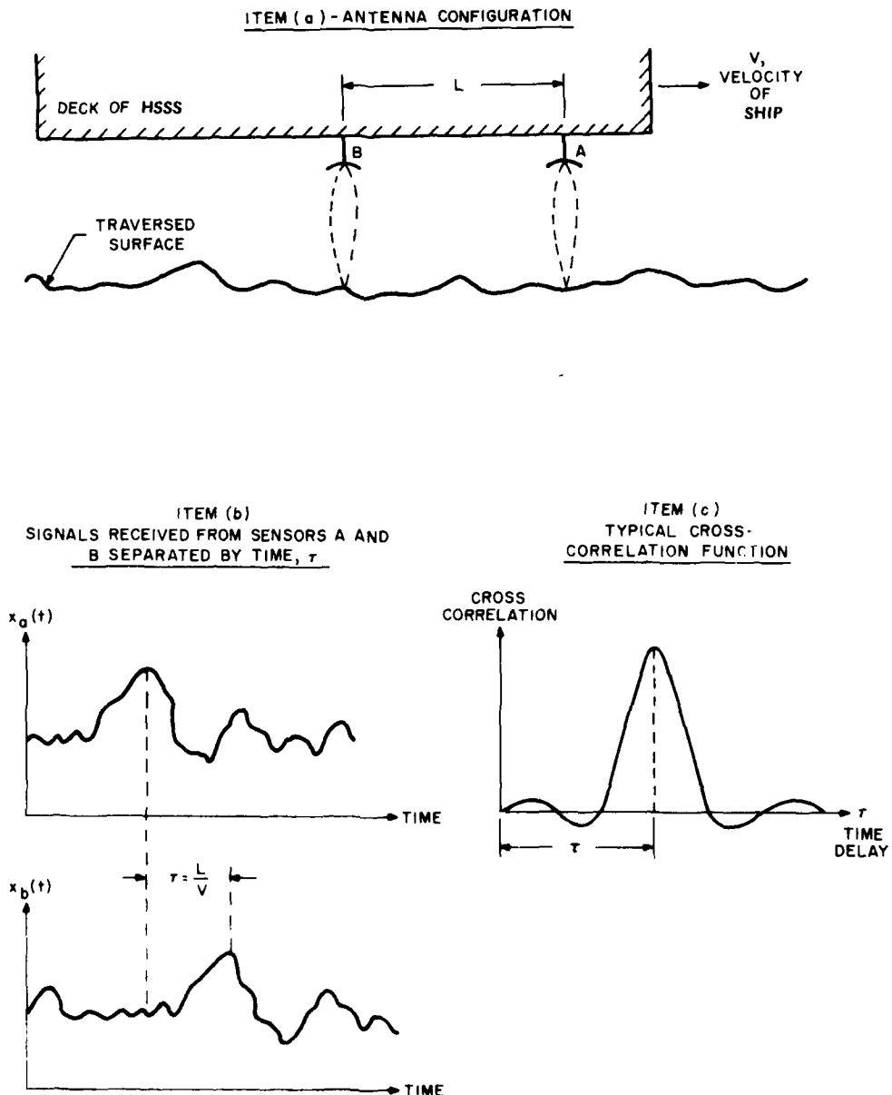
Figure 7. Cross-Correlation Speed Sensor
