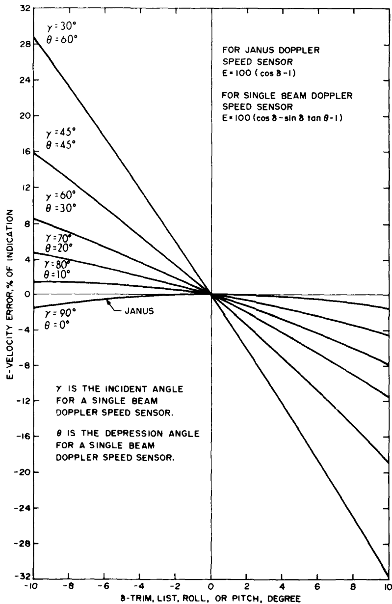
Figure 3. Velocity Error for Single Beam and Janus (Dual Beam) Doppler Sensors
