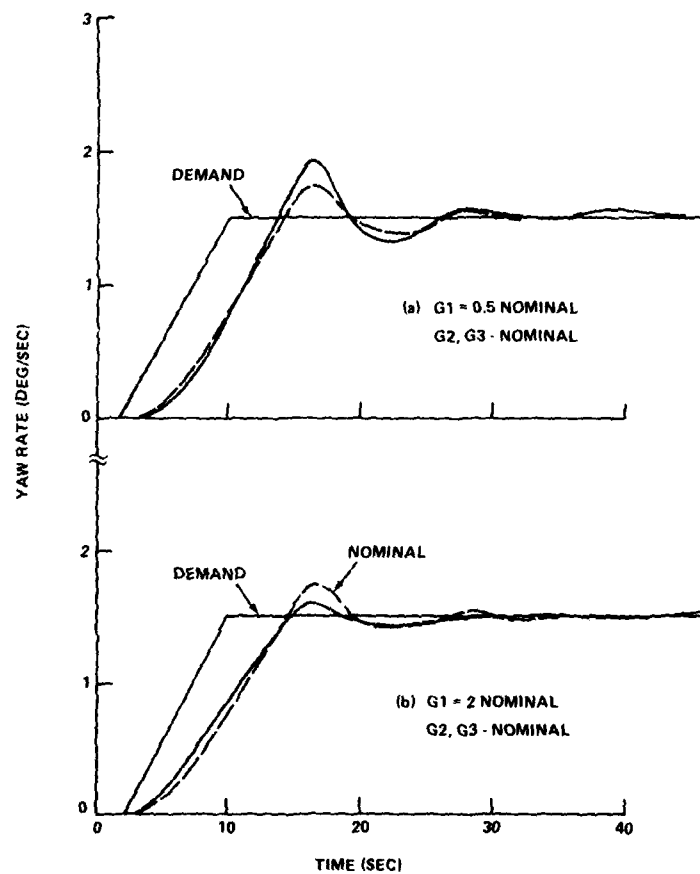
FIGURE 5. SENSITIVITY OF TURN RATE WITH RESPECT TO VARIATIONS IN G1 AT 40 kt
