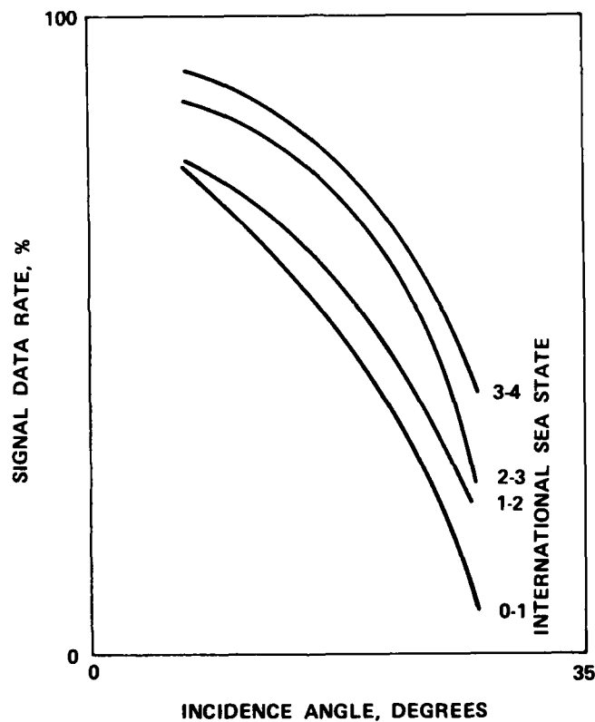
Figure 6. Illustrative Curves of Signal Data Rate for 10.6 Micron Laser as a Function of Incident Angle and Sea State
