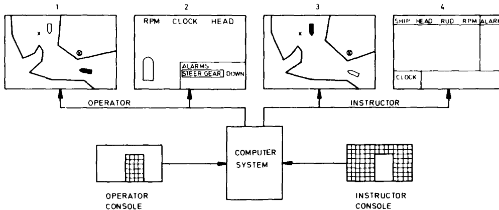
FIG. 7 Example of information on the four TV-screens in a collision study
