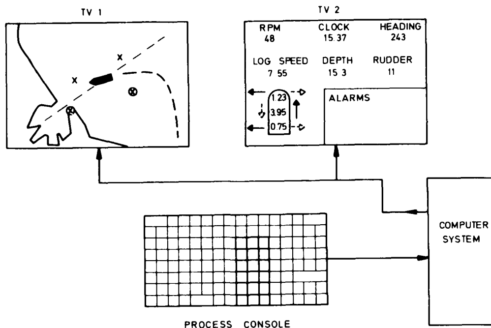
FIG. 5 The two main screens for SHIP 0
