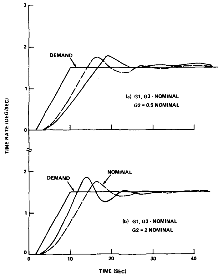
FIGURE 6. SENSITIVITY OF TURN RATE WITH RESPECT TO VARIATIONS IN G2 AT 40 kt
