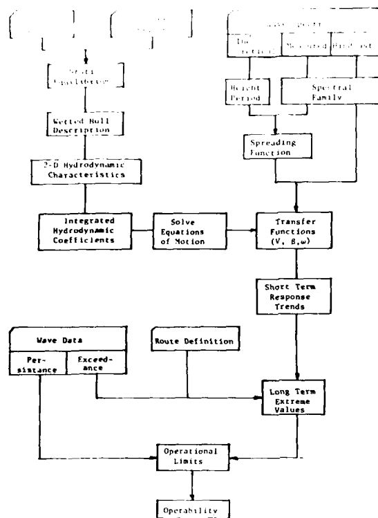
Figure 3. Typical Seakeeping Analysis Procedure.
