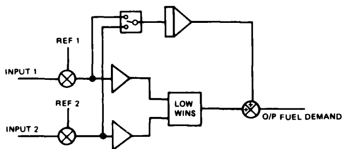
FIGURE 6 SINGLE INTEGRATOR CONTROLLER
