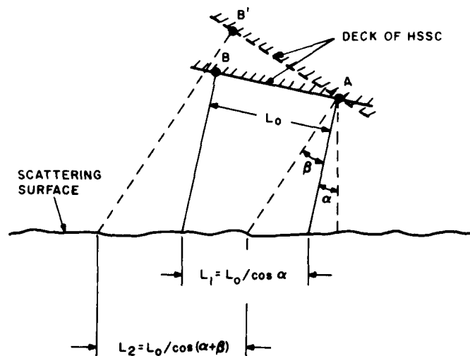
Figure 9. Beam Geometry for Cross-Correlation Speed Sensor
