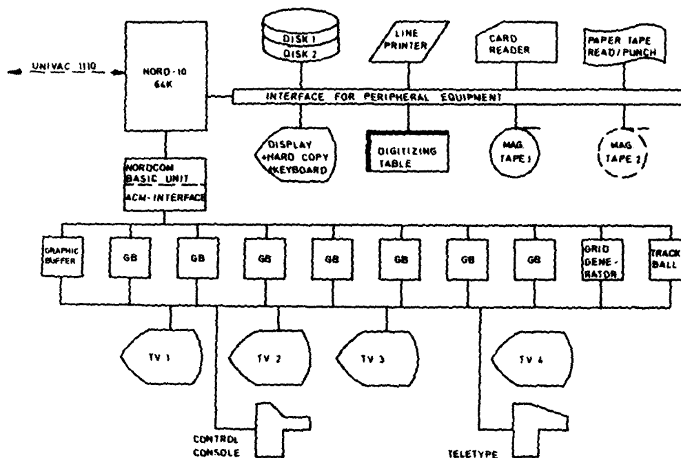
FIG. 1 The hardware configuration of GENSIM
