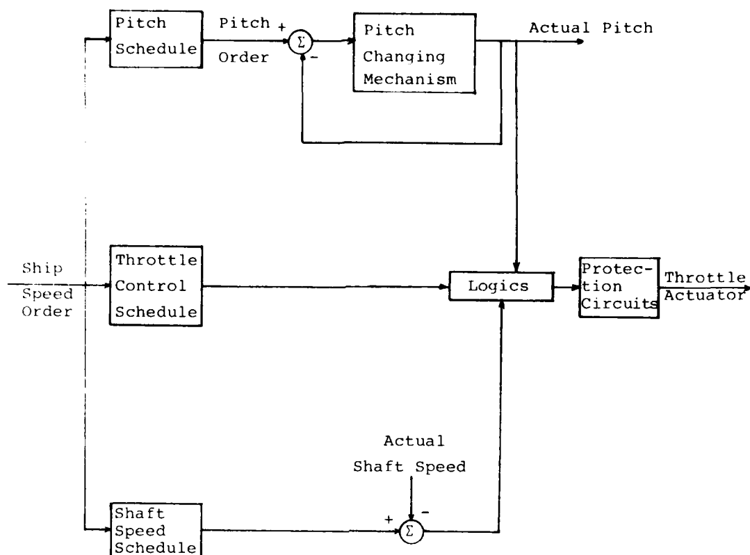
Figure 2. "Programmed Control" Structure.
