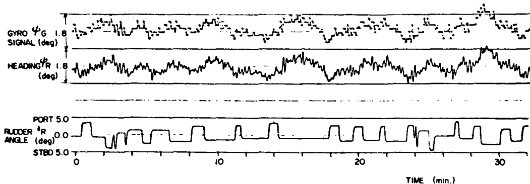
Fig. 8 Conventional APS with Weather Adjust at Heavy Sea
