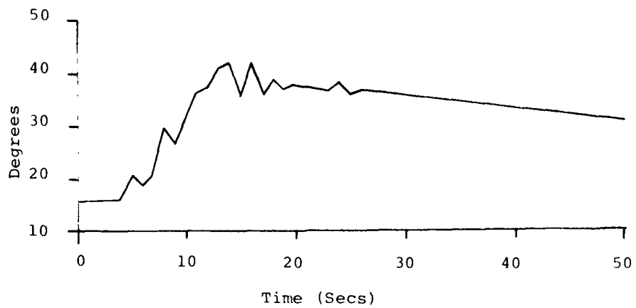
Figure 7. Throttle Control, Weights (ii).
