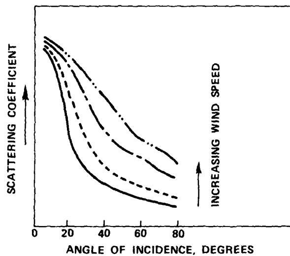
(a) Typical Scattering Coefficients for 1-3 cm Radar Over Water
