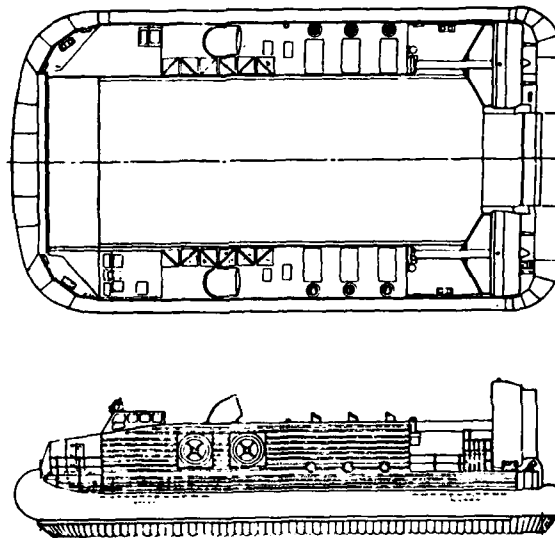
FIGURE 2. JEFF(B) LAYOUT
