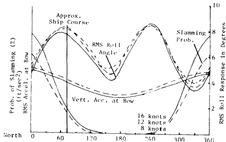
Figure 5. Variations of vertical acceleration at the bow, slamming probability and roll responses due to changes in heading and speed.
