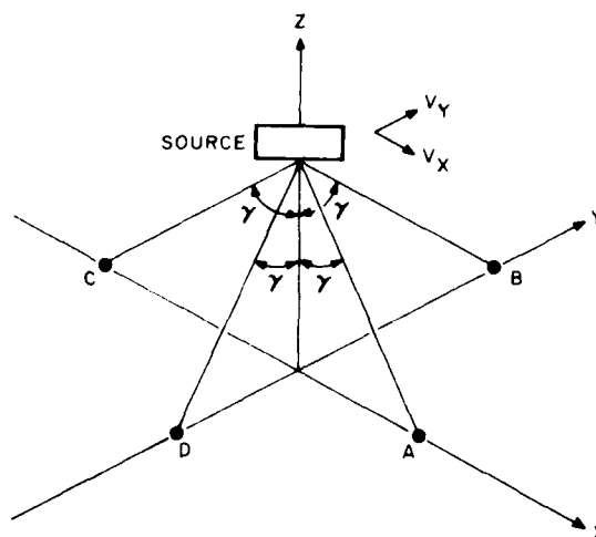
Figure 2. Geometry of a Janus Doppler System
