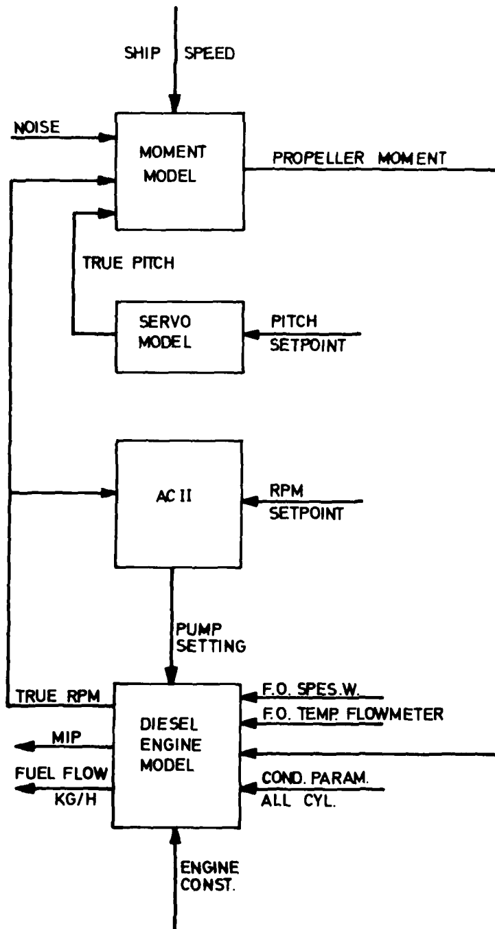
Fig. 3 SIMPLIFIED MODEL OF THE MAIN ENGINE MODEL.
