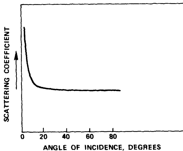
(b) Typical Scattering Coefficients for 1-3 cm Radar over Wet Partially Grassy Terrain
