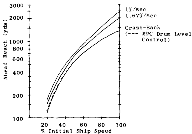
Figure 9. Ahead Reach For Crash-Back And Normal Throttle Valve Maneuvering Rates
