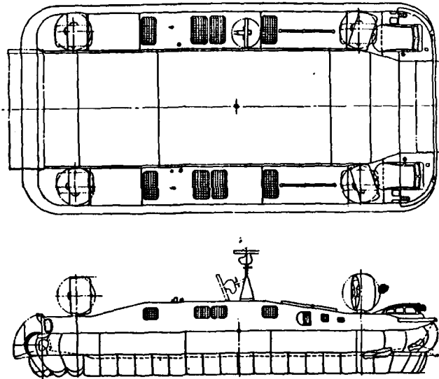
FIGURE 1. JEFF(A) LAYOUT
