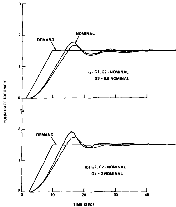
FIGURE 7. SENSITIVITY OF TURN RATE WITH RESPECT TO VARIATIONS IN G3 AT 40 kt
