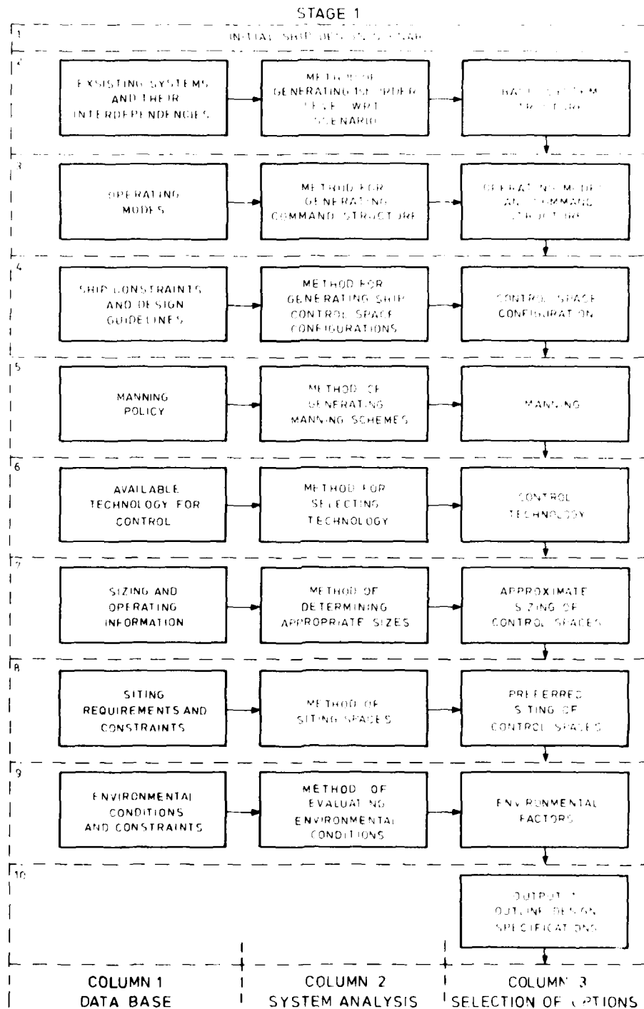
Figure 3 Design Algorithm
