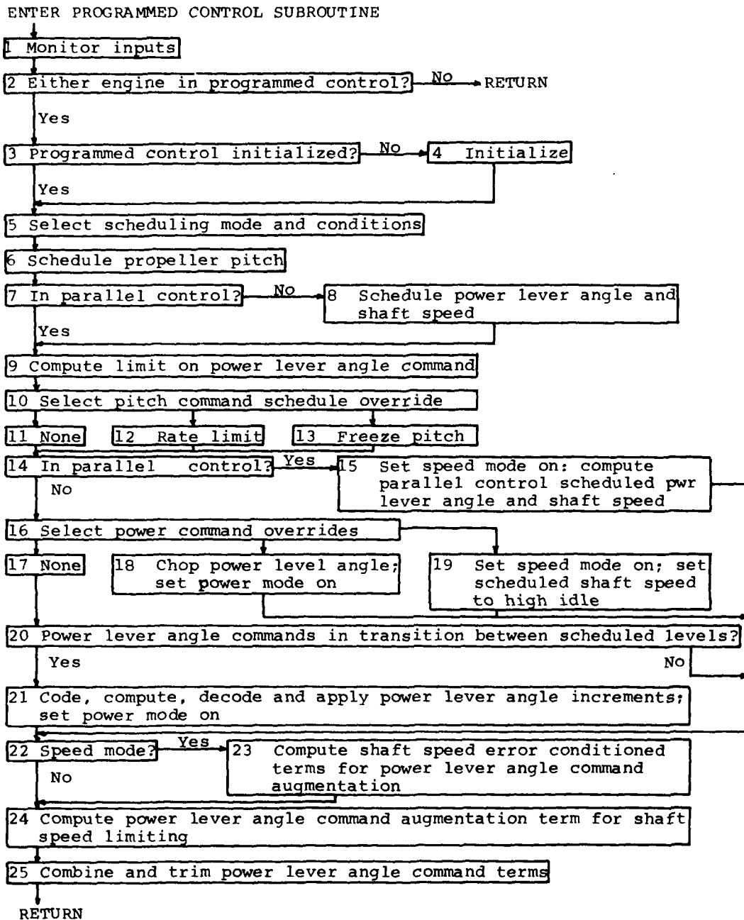
Figure 16-Programmed Control Subroutine
