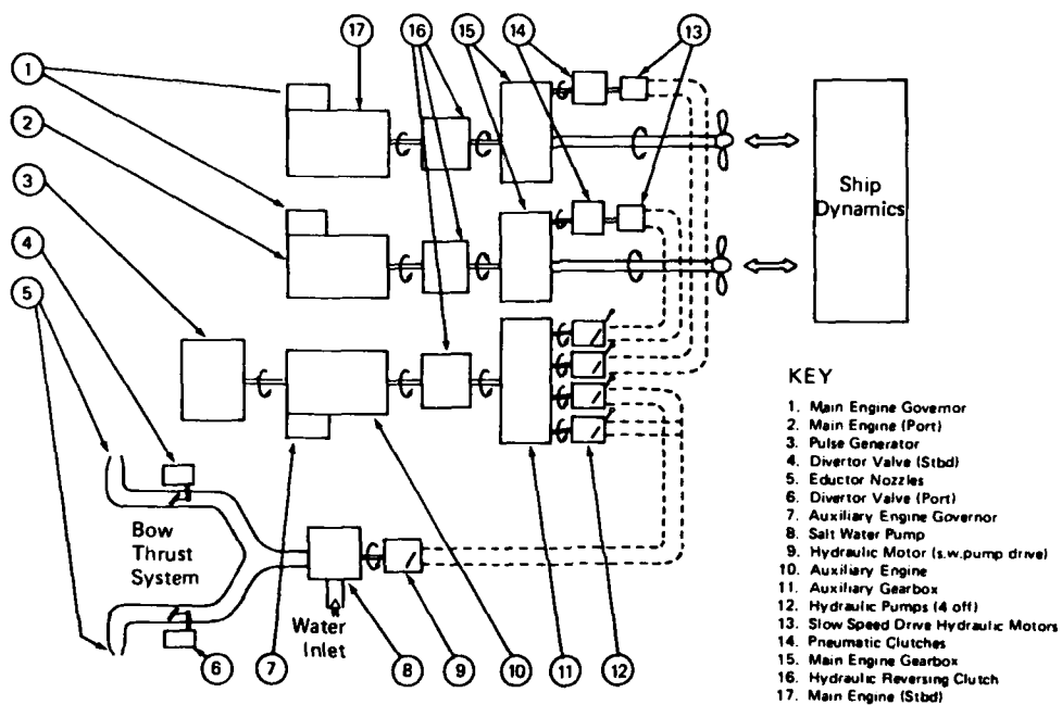
SCHEMATIC DIAGRAM OF PROPOSED MCMV PROPULSION MACHINERY
