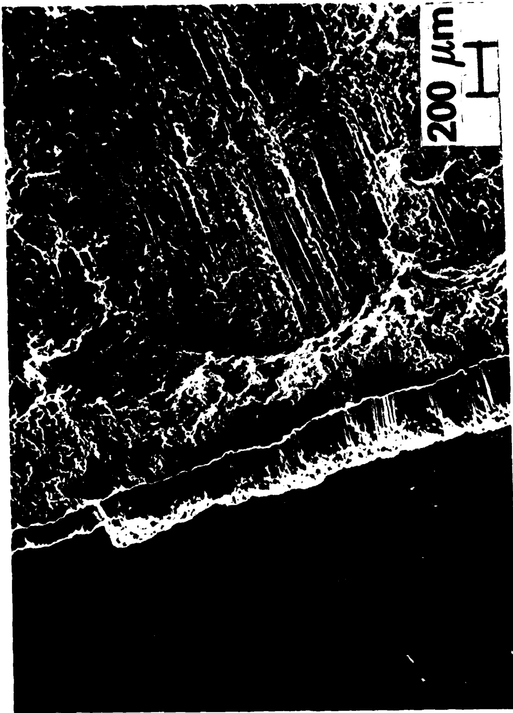
Fig. 3 — View of graphite fiber/magnesium composite after immersion in 0.001 N NaCl showing edge attack and exposure of graphite fibers.
