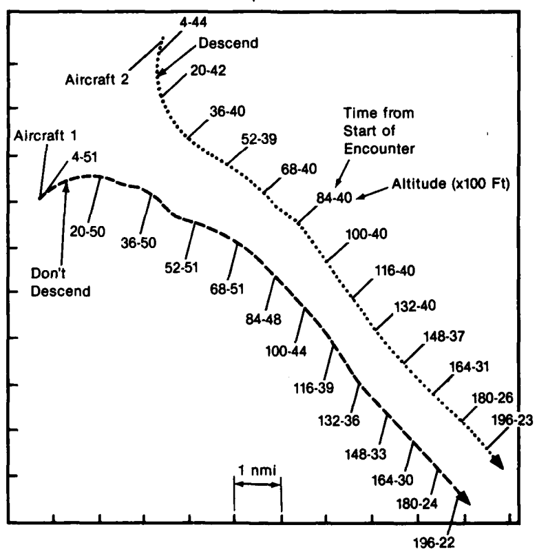
FIGURE E-1 VERTICAL AND PLAN-VIEW PLOTS OF ENCOUNTER 1
