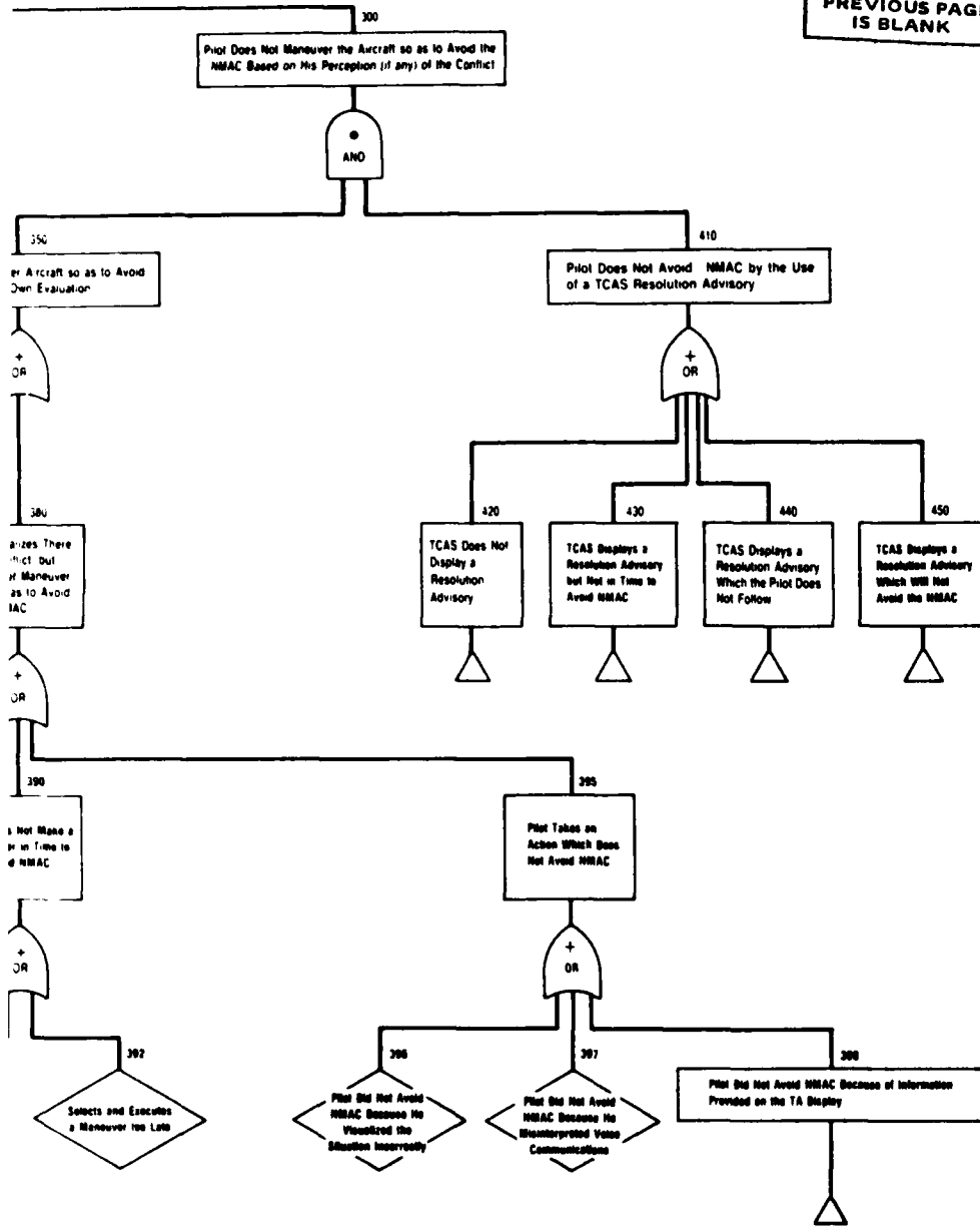
FIGURE D-3 000 BRANCH OF FAULT TREE FURTHER REDUCED FOR IMC
