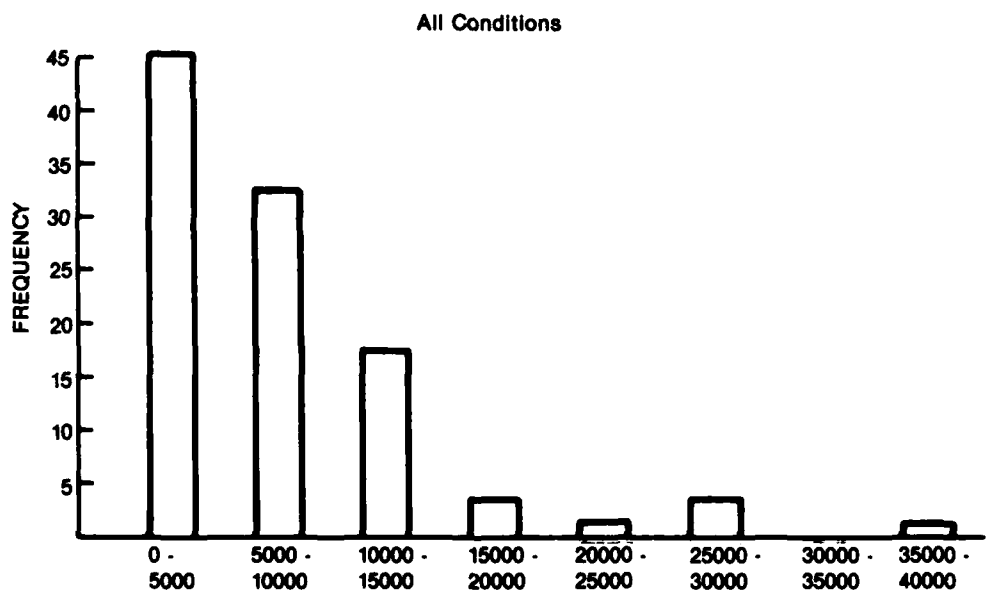
FIGURE 3-1 ALTITUDE DISTRIBUTION OF NMACs
