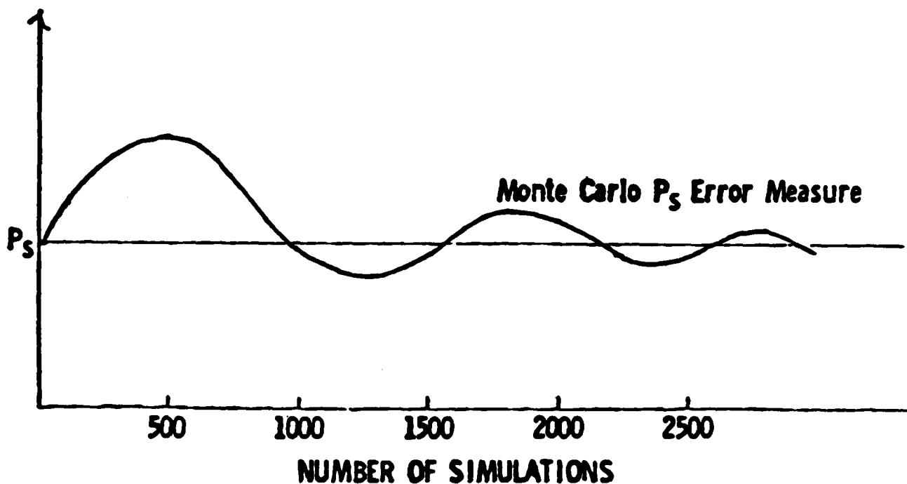
Figure 36. Additional criteria: convergence of 3rd and 4th moments.
