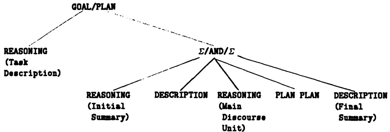
Figure 6: Top-level Structure of Boolean Level Stimulus
