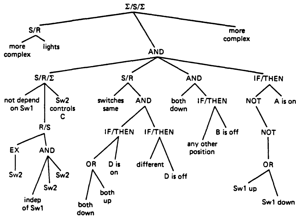
Figure 2: Structure Tree for a Reasoning Unit
