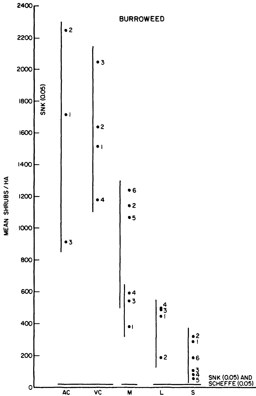
Figure 5. Intra- and intersite comparisons of burrowweed density.
