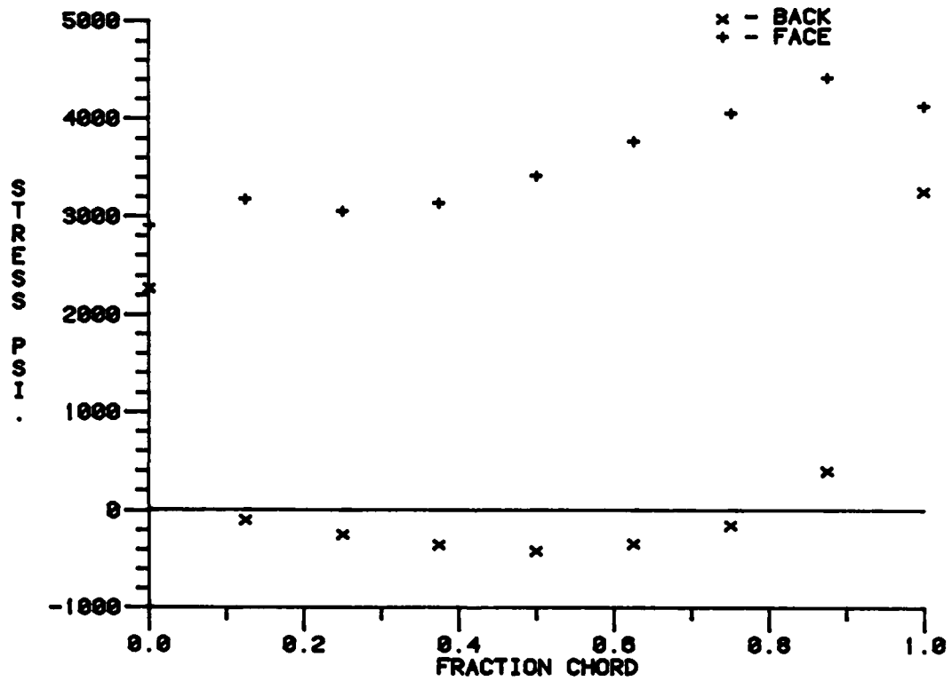
CHORDWISE DISTRIBUTION OF PRIMARY PRINCIPAL STRESSES
