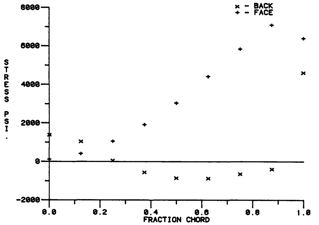
CHORDWISE DISTRIBUTION OF PRIMARY PRINCIPAL STRESSES
