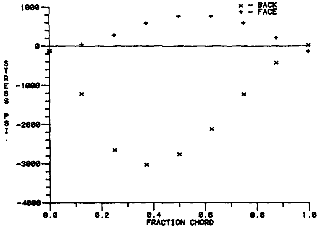
CHORDWISE DISTRIBUTION OF SECONDARY PRINCIPAL STRESSES
