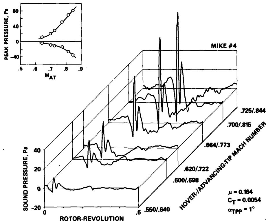
Figure 15.- Effect of blade-tip Mach number.
