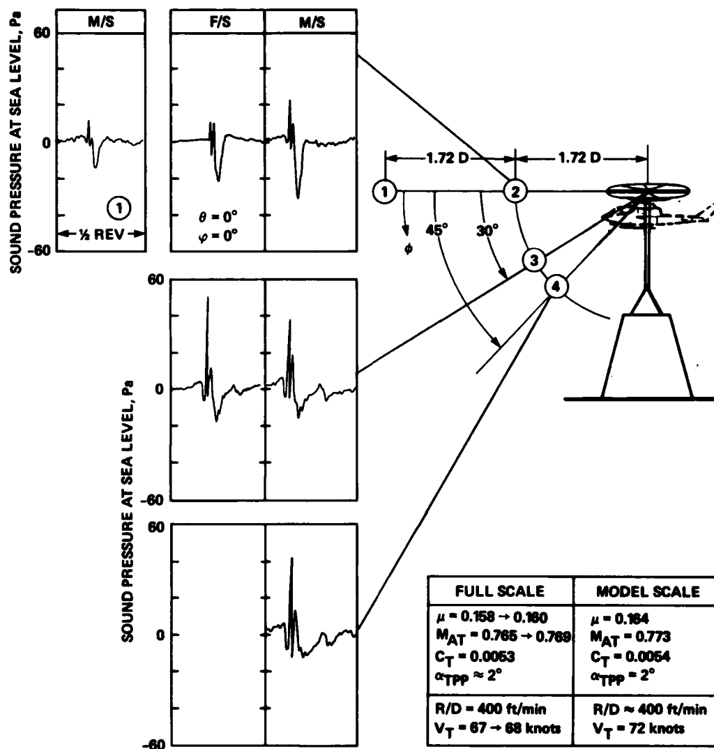
(a) Longitudinal directivity.
