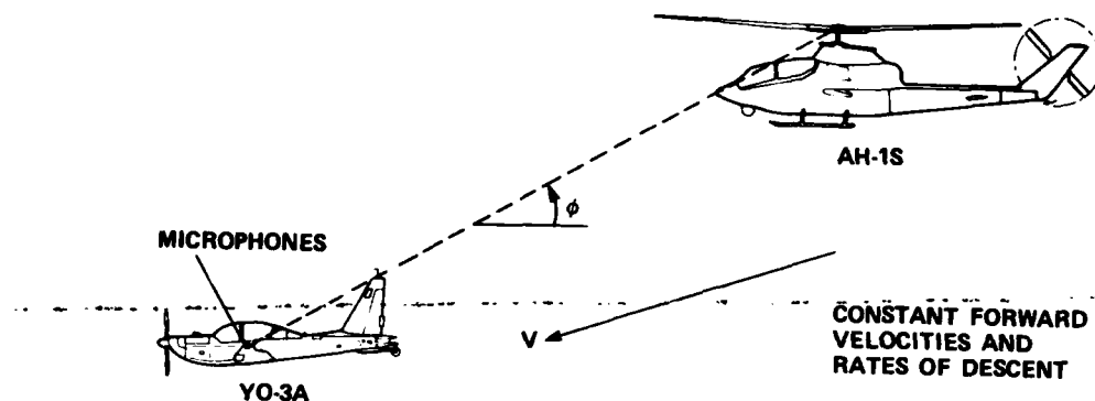
Figure 1.- Full-scale blade-vortex interaction acoustic measurement technique.
