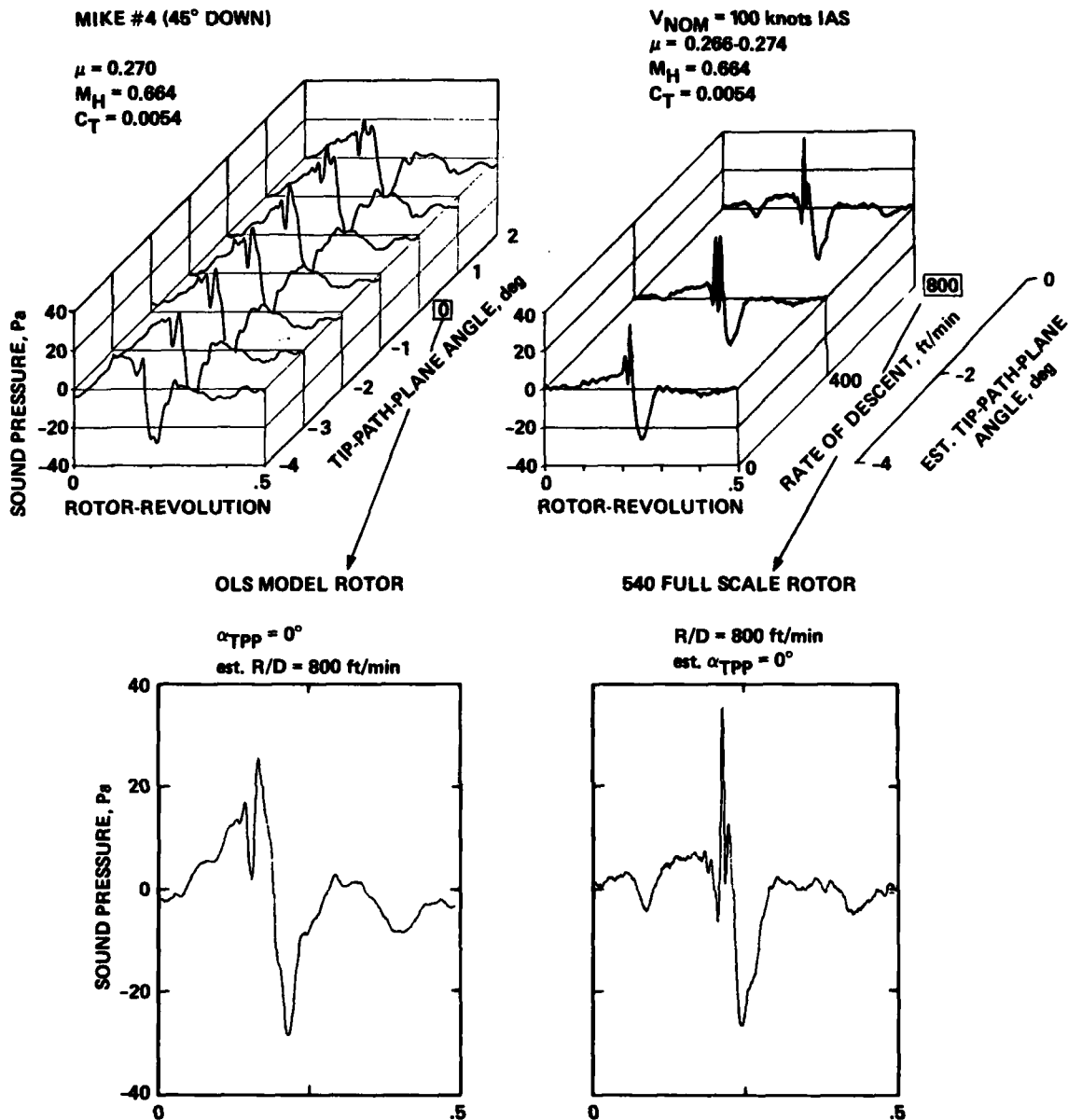
Figure 12.- Comparison of model-scale and full-scale acoustic data. Top: sweep of tip-path-plane angle or rate of descent; bottom: waveform comparisons of most intense interaction. \mu = 0.270 .
