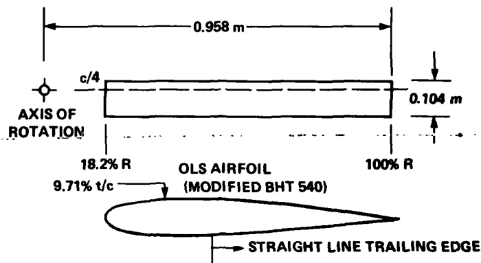
Figure 4.- OLS blade characteristics.
