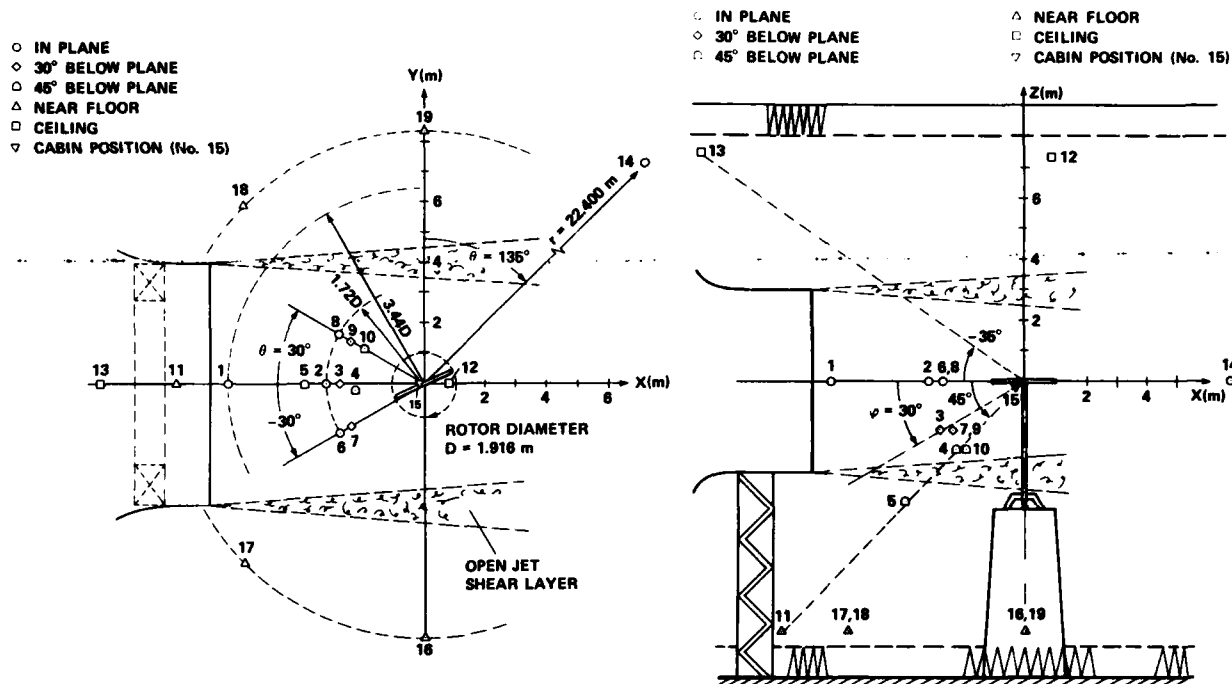
Figure 3.- Microphone locations in the DNW.
