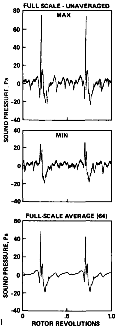
Figure 7.- Comparison of unaveraged and averaged sound pressure time-histories for one rotor revolution. (a) Full-scale (540) rotor; (b) model-scale OLS rotor.
