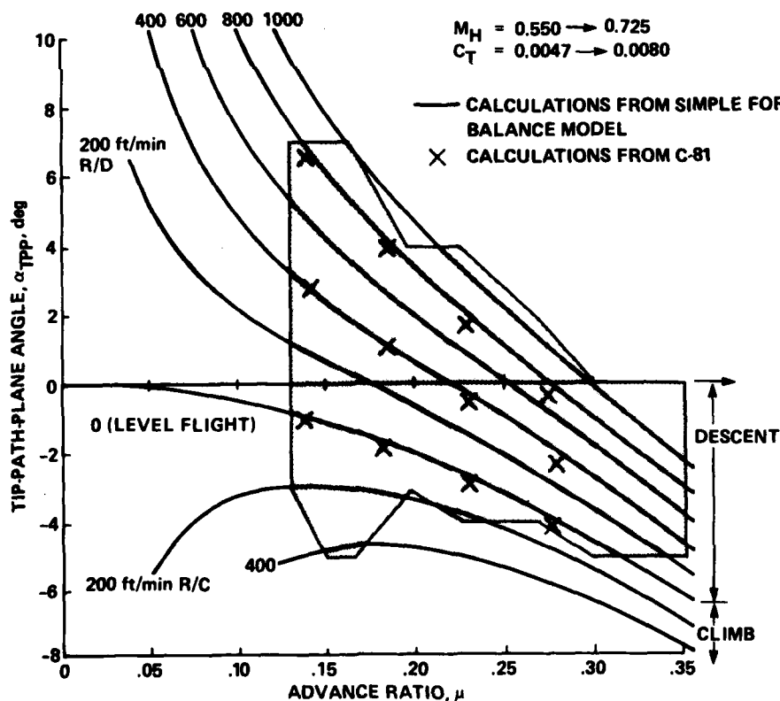
Figure 6.- OLS model testing envelope.
