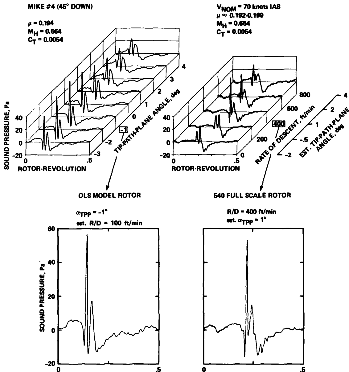
Figure 10.- Comparisons of model-scale and full-scale acoustic data. Top: sweep of tip-path-plane angle or rate of descent; bottom: waveform comparisons of most intense interaction. \mu = 0.194 .
