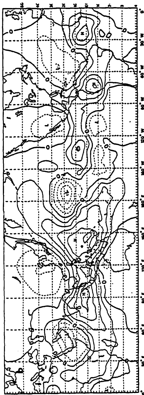
Fig. 15 As Fig. 1 except for the period 14-18 Dec 1984.
