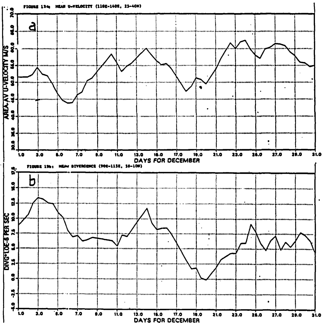
Fig. 13a As in Fig. 11a except for the East Asia-western Pacific region (EA) ( 110^{\circ}\text{E} , 25^{\circ}\text{N} )
