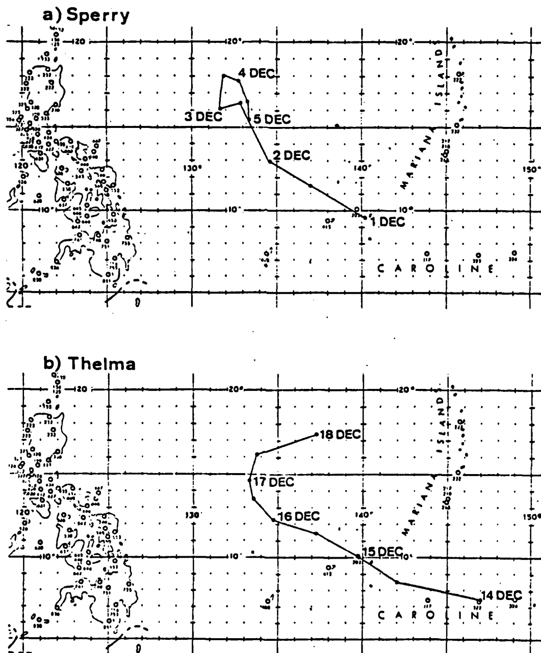
Fig. 14 Storm tracks for (a) Sperry and (b) Thelma 1983.
