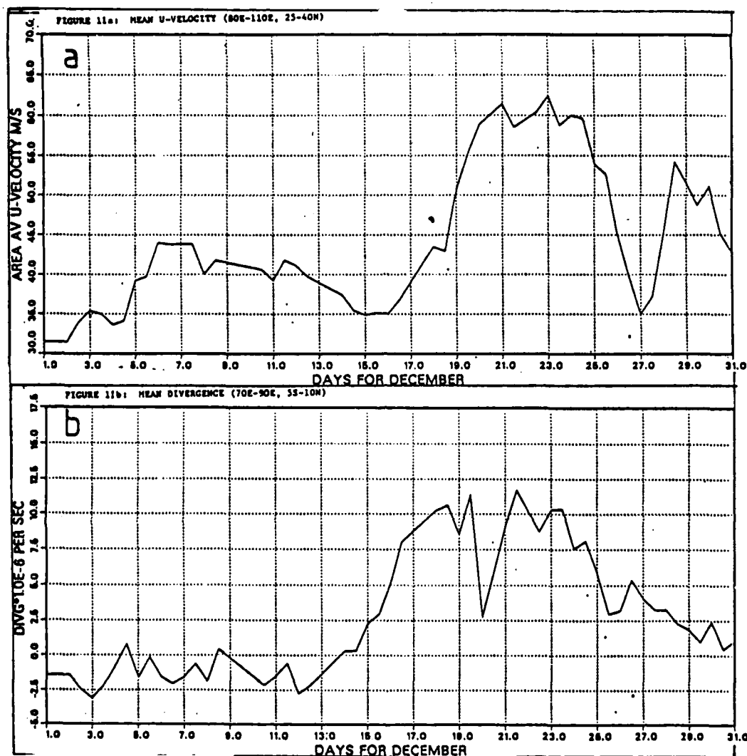
Fig. 11a Time series of area-averaged zonal velocity for the Tibetan Plateau region, (TP) ( 80^{\circ} - 110^{\circ} E, 25^{\circ} N- 40^{\circ} N)
