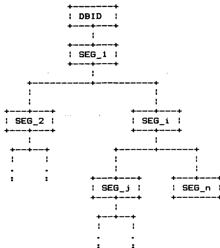
Figure 16. The Hierarchical Database Schema.
