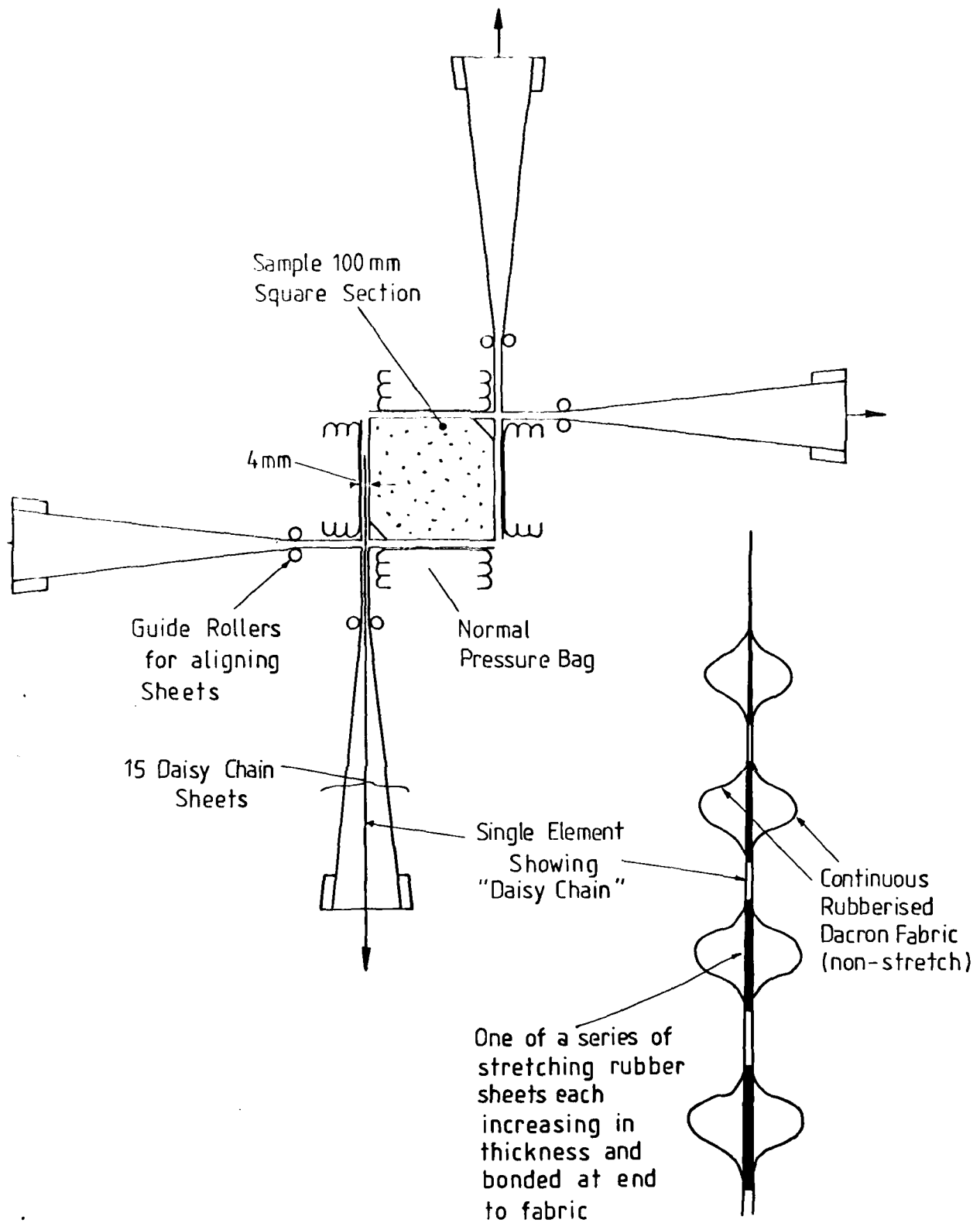
Principle of New Wide Stress Range Shear Sheets
