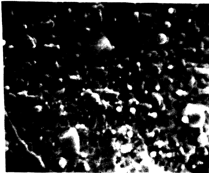
Figure B.15 Target A (X 2000) Area Sevefely Damaged by Arcing (Note Debris).
