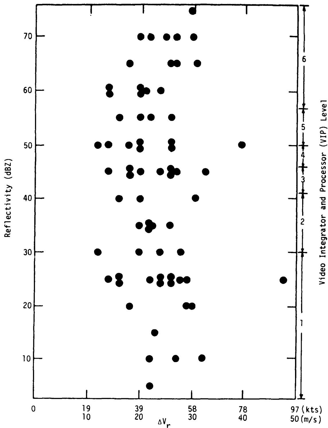
Figure 2.9. Plot of maximum radar reflectivity near the surface (echo intensity) as a function of maximum velocity differential). Serious low-altitude microburst wind shear can occur in a wide range of convective intensity, from non-thunderstorm (reflectivities generally less than 30 dBZ) to intense thunderstorms (reflectivities greater than 50 dBZ).
