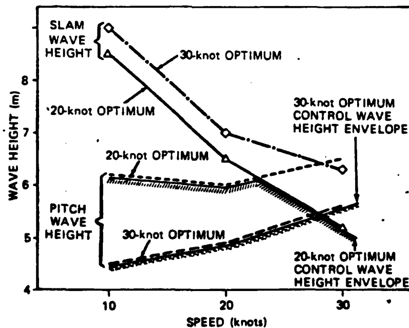
Figure 11 - Limiting Wave Height versus Ship Speed
