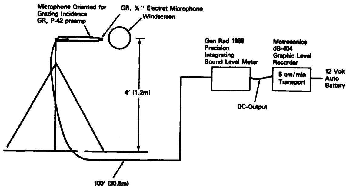
Direct Read Noise Measurement System
