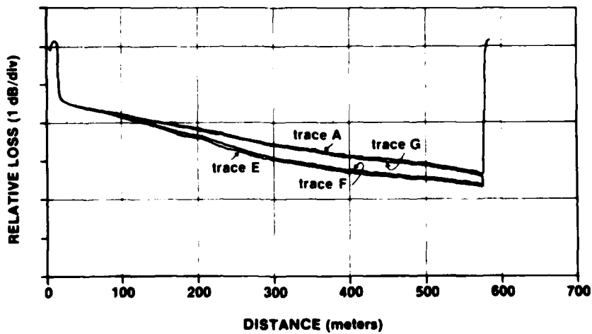
Figure 17. OTDR measurements: traces A, E, F, and G.
