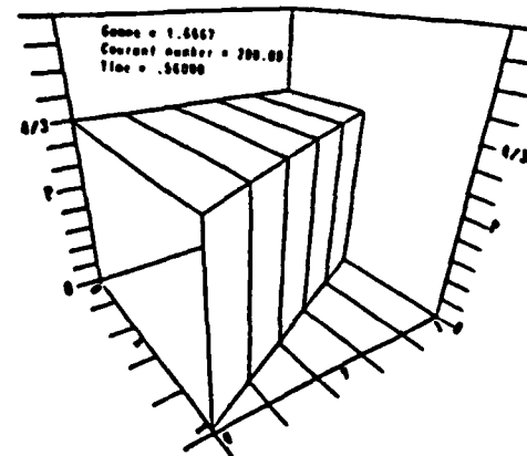
FIG.9, INFINITE 2D PLANAR SHOCK, \gamma = 5/3
