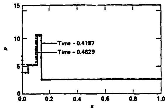
FIG.5, COLLIDING WAVES(STEP-UP), \gamma = 5/3
