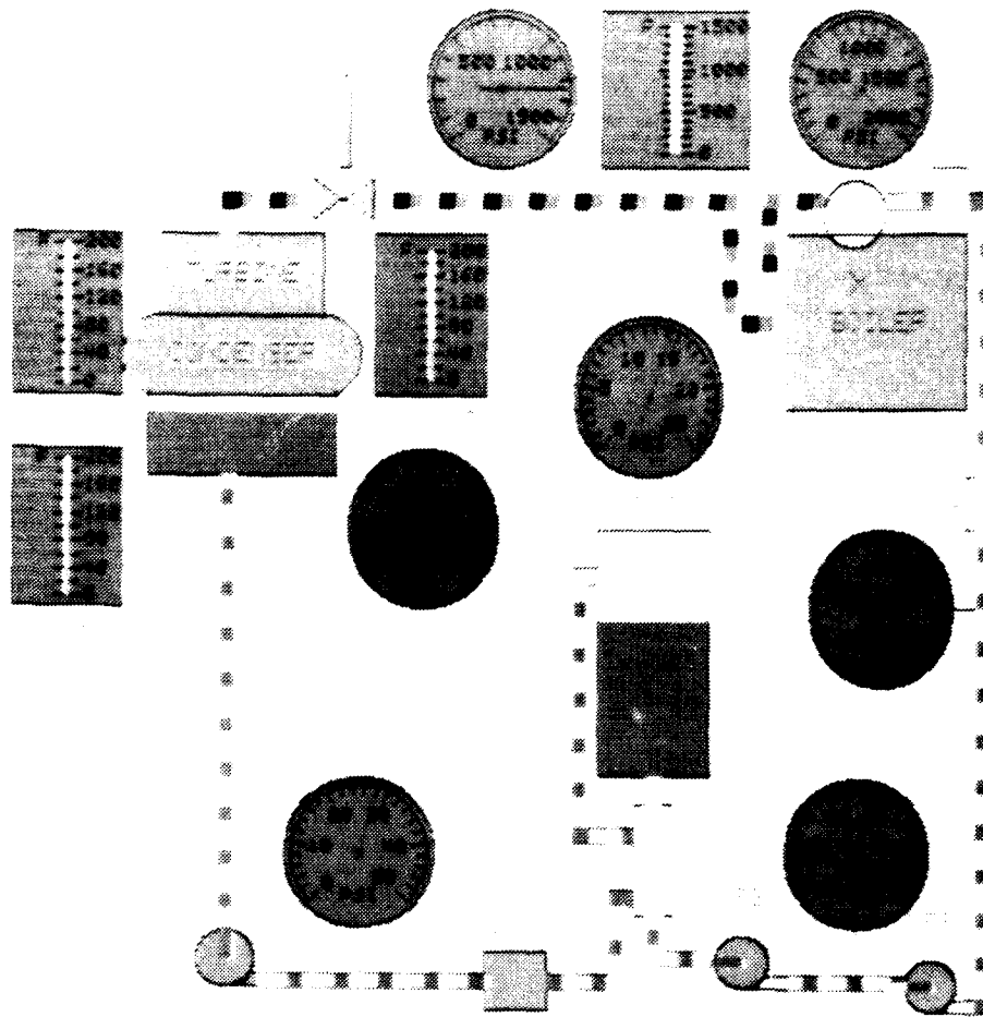
FIGURE A-2 STEAMER: A simulator with low physical fidelity and high training capability.
