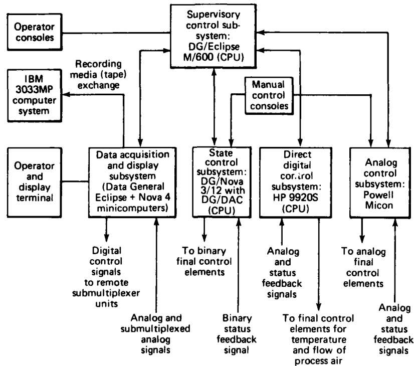
Figure 9 —PRL instrumentation and control system for automated testing in the IR Seeker Aerothermal Test Facility.
