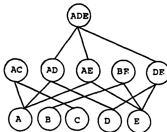
situation lattice
