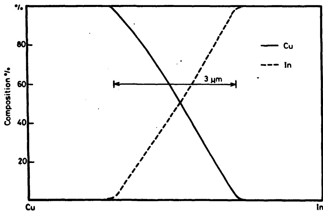
Fig. 5.4 MICROPROBE ANALYSIS OF INDIUM FILM DEPOSITED AT 40 MICRONS OF ARGON PRESSURE ON COPPER SUBSTRATE (QUALITATIVE)
