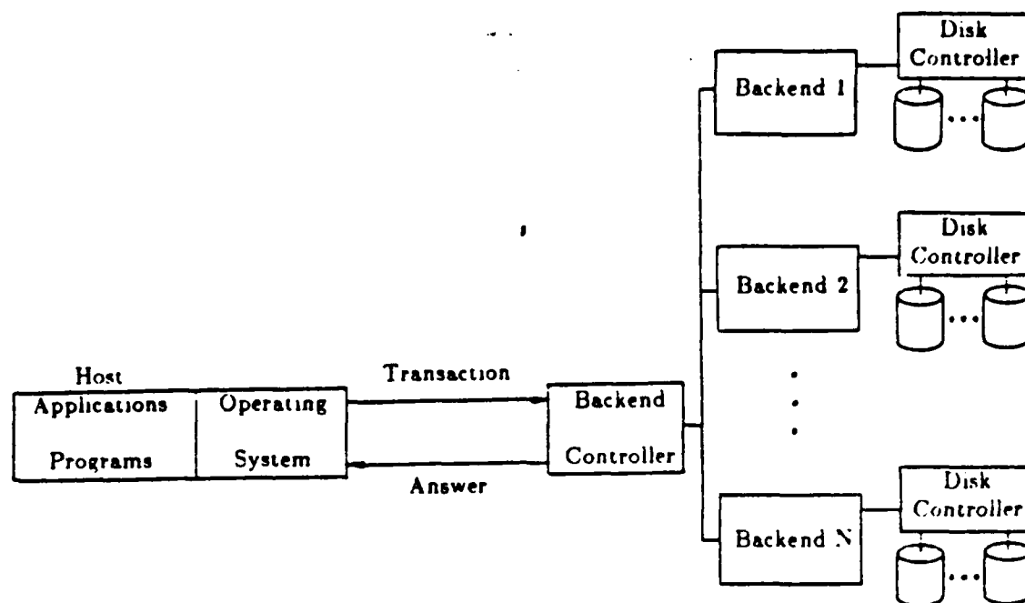
Figure 3. The Software Multiple-Backend Approach.
