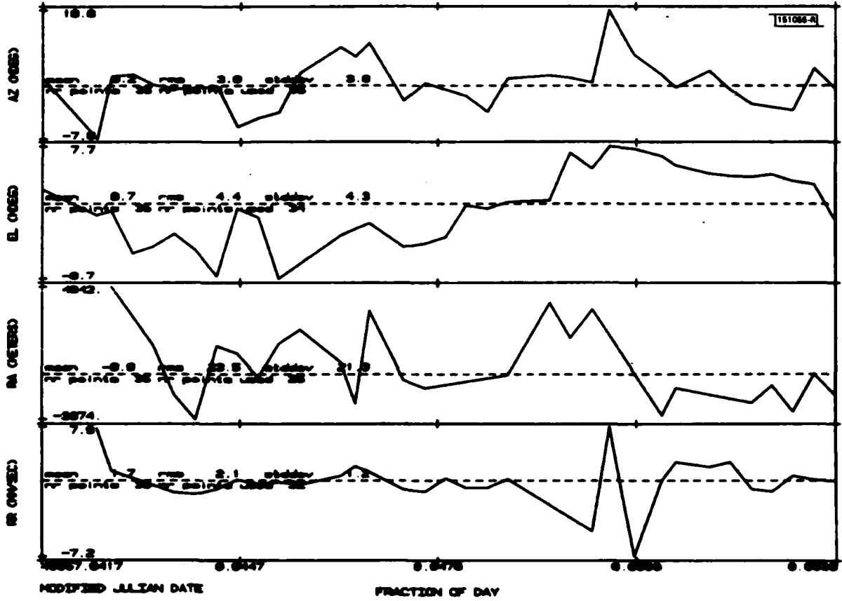
Fig. 2C. Millstone Hill Radar residuals laser reference orbit.
