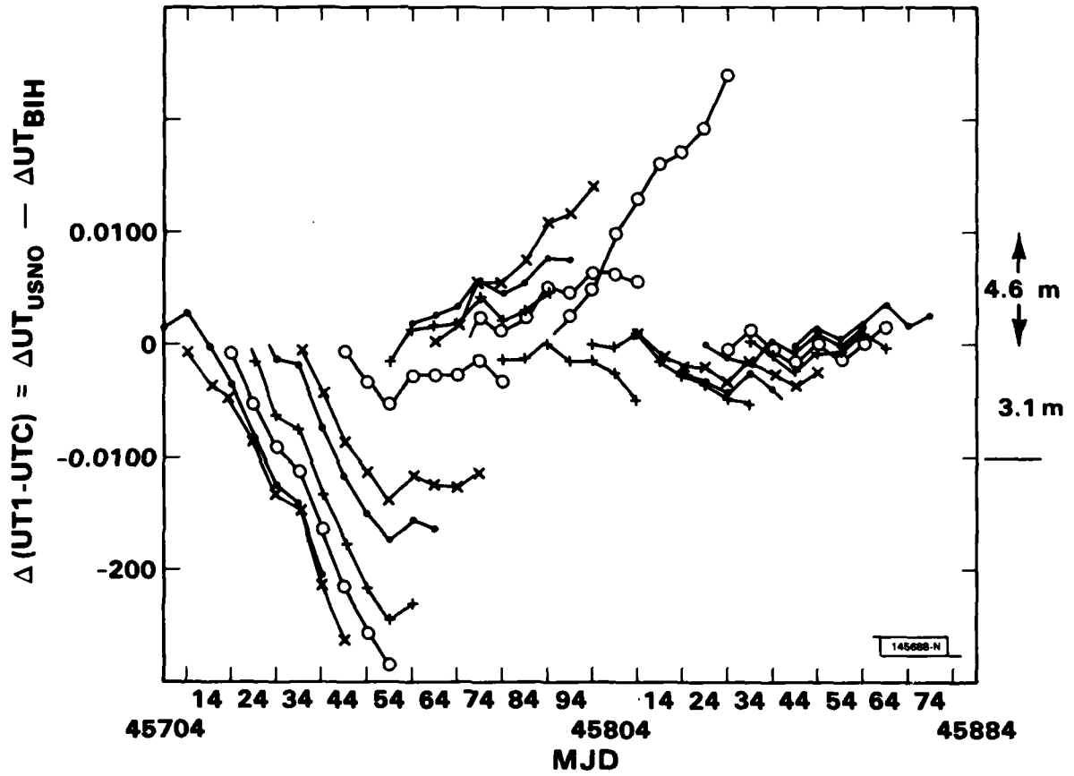
Fig. 8. UT1 prediction.
