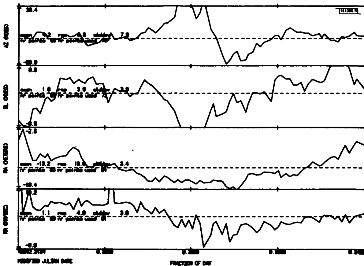
Fig. 2M. Millstone Hill Radar residuals laser reference orbit.
