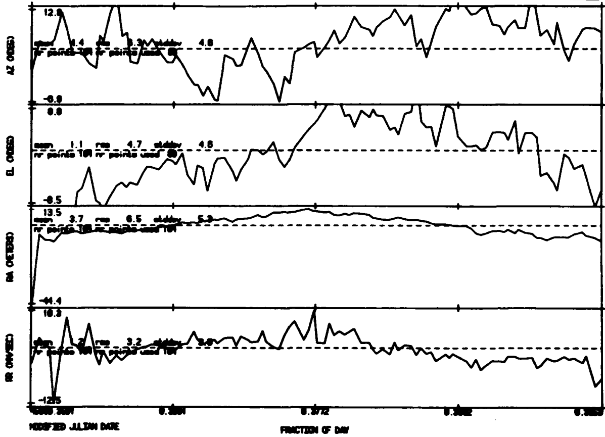
Fig. 2I. Millstone Hill Radar residuals laser reference orbit.
