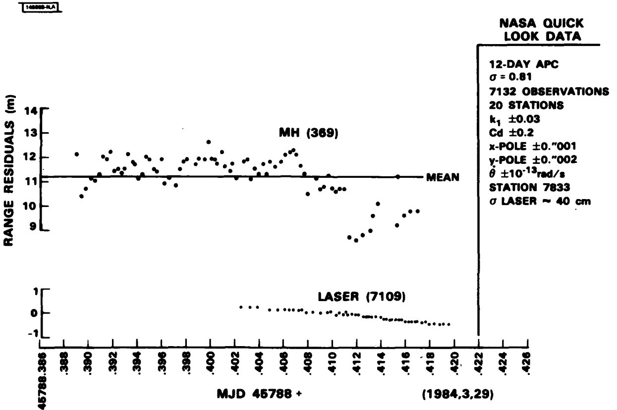
Fig. 4. Orbital residuals.
