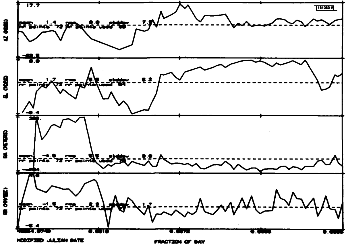
Fig. 2A. Millstone Hill Radar residuals laser reference orbit.
