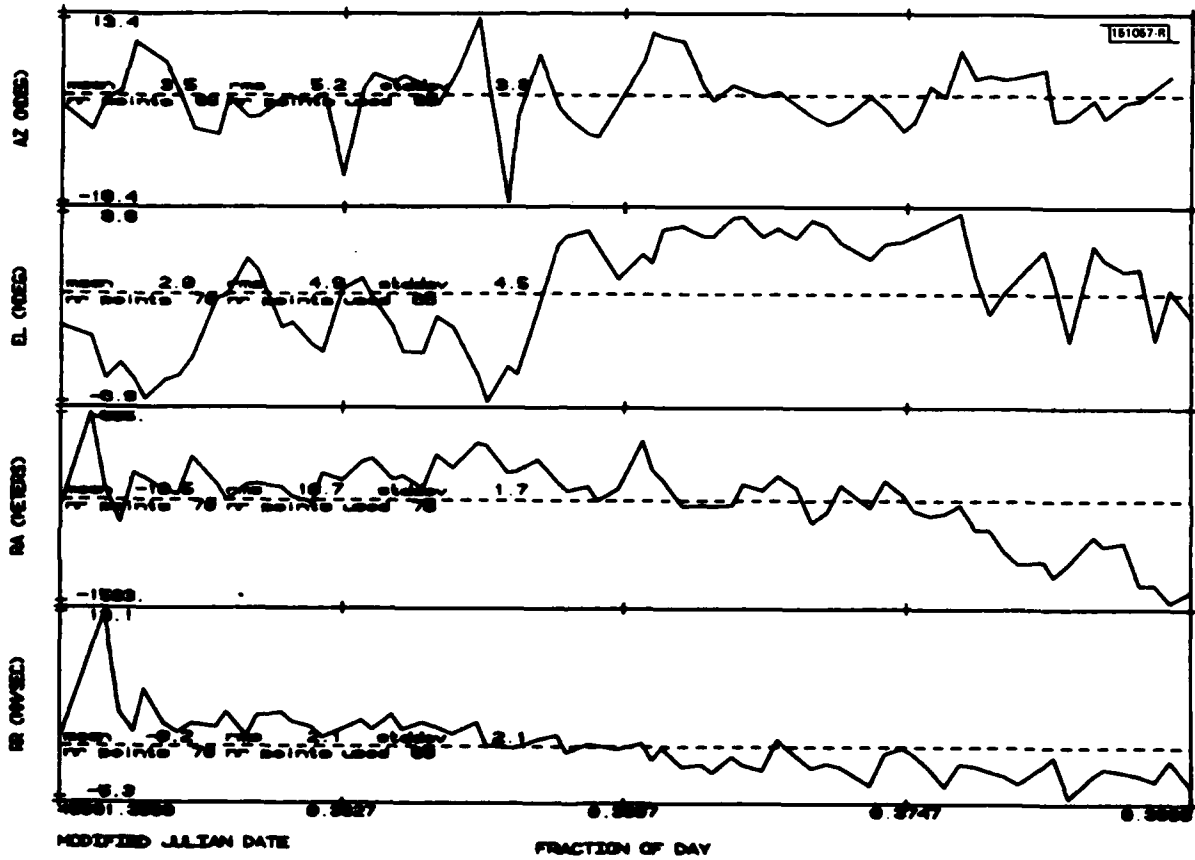
Fig. 2E. Millstone Hill Radar residuals laser reference orbit.
