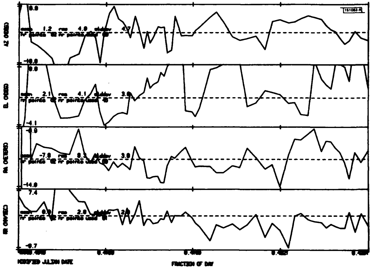
Fig. 2K. Millstone Hill Radar residuals laser reference orbit.
