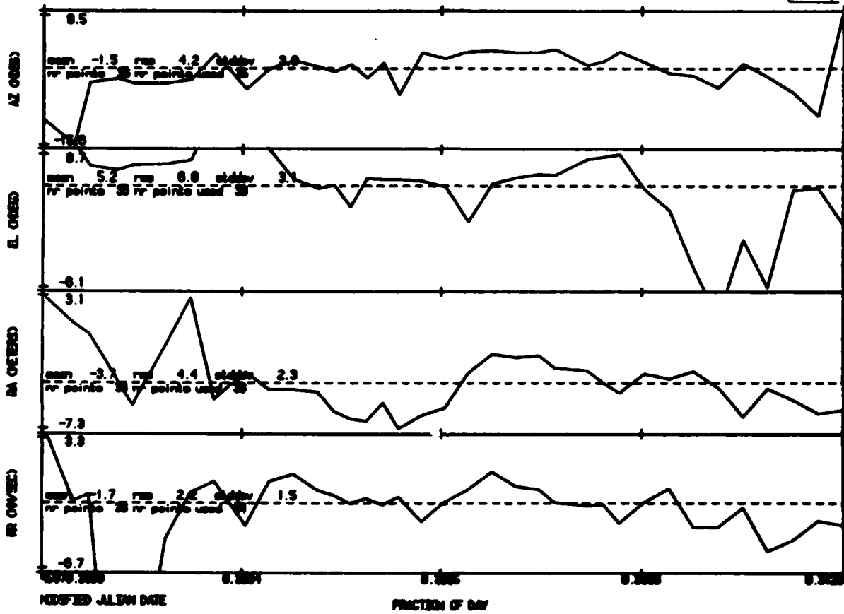
Fig. 2L. Millstone Hill Radar residuals laser reference orbit.
