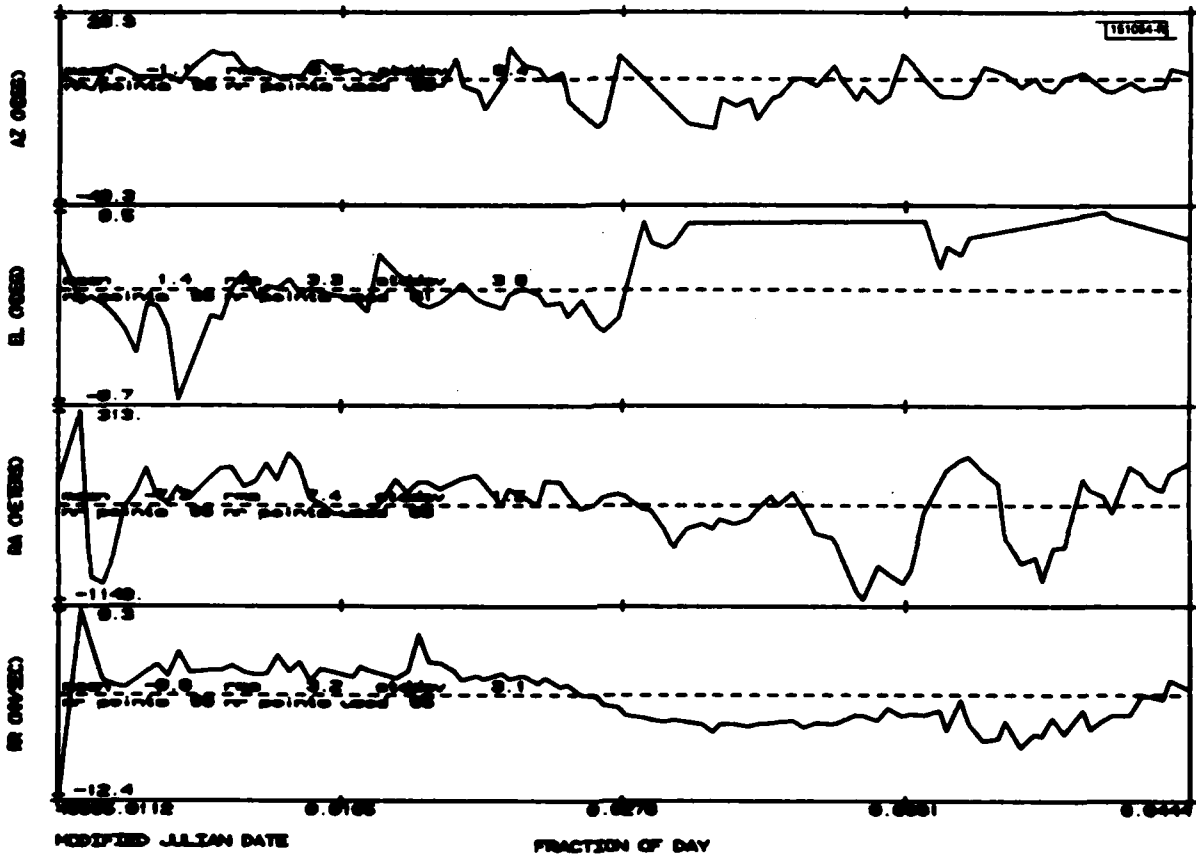
Fig. 2B. Millstone Hill Radar residuals laser reference orbit.
