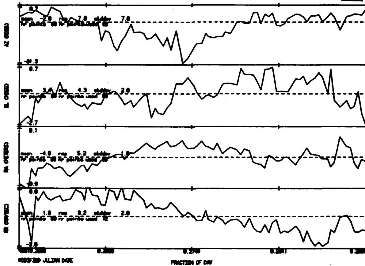
Fig. 2N. Millstone Hill Radar residuals laser reference orbit.
