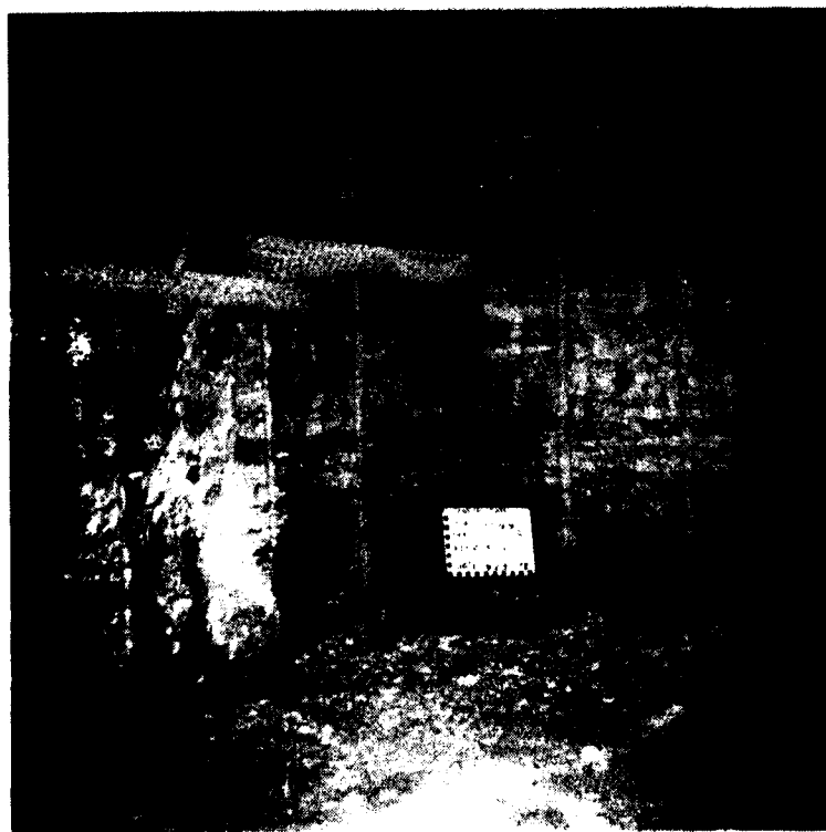
Cutoff wall, final foundation for concrete placement CW 1-3. Station 19+99, Elevation 570 feet. 23 Sept. 1978.
