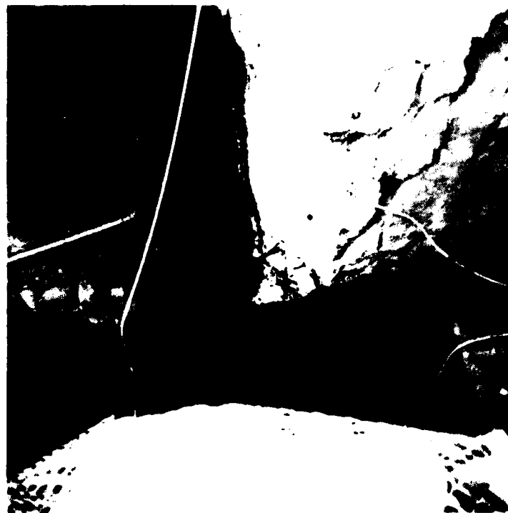
Left abutment cutoff wall, cavity #6, Station 19+00, Offset upstream, Elevation 580 feet. 12 Oct. 1978.
