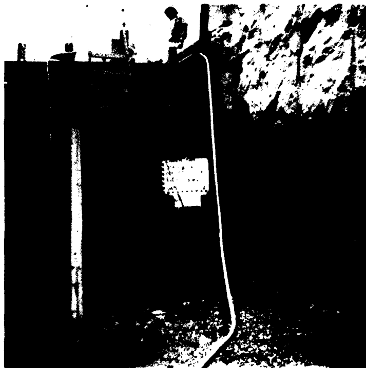
Cutoff wall, final foundation for concrete placement CW 2-5. Station 19+40, Offset upstream, Elevation 590 feet. 11 Oct. 1978.
