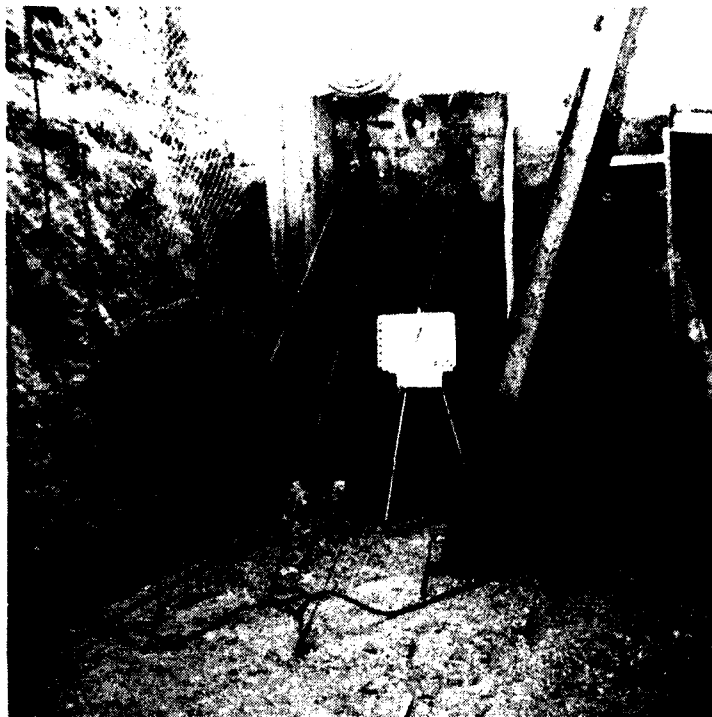
Cutoff wall, final foundation for concrete placement CW 4-4. Station 18+80, Offset downstream, Elevation 580 feet. 12 Oct. 1978.
