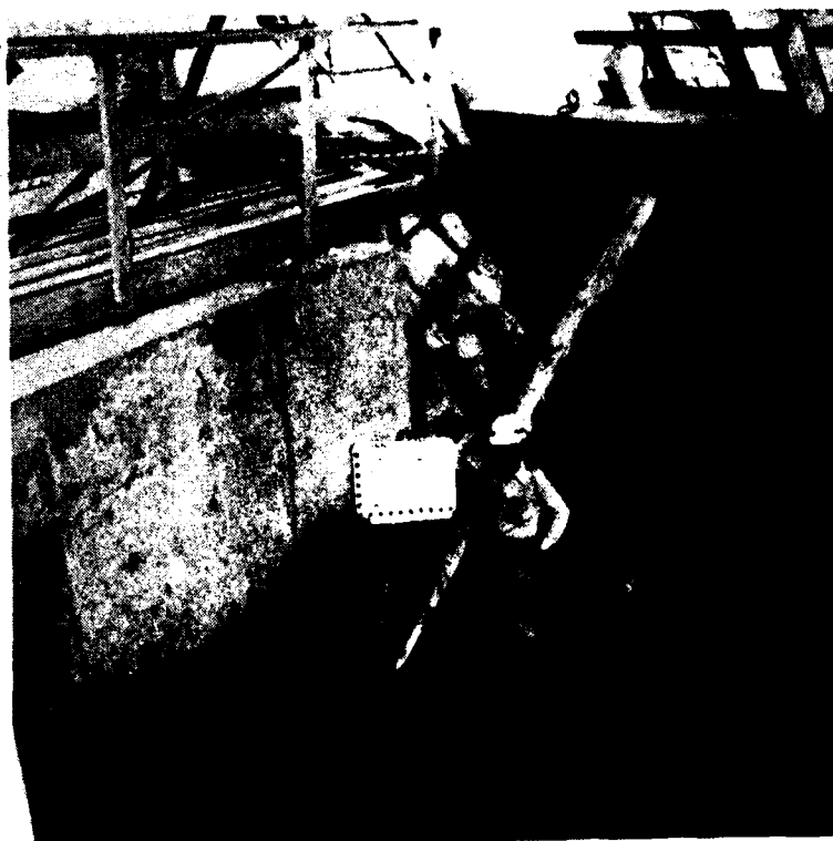
Cutoff wall, final foundation for concrete placement CW 5-6. Station 18+80, Offset downstream, Elevation 600-610 feet. 31 Oct. 1978.
