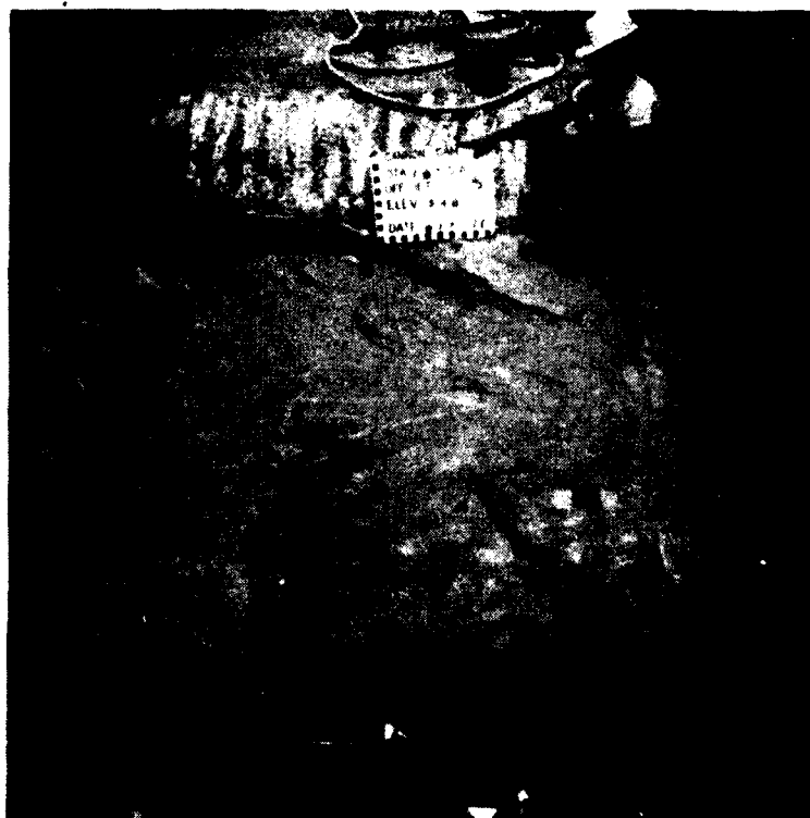
Left abutment cutoff wall final foundation, Hannibal Shale. Station 19+00, Elevation 548 feet. 17 August 1978
