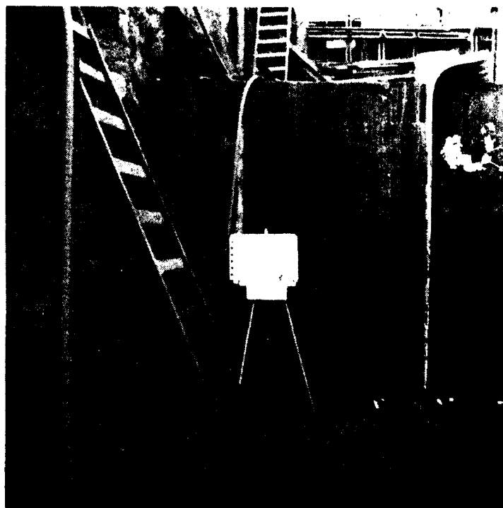
Cutoff wall, final foundation for concrete placement CW 4-4. Station 19+10, Offset upstream, Elevation 580 feet. 12 Oct. 1978.
