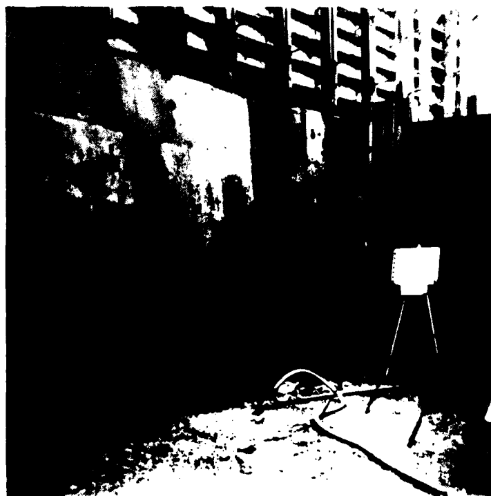
Cutoff wall, final foundation for concrete placement CW 2-5. Station 19+40 Offset downstream, Elevation 590 feet. 11 Oct. 1978.
