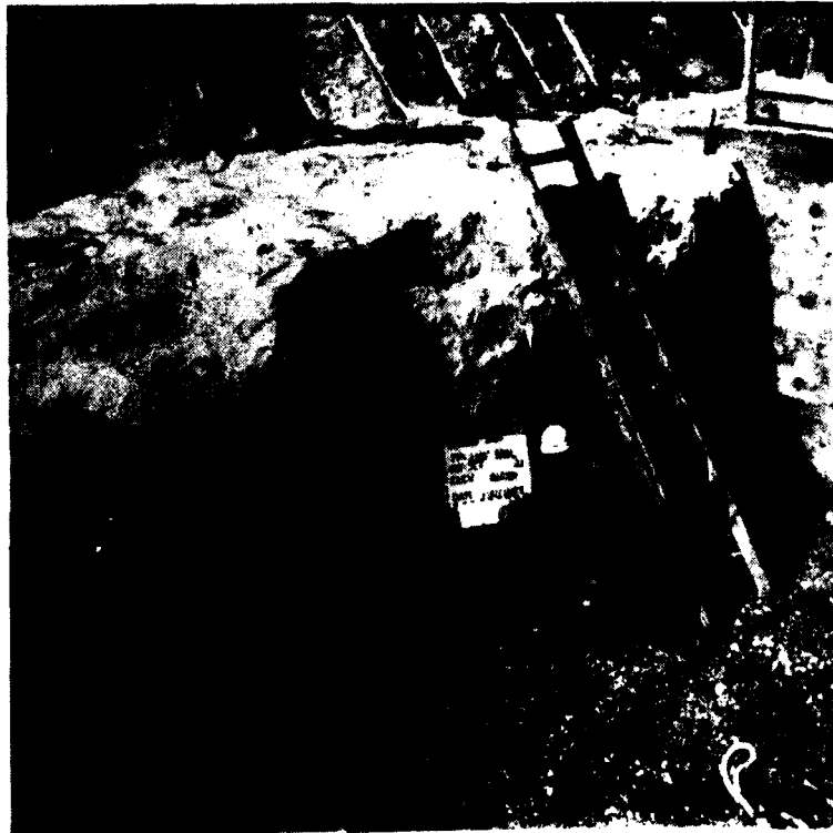
Cutoff wall, final foundation for concrete placement CW 2-6. Station 19+58, Offset upstream, Elevation 600 feet. 16 Oct. 1978.
