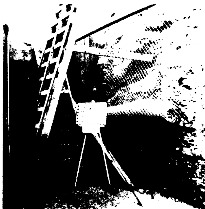
Cutoff wall, final foundation for concrete placement CW 4-4. Station 18+80 Offset upstream, Elevation 580 feet. 12 Oct. 1978.
