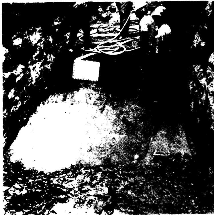
Left abutment cutoff wall final foundation. Hannibal Shale. Station 18+59, Elevation 547.5 feet. 18 August 1978
