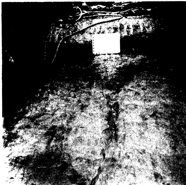
Left abutment cutoff wall final foundation, Hannibal Shale. Station 19+75, Elevation 550 feet. 14 August 1978
