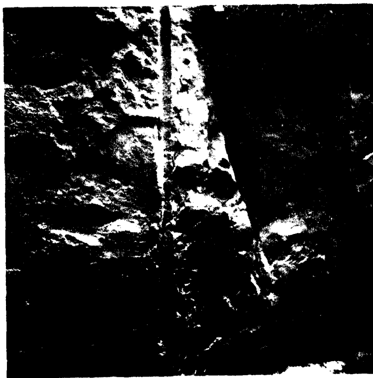
Cutoff wall, final foundation for concrete placement CW 1-1. 18 Sept. 1978
