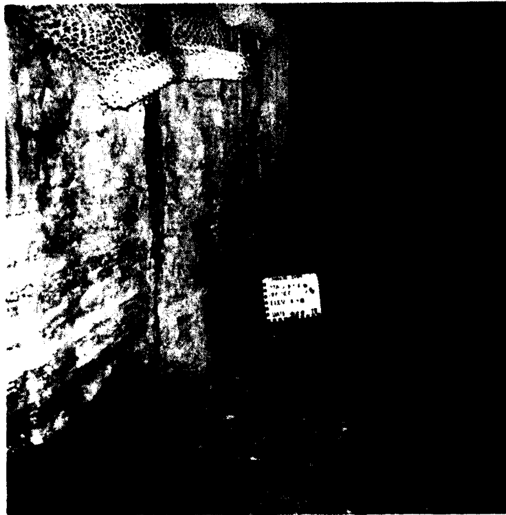
Cutoff wall, final foundation for concrete placement CW 1-3. Station 19+69, Elevation 570 feet. 23 Sept. 1978.
