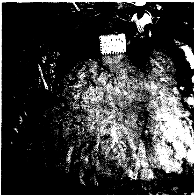
Left abutment cutoff wall final foundation. Hannibal Shale. Station 18+90, Elevation 548 feet. 17 August 1978
