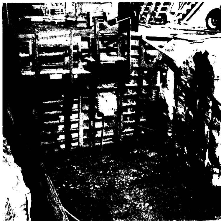
Cutoff wall, final foundation for concrete placement CW 4-6. Station 19+10, Offset downstream, Elevation 600-610 feet. 20 Oct. 1978.
