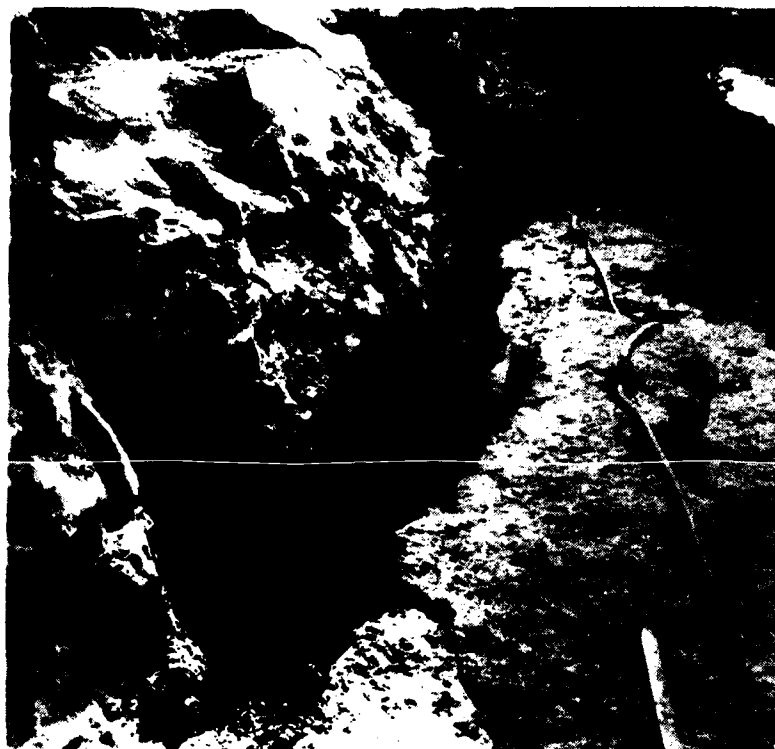
Left abutment downstream ravine, performing foundation preparation on solutioned joint at Station 18+33, Offset 175 feet downstream, Elevation 600 feet. July 1978
