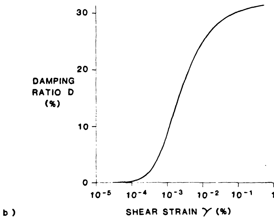
Figure 8. (a) Hysteresis loops for cyclic loading using Ramberg-Osgood 11 relations (b) Variation of damping ratio with strain level.
