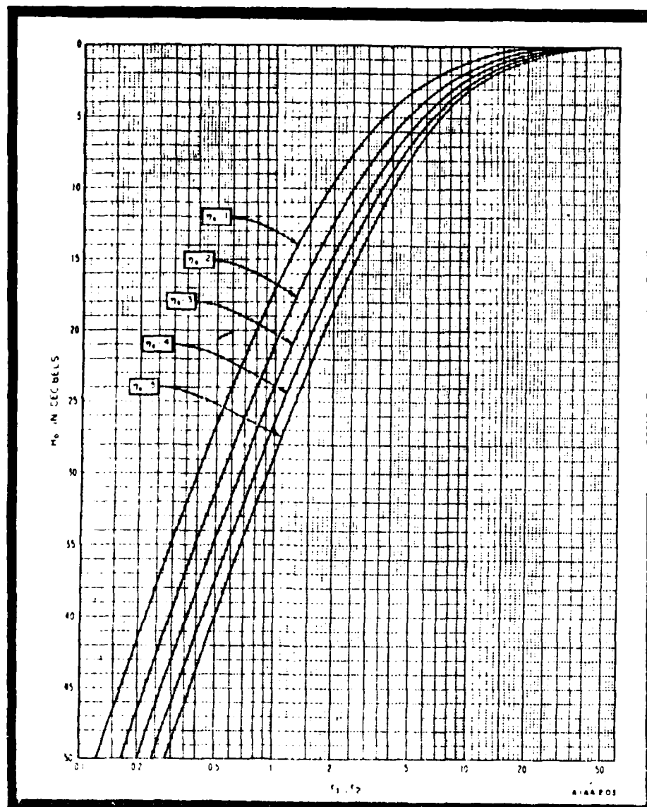
Figure A-6 Frequency Gain Function
