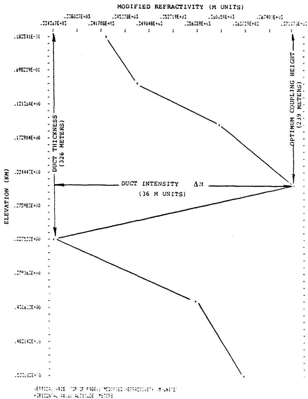
Figure 5-4 M-Profile Plot (Surface Duct)
