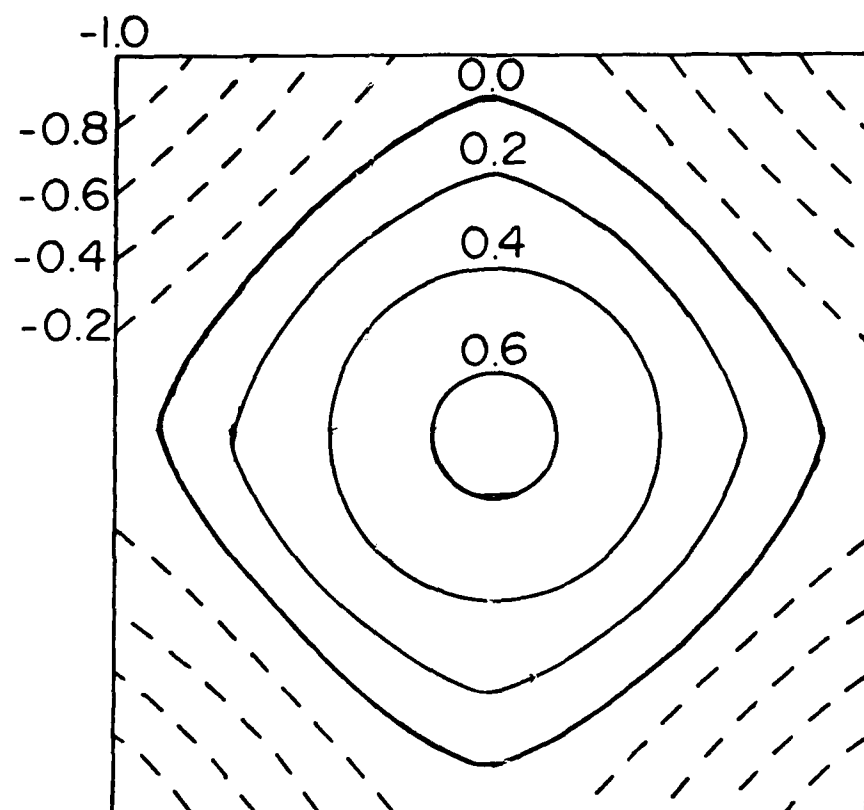
Figure A.3. Flexible Mode 3 - Contour Plots.
