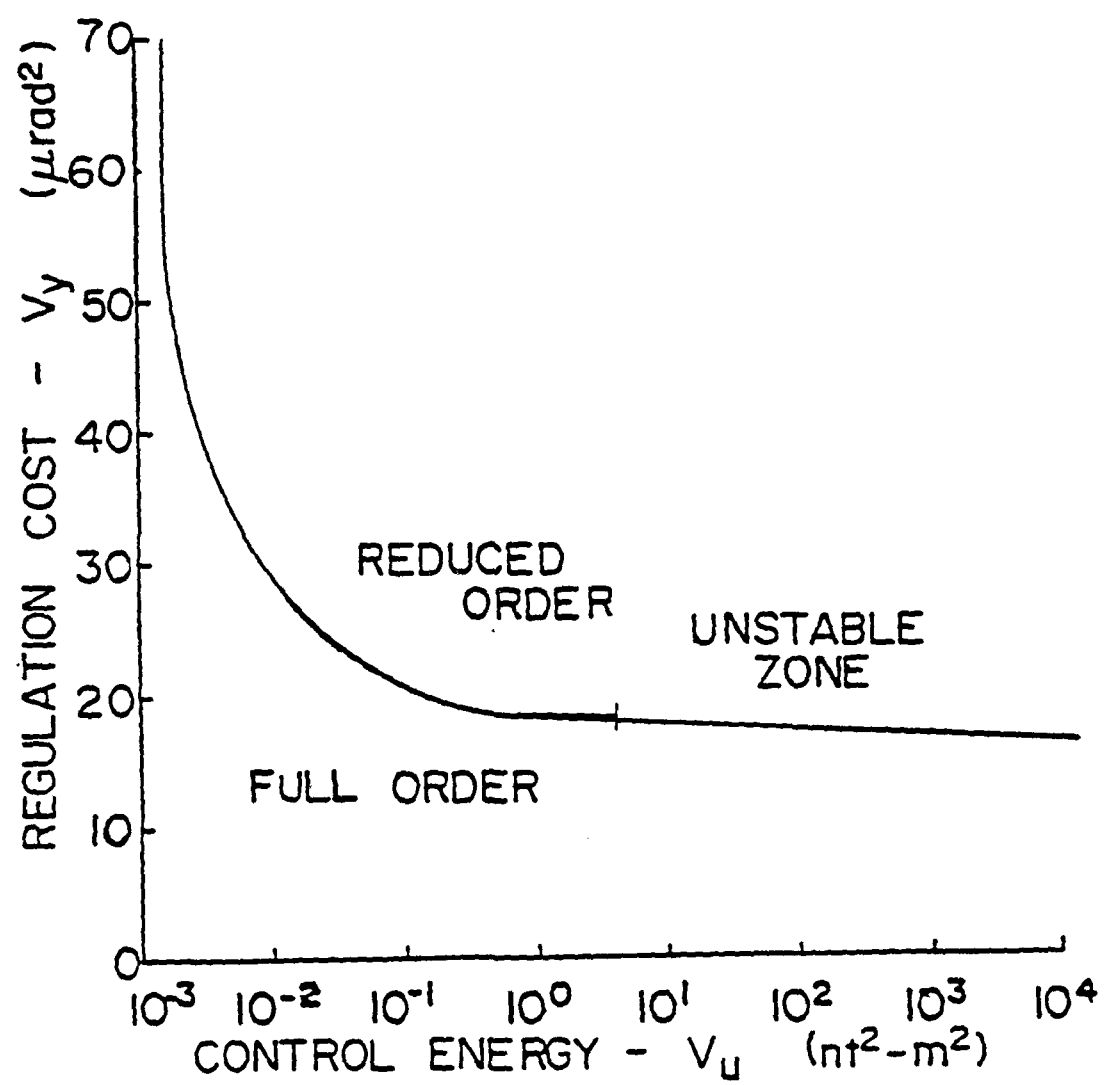
Figure B.7. System Performance Plot ( h = 3.75\text{m} ).
