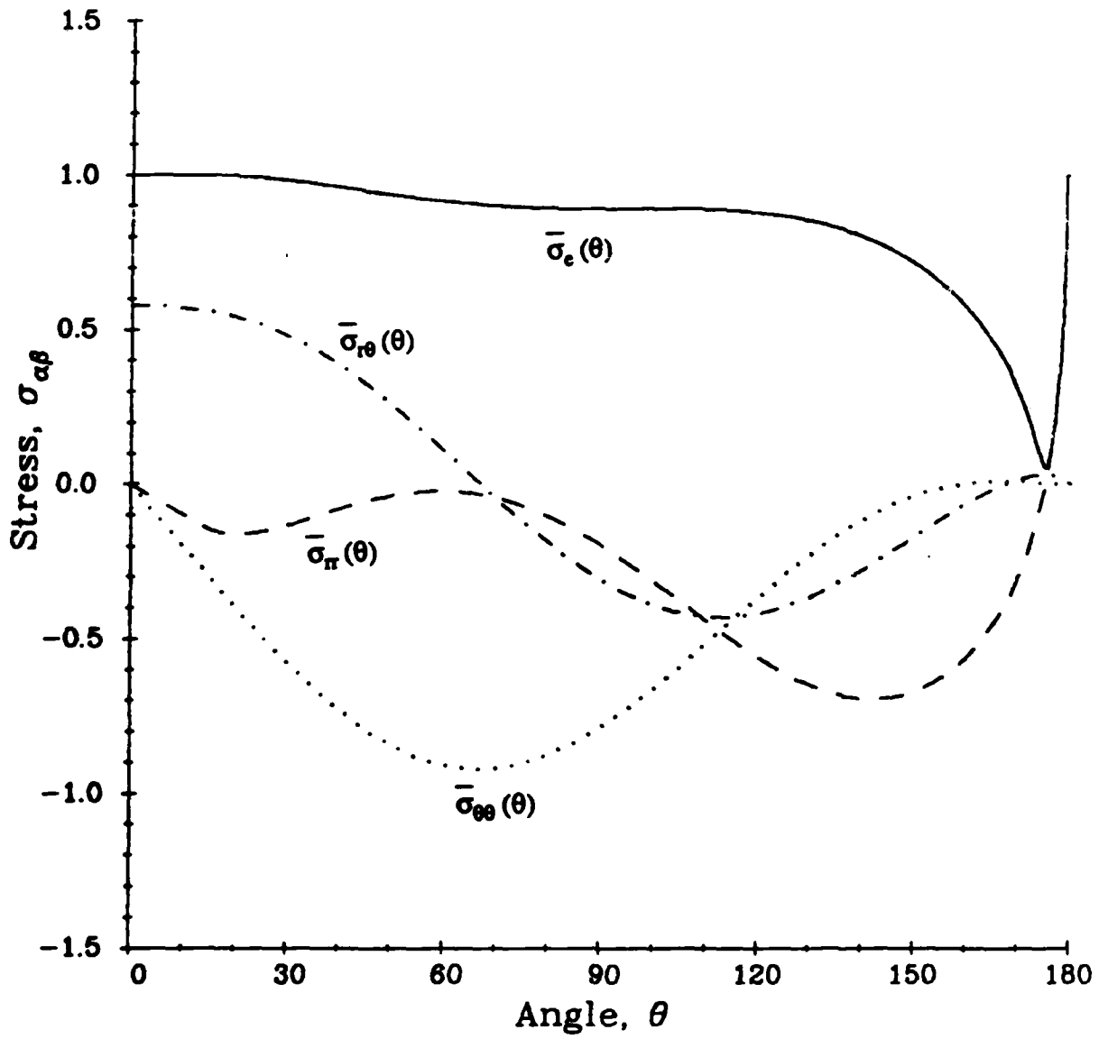
Figure 2. Stress distribution
