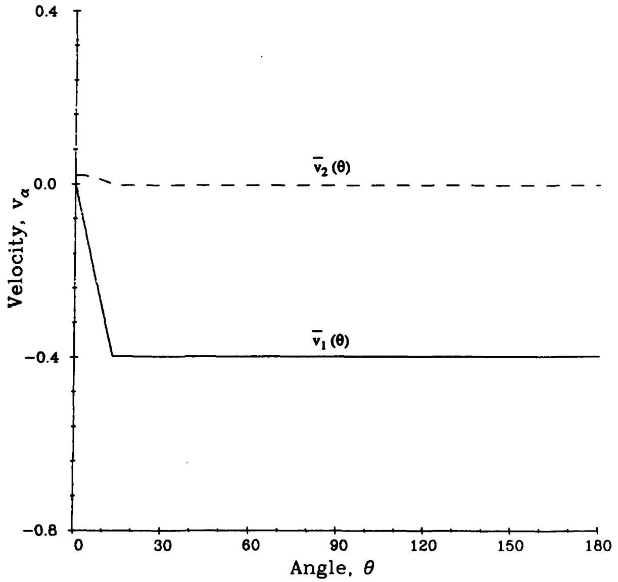
Figure 2. Velocity distribution
