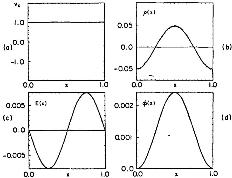
Figure 3. Initial conditions used in Pierce diode simulations for the case \alpha = 0.5W . (a) Electron phase space v versus x , (b) Charge density \rho(x) = e(n_0 - n_e(x)) , (c) resulting electric field E(x) , and (d) potential profile \phi(x) > 0 , indicating "positive initialization".
