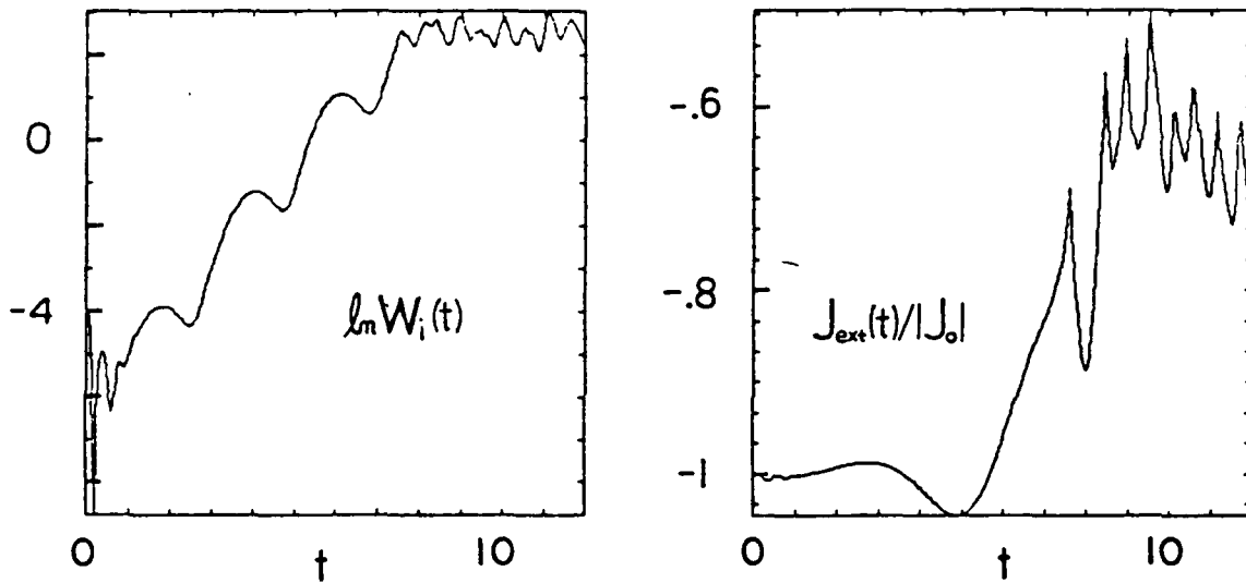
Figure 14. Case: \alpha = 2.5\pi , negative initialization. History plots showing (a) system internal electrostatic energy, \ln W_1(t) , and (b) external circuit current, J_{\text{ext}}(t)/|J_0| .
