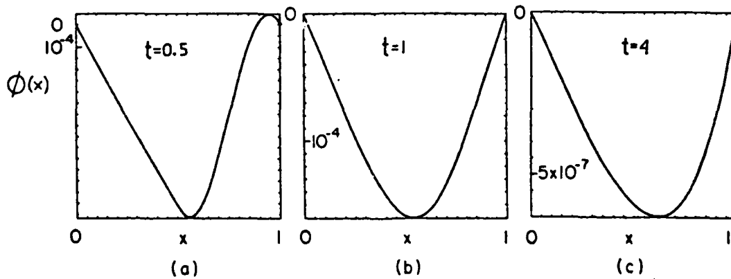
Figure 4. Case: \alpha = 0.5W , positive initialization. Potential profiles \phi(x) at times t = 0.5, 1 , and 4 . Note that the ordinate on each plot is scaled according to the respective maximum values of \phi .
