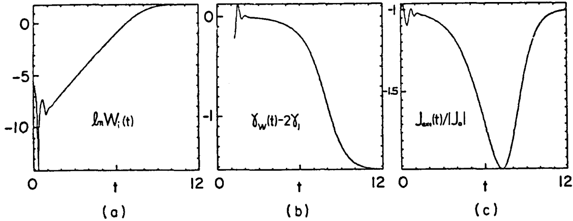
Figure 9. Case: \alpha = 1.5\bar{w} , positive initialization. History plots showing (a) the internal electrostatic energy, \ln W_1(t) , and (b) the difference between the simulation energy rate of change, \delta \dot{W}(t) , and the predicted growth rate in the dominant eigenmode stage, 2\gamma_1 , and (c) the external current, J_{\text{ext}}(t)/|J_0| .
