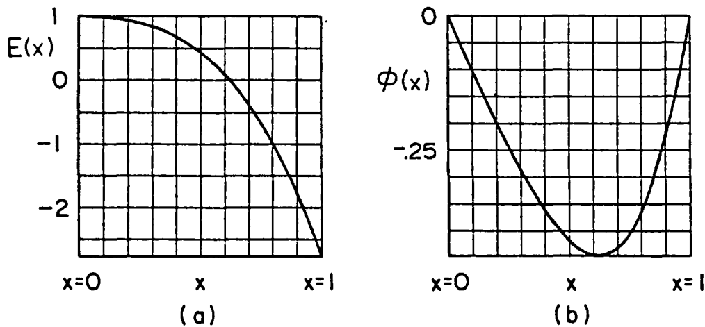
Figure 2. Calculated theoretical profiles of the dominant linear eigenmode for the case \alpha = 0.5\omega . (a) Electric field E(x) , (b) potential \phi(x) .
