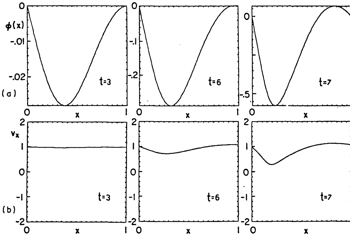
Figure 10. Case: \alpha = 1.5\bar{w} , negative initialization. Early behavior of the Pierce diode. Snapshots show diode evolving from linear into nonlinear stages at t = 3, 6 , and 7 . (a) Potential profiles \phi(x) , and (b) the corresponding electron phase spaces.
