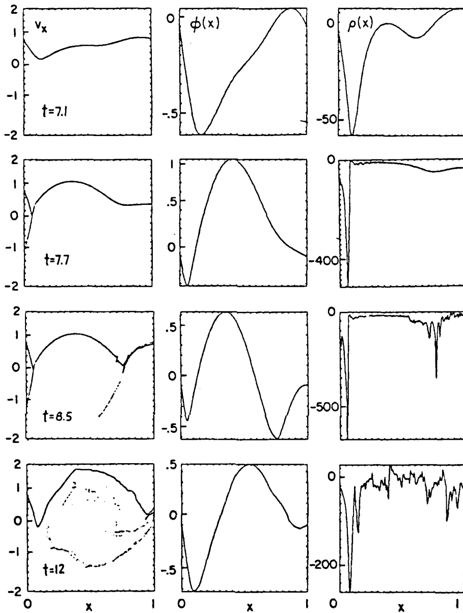
Figure 16. Case: \alpha = 2.5v , positive initialization. Nonlinear diode behavior from shortly after dominant eigenmode stage, t = 7.1 , to effective final state at t=12 . Electron phase space, potential profiles, and spatial charge density showing virtual cathode.
